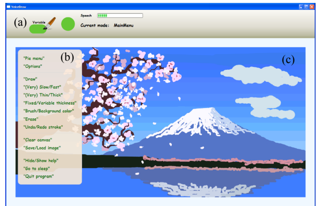
Figure 1: A screenshot of the VoiceDraw application 1 showing (a) the status bar, (b) help overlay, and (c) canvas area. The first author created this painting using only his voice in about 2.5 hours.
