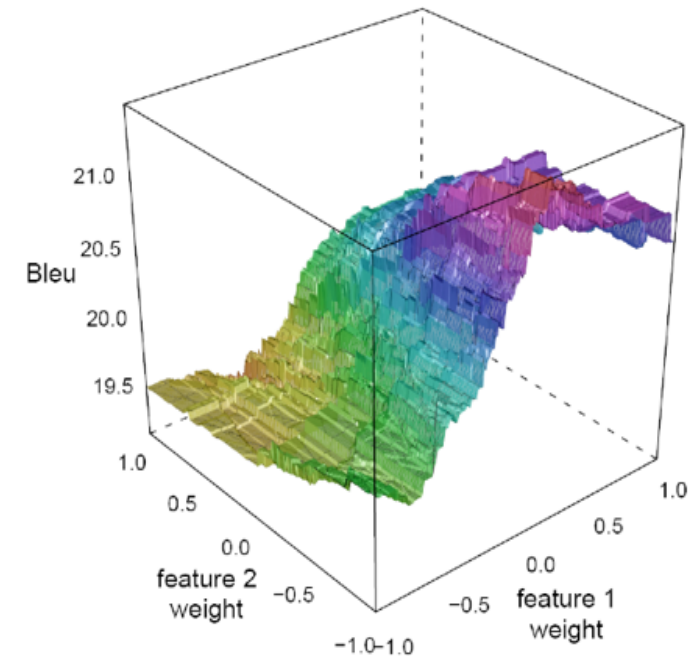
\gamma = \infty
