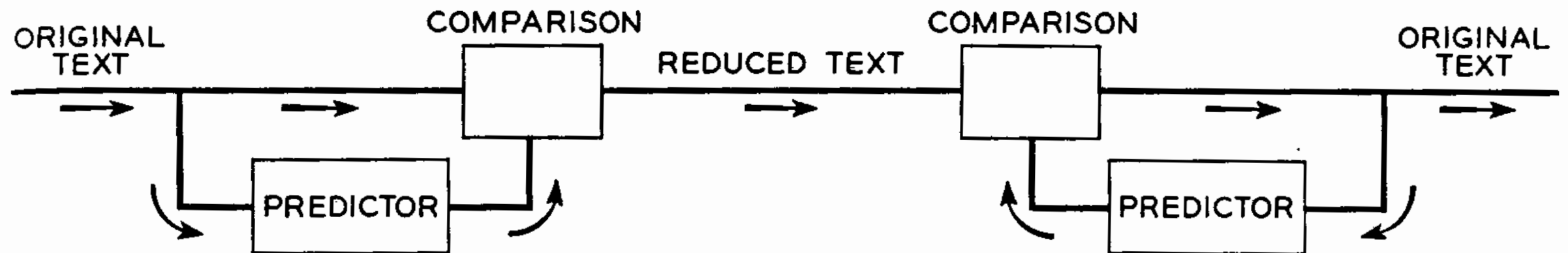
Fig. 2—Communication system using reduced text.
