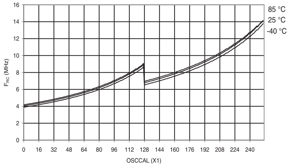
Figure 28-236. ATmega644A: Calibrated 8 MHz RC Oscillator vs. OSCCAL Value
