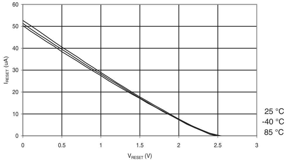
Figure 28-265. ATmega644PA: Reset Pull-up Resistor Current vs. Reset Pin Voltage ( V_{CC} = 5V ).
