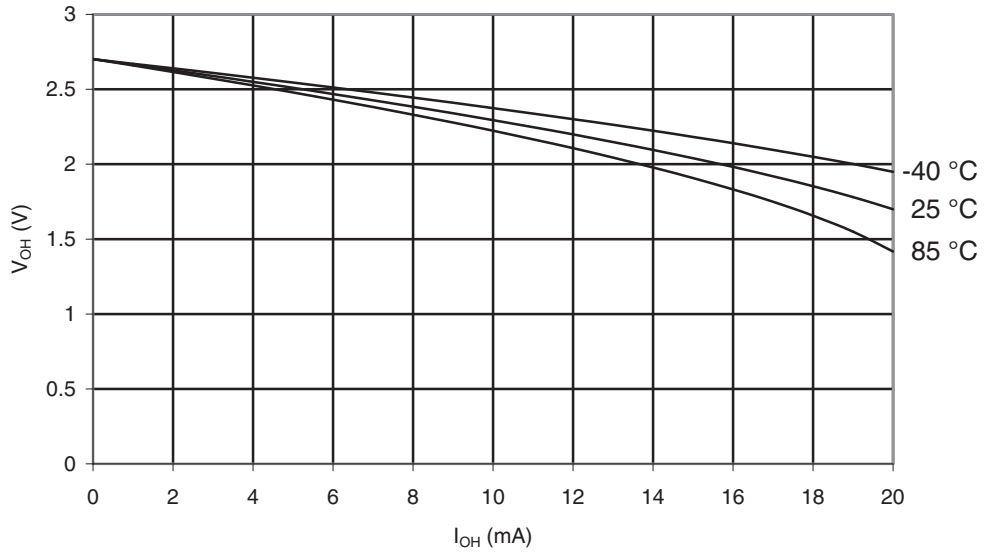
Figure 28-368. ATmega1284P: I/O Pin Output Voltage vs. Source Current ( V_{CC} = 2.7V )
