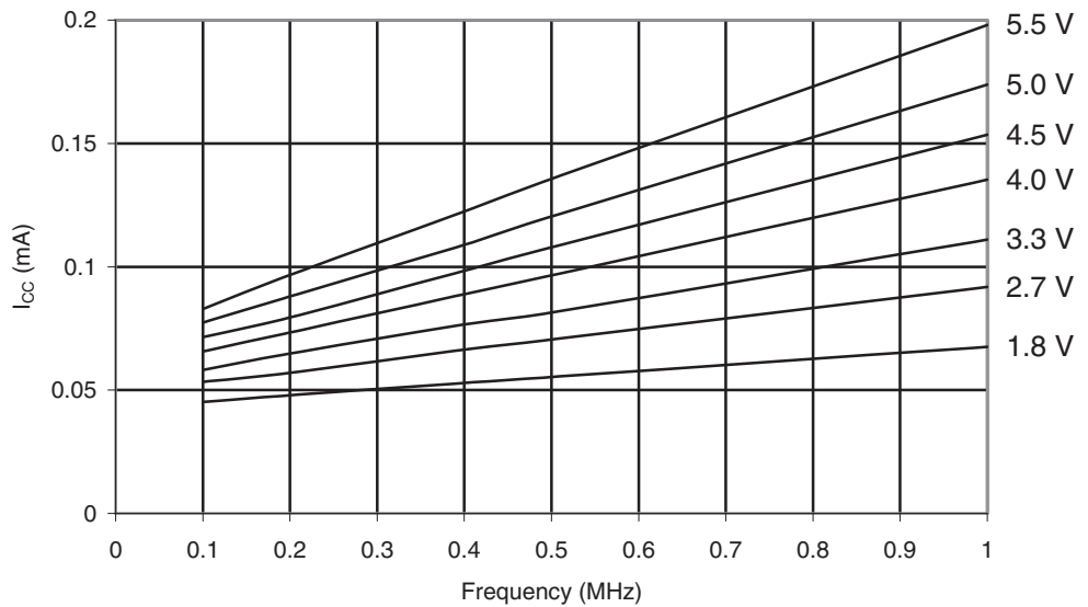
Figure 28-55. ATmega164PA: Idle Supply Current vs. V_{CC} (0.1 - 1.0 MHz).
