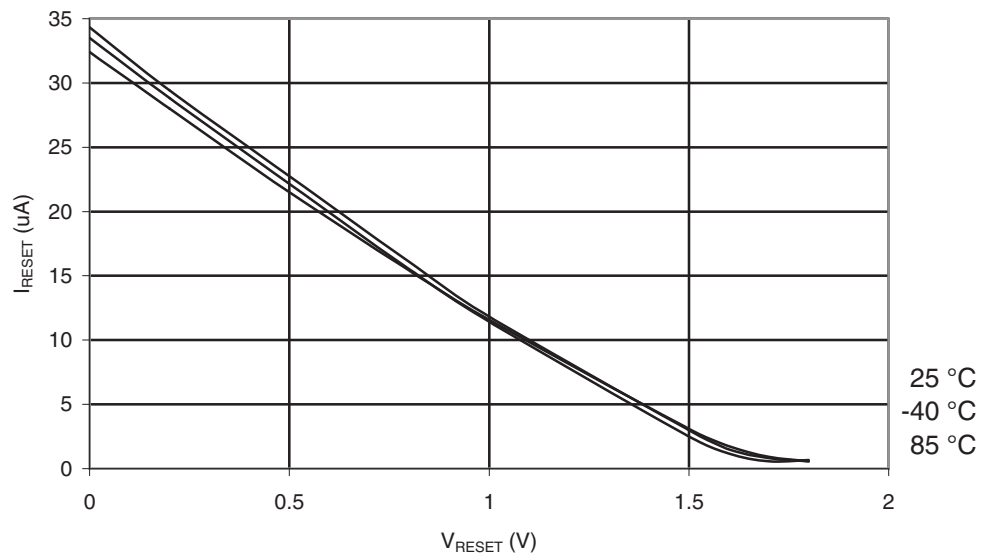
Figure 28-67. ATmega164PA: Reset Pull-up Resistor Current vs. Reset Pin Voltage ( V_{CC} = 1.8V ).
