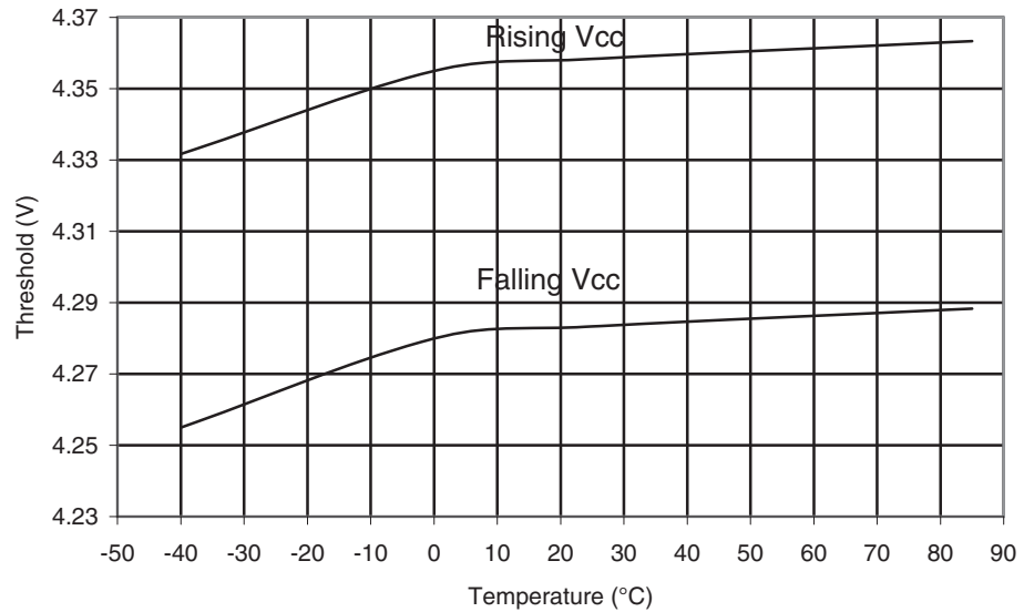
Figure 28-376. ATmega1284P: BOD Threshold vs. Temperature ( V_{BOT} = 4.3V )
