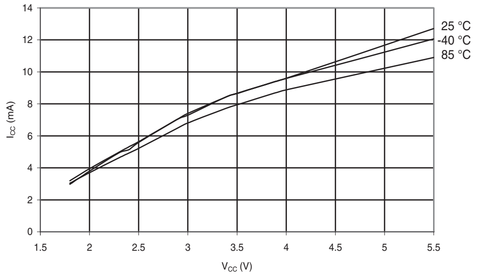
Figure 28-143. ATmega324A: Programming Current vs. V_{CC}
