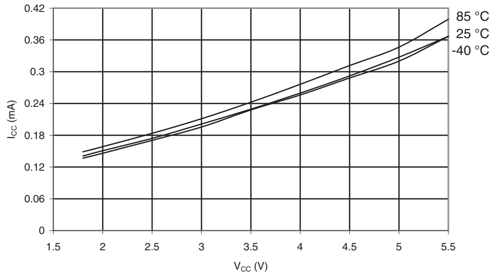
Figure 28-303. ATmega1284: Idle Supply Current vs. V_{CC} (Internal RC Oscillator, 1 MHz)
