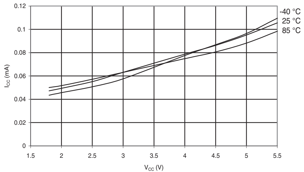
Figure 28-108. ATmega324A: Idle Supply Current vs. V_{CC} (Internal RC Oscillator, 128 kHz).
