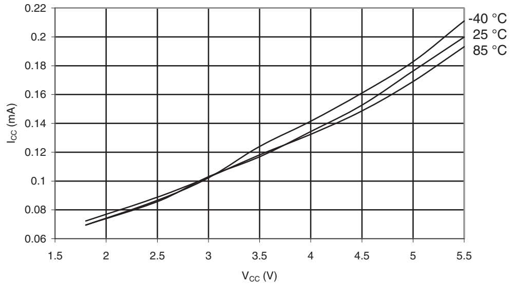
Figure 28-201. ATmega644A: Active Supply Current vs. V_{CC} (Internal RC Oscillator, 128 kHz).
