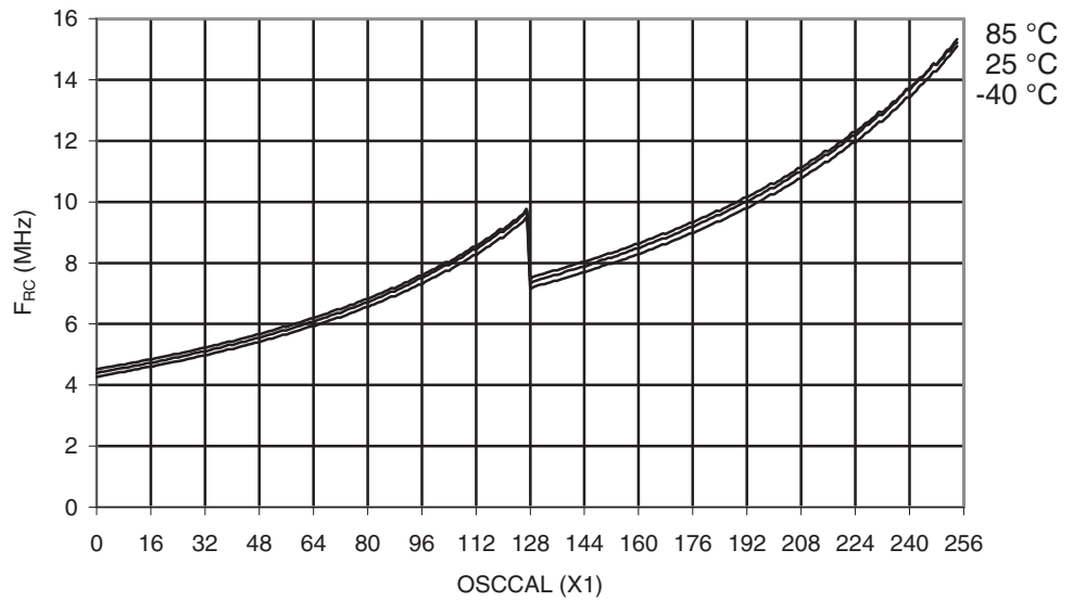
Figure 28-40. ATmega164A: Calibrated 8 MHz RC Oscillator vs. OSCCAL Value
