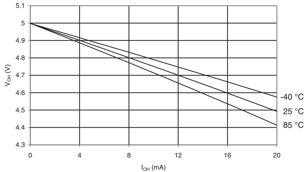
Figure 28-24. ATmega164A: I/O Pin Output Voltage vs. Source Current ( V_{CC} = 5V ).
