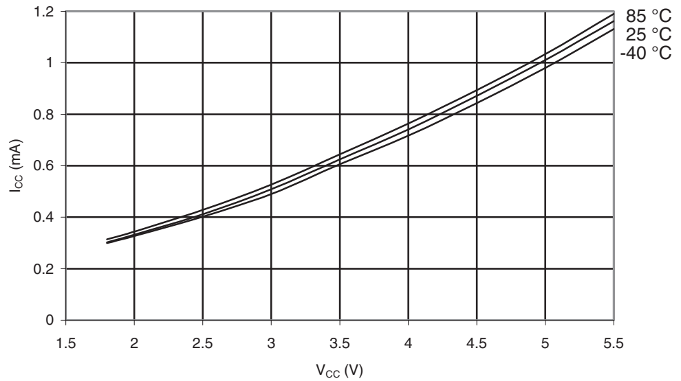
Figure 28-4. ATmega164A: Active Supply Current vs. V_{CC} (Internal RC Oscillator, 1 MHz).
