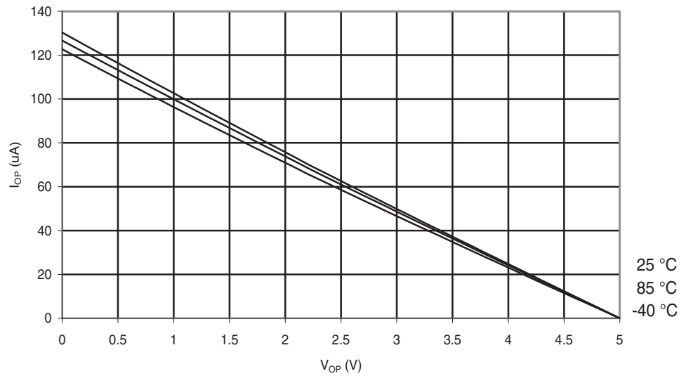
Figure 28-213. ATmega644A: I/O Pin Pull-up Resistor Current vs. Input Voltage ( V_{CC} = 5V ).
