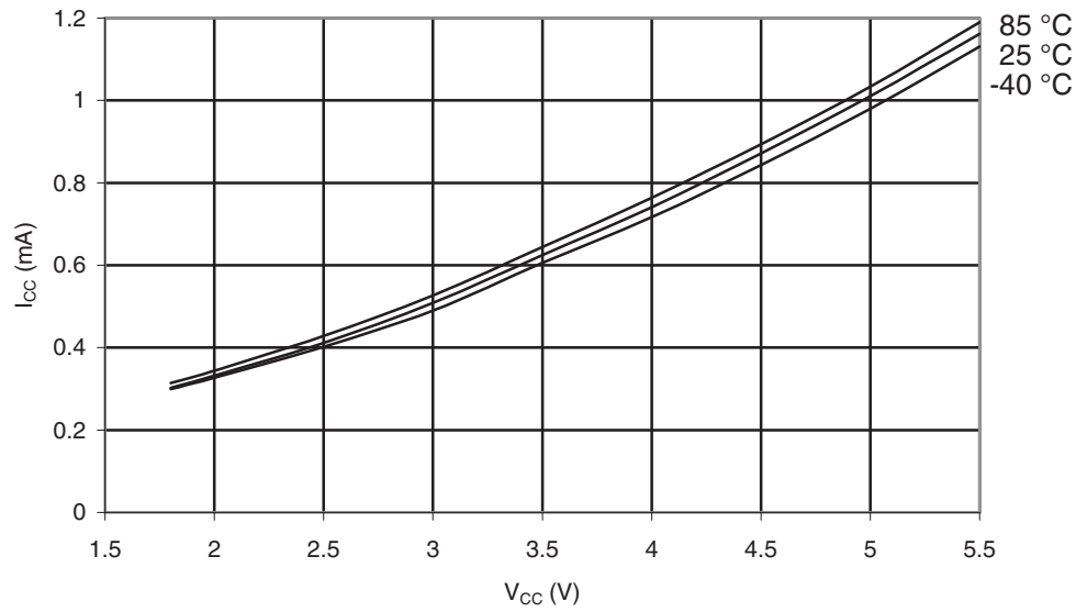
Figure 28-53. ATmega164PA: Active Supply Current vs. V_{CC} (Internal RC Oscillator, 1 MHz).
