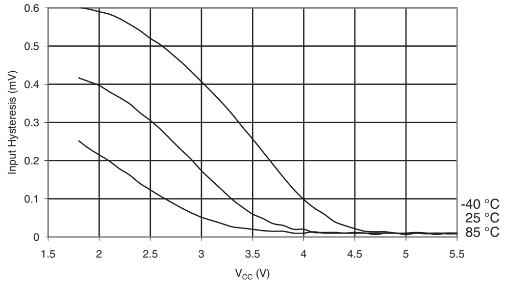
Figure 28-375. ATmega1284P: Reset Pin Input Hysteresis vs. V_{CC}
