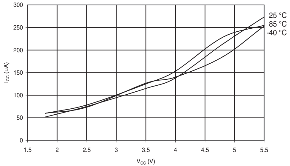
Figure 28-188. ATmega324PA: ADC Current vs. V_{CC} (AREF = AV_{CC} )
