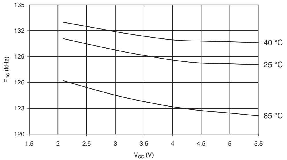
Figure 28-86. ATmega164PA: Watchdog Oscillator Frequency vs. V_{CC}
