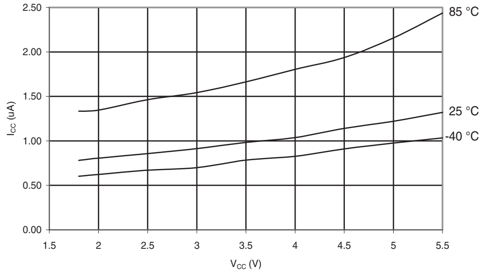
Figure 28-111. ATmega324A: Power-save Supply Current vs. V_{CC} (Watchdog Timer Disabled and 32 kHz Crystal Oscillator Running).
