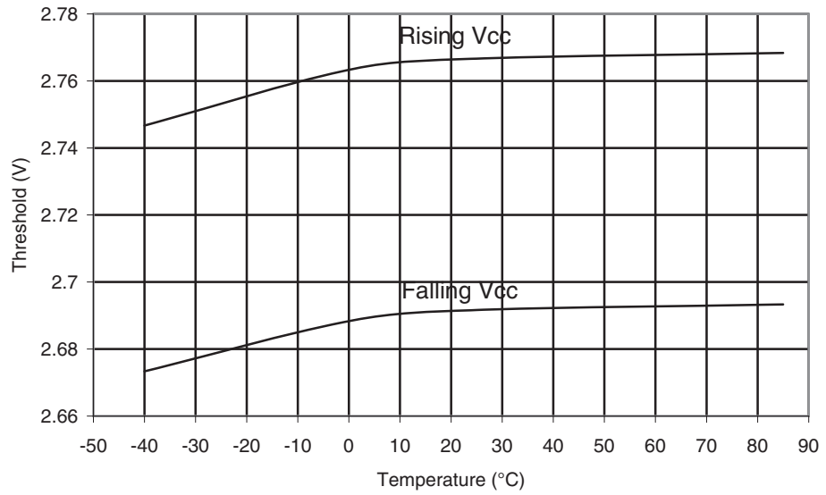
Figure 28-327. ATmega1284: BOD Threshold vs. Temperature ( V_{BOT} = 2.7V )
