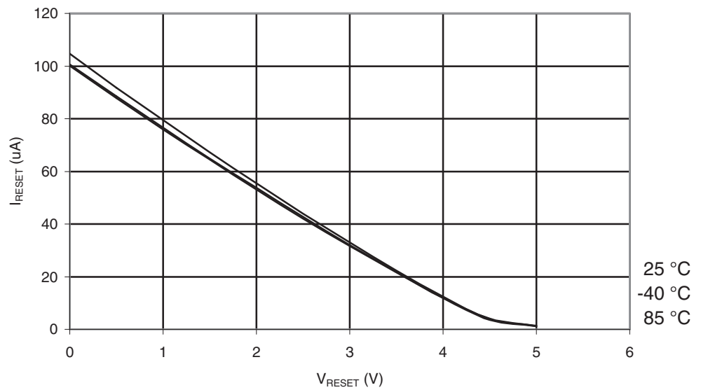
Figure 28-20. ATmega164A: Reset Pull-up Resistor Current vs. Reset Pin Voltage ( V_{CC} = 5V ).
