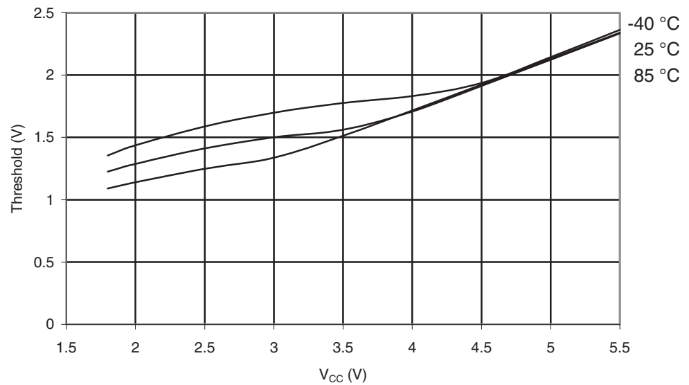
Figure 28-77. ATmega164PA: Reset Pin Input Threshold vs. V_{CC} ( V_{IH} , I/O Pin Read as '1').
