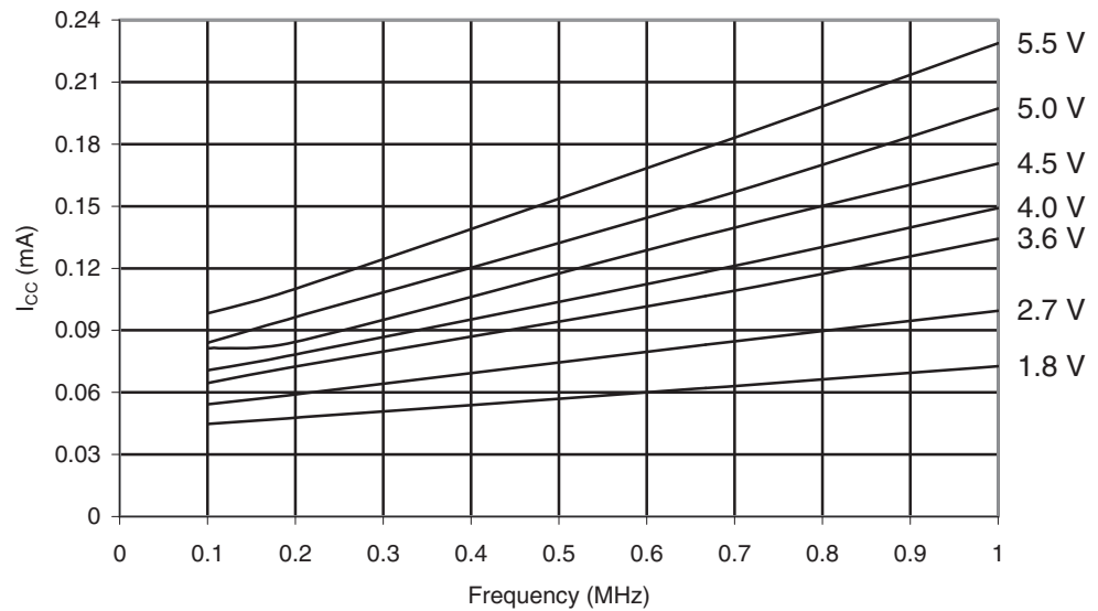
Figure 28-300. ATmega1284: Idle Supply Current vs. Low Frequency (0.1 - 1.0 MHz)
