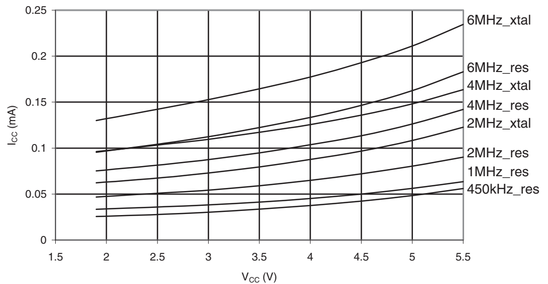
Figure 28-358. ATmega1284P: Standby Supply Current vs. V_{CC} (Watchdog Timer Disabled)
