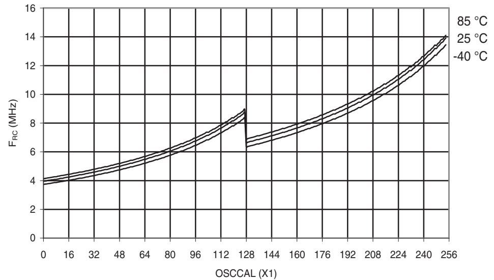
Figure 28-187. ATmega324PA: Calibrated 8 MHz RC Oscillator vs. OSCCAL Value
