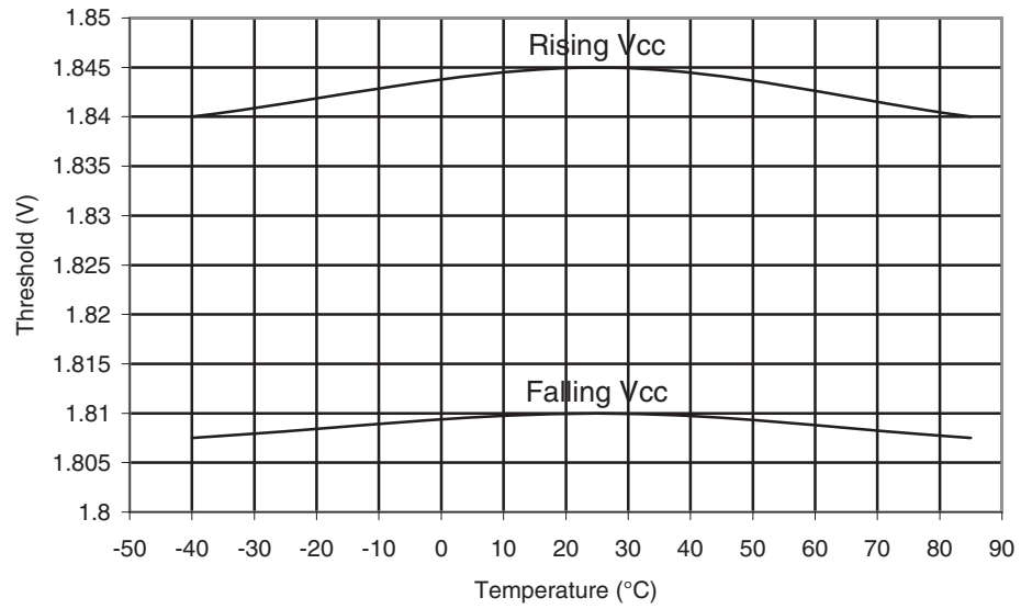
Figure 28-82. ATmega164PA: BOD Threshold vs. Temperature ( V_{BOT} = 1.8V )
