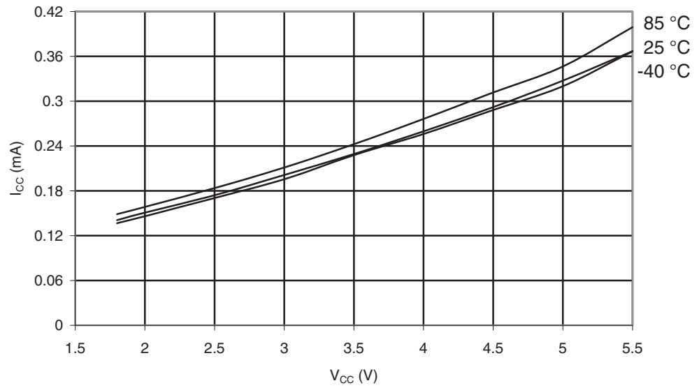
Figure 28-353. ATmega1284P: Idle Supply Current vs. V_{CC} (Internal RC Oscillator, 1 MHz)
