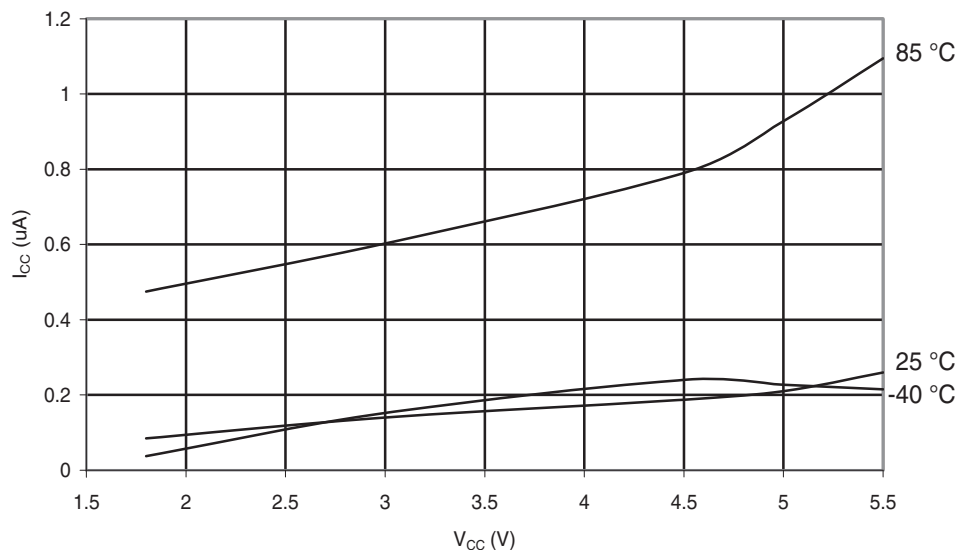
Figure 28-109. ATmega324A: Power-down Supply Current vs. V_{CC} (Watchdog Timer Disabled).
