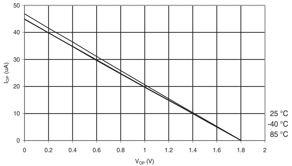
Figure 28-113. ATmega324A: I/O Pin Pull-up Resistor Current vs. Input Voltage ( V_{CC} = 1.8V ).
