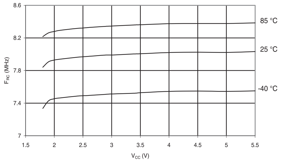
Figure 28-185. ATmega324PA: Calibrated 8 MHz RC Oscillator vs. V_{CC}
