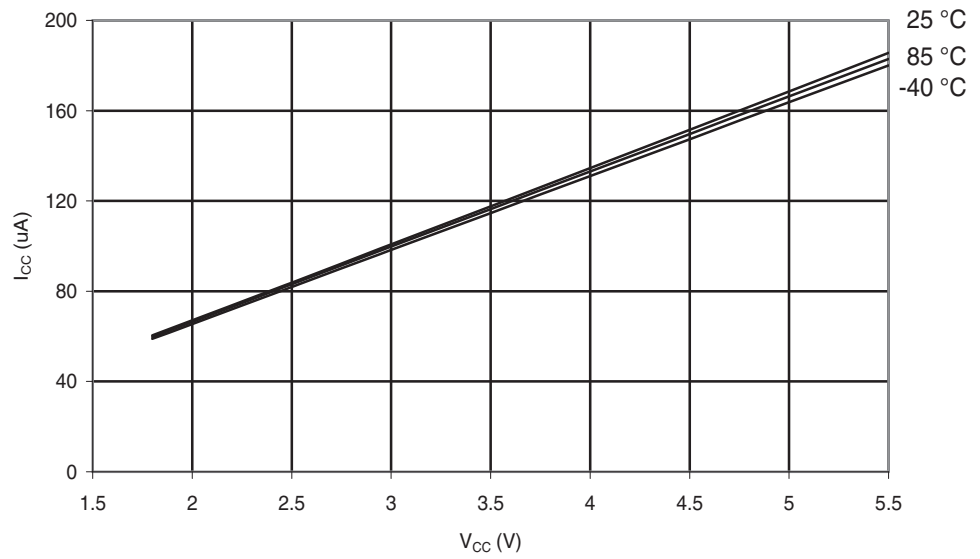
Figure 28-141. ATmega324A: AREF External Reference Current vs. V_{CC}
