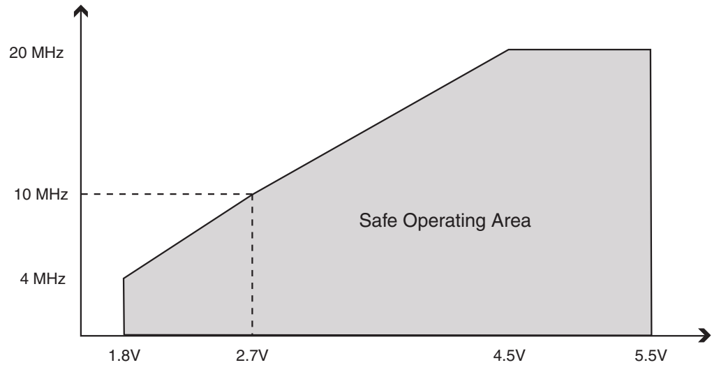
Figure 27-1. Maximum Frequency vs. V_{CC} , ATmega164A/164PA/324A/324PA/644A/644PA/1284/1284P
