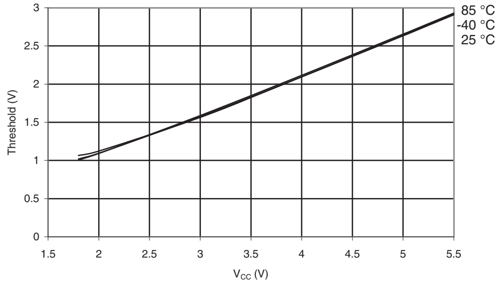
Figure 28-222. ATmega644A: I/O Pin Input Threshold vs. V_{CC} ( V_{IL} , I/O Pin Read as '0').
