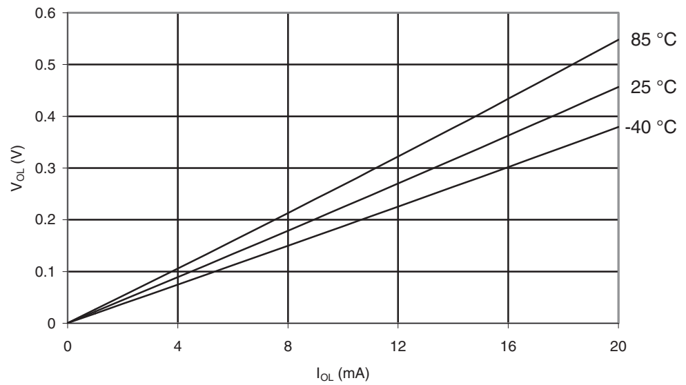
Figure 28-71. ATmega164PA: I/O Pin Output Voltage vs. Sink Current ( V_{CC} = 5V ).
