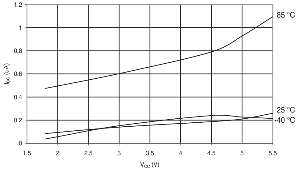
Figure 28-158. ATmega324PA: Power-down Supply Current vs. V_{CC} (Watchdog Timer Disabled).
