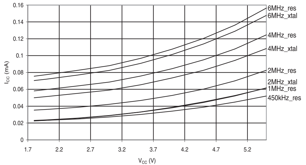
Figure 28-210. ATmega644A: Standby Supply Current vs. V_{CC} (Watchdog Timer Disabled)
