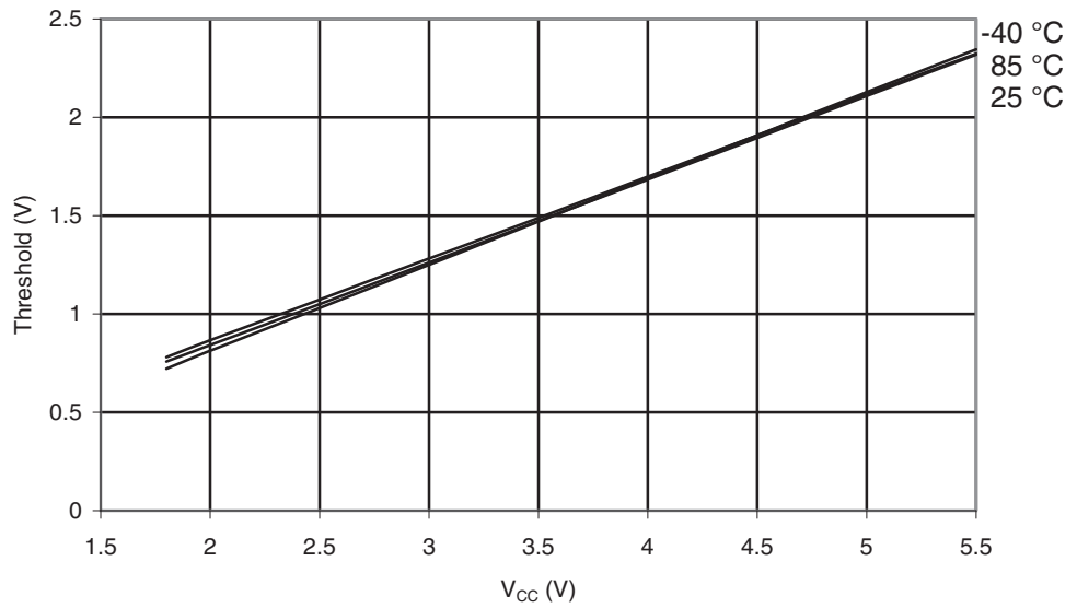
Figure 28-374. ATmega1284P: Reset Pin Input Threshold vs. V_{CC} ( V_{IL} , I/O Pin Read as '0')
