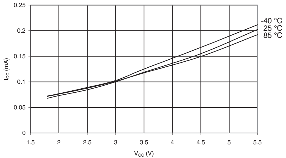
Figure 28-5. ATmega164A: Active Supply Current vs. V_{CC} (Internal RC Oscillator, 128 kHz).
