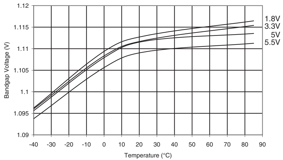
Figure 28-330. ATmega1284: Bandgap Voltage vs. Temperature
