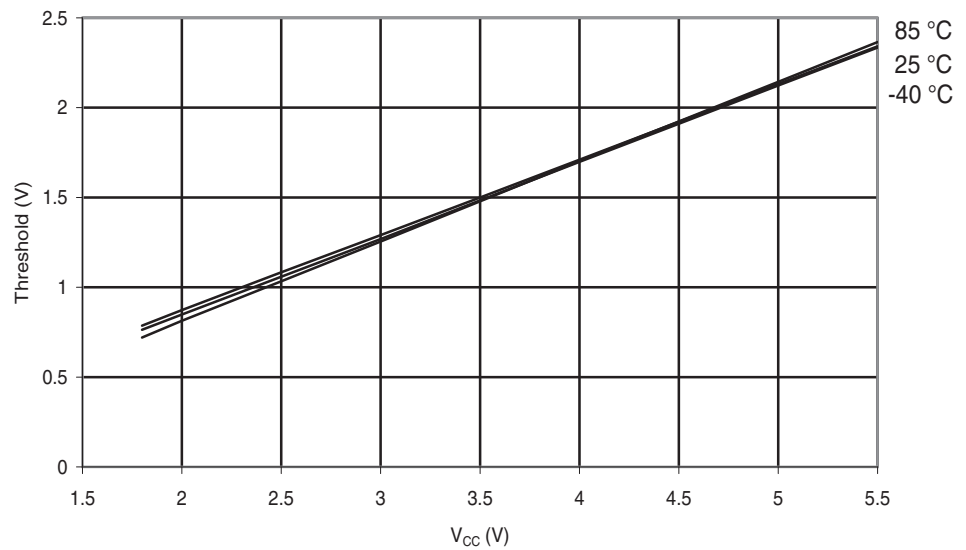
Figure 28-271. ATmega644PA: I/O Pin Input Threshold vs. V_{CC} ( V_{IL} , I/O Pin Read as '0').
