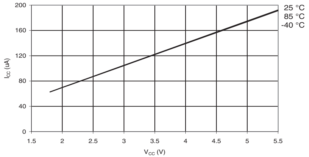
Figure 28-43. ATmega164A: AREF External Reference Current vs. V_{CC}
