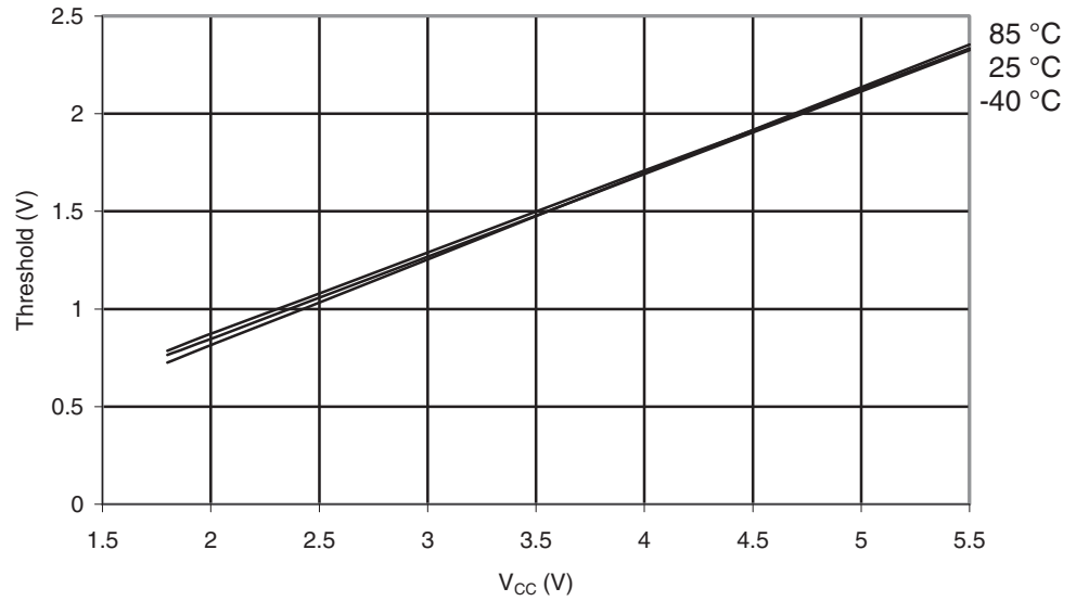
Figure 28-78. ATmega164PA: Reset Pin Input Threshold vs. V_{CC} ( V_{IL} , I/O Pin Read as '0').
