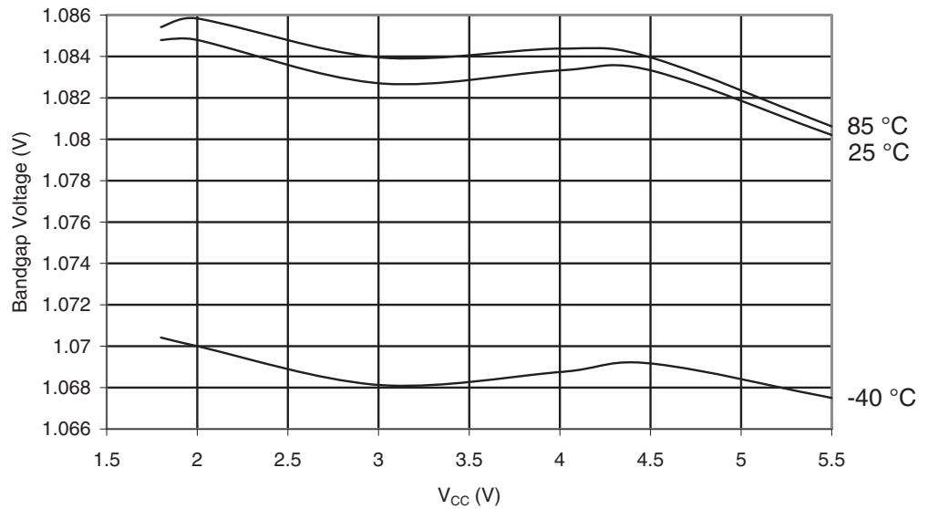
Figure 28-279. ATmega644PA: Calibrated Bandgap Voltage vs. V_{CC}
