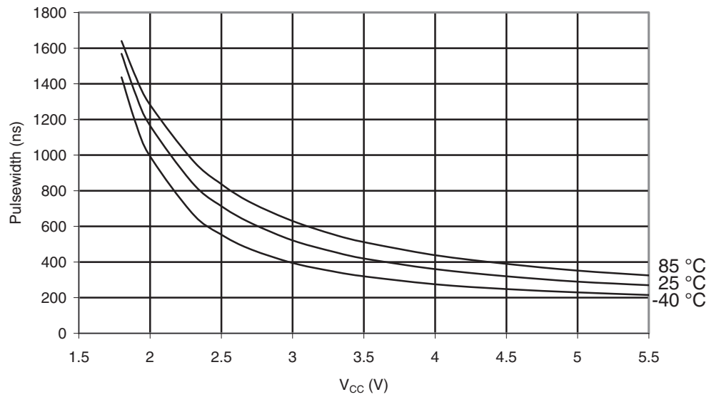
Figure 28-344. ATmega1284: Minimum Reset Pulsewidth vs. V_{CC}
