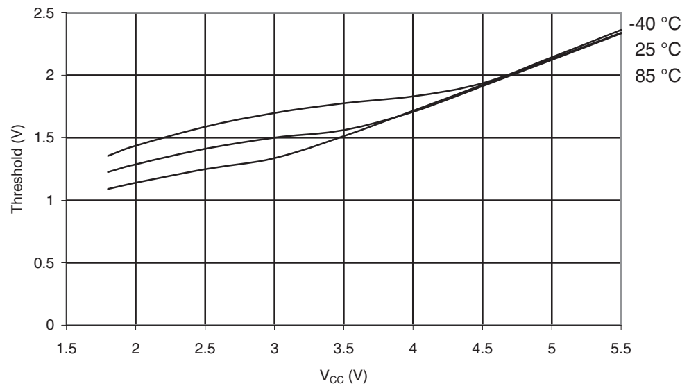
Figure 28-28. ATmega164A: Reset Pin Input Threshold vs. V_{CC} ( V_{IH} , I/O Pin Read as '1').
