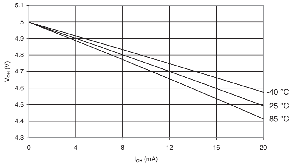
Figure 28-73. ATmega164PA: I/O Pin Output Voltage vs. Source Current ( V_{CC} = 5V ).
