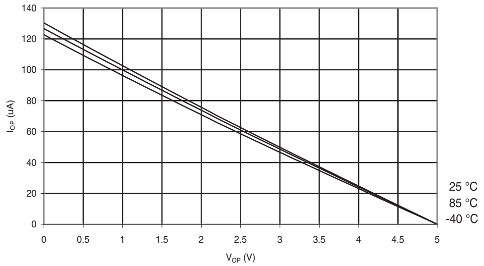
Figure 28-262. ATmega644PA: I/O Pin Pull-up Resistor Current vs. Input Voltage ( V_{CC} = 5V ).
