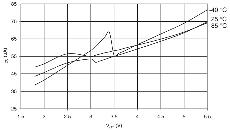
Figure 28-388. ATmega1284P: AREF External Reference Current vs. V_{CC}
