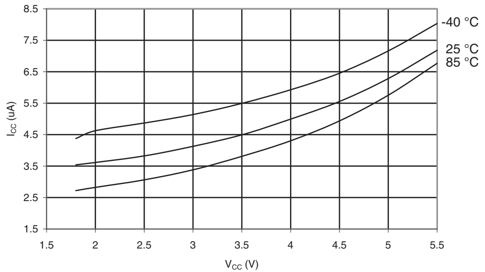
Figure 28-341. ATmega1284: Watchdog Timer Current vs. V_{CC}
