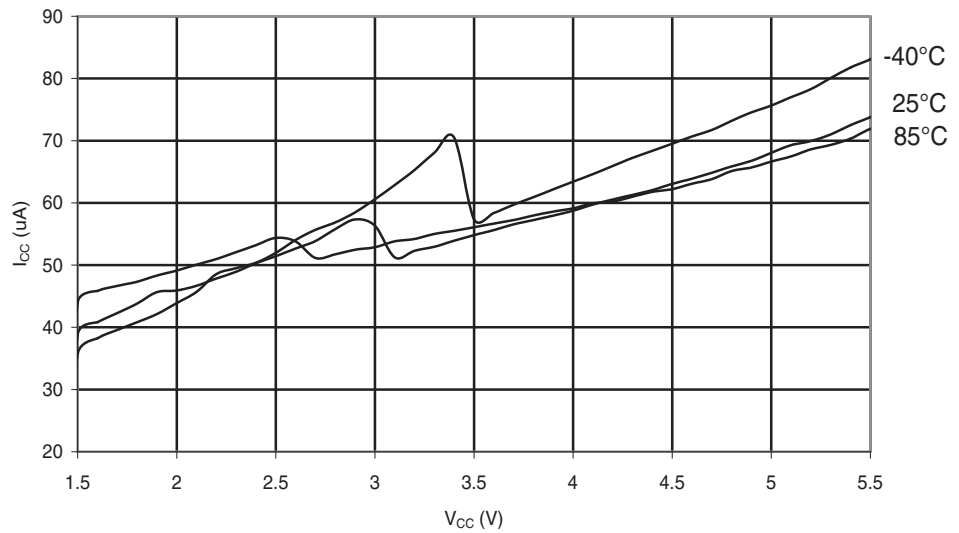
Figure 28-287. ATmega644PA: Analog Comparator Current vs. V_{CC}
