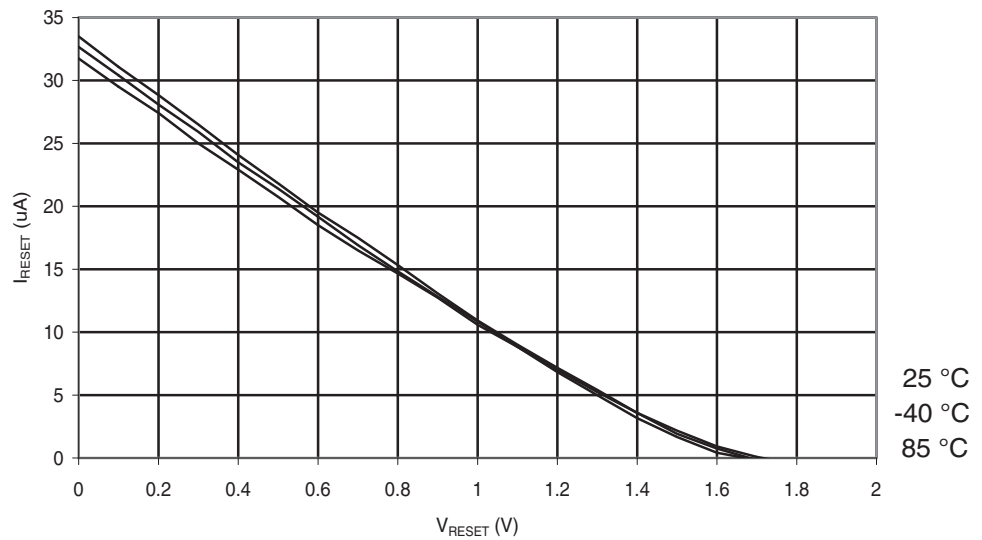
Figure 28-214. ATmega644A: Reset Pull-up Resistor Current vs. Reset Pin Voltage ( V_{CC} = 1.8V ).
