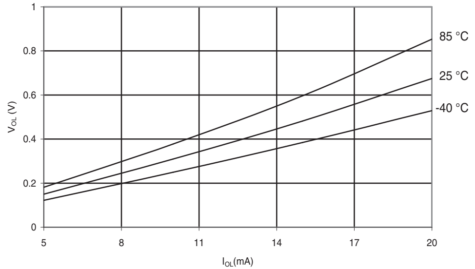
Figure 28-168. ATmega324PA: I/O Pin Output Voltage vs. Sink Current ( V_{CC} = 3V ).
