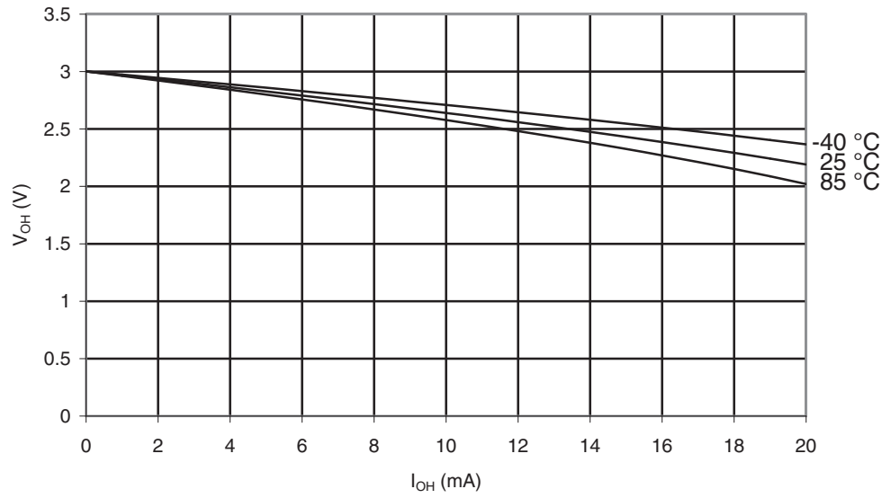
Figure 28-369. ATmega1284P: I/O Pin Output Voltage vs. Source Current ( V_{CC} = 3V )
