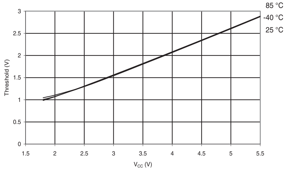
Figure 28-123. ATmega324A: I/O Pin Input Threshold vs. V_{CC} ( V_{IH} , I/O Pin Read as '1').
