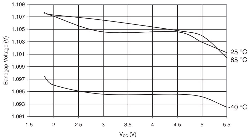
Figure 28-34. ATmega164A: Calibrated Bandgap Voltage vs. V_{CC}
