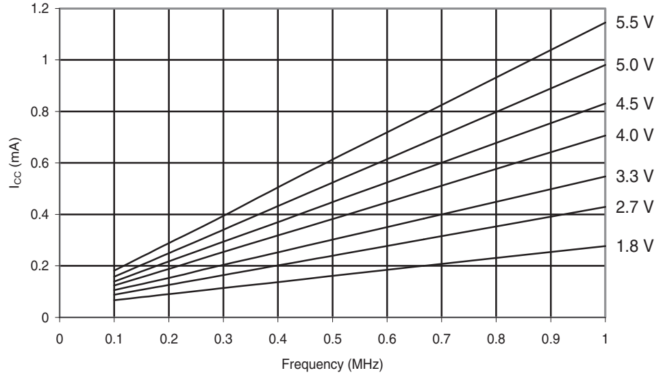
Figure 28-99. ATmega324A: Active Supply Current vs. Low Frequency (0.1 - 1.0 MHz).
