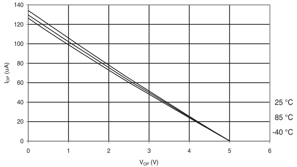
Figure 28-115. ATmega324A: I/O Pin Pull-up Resistor Current vs. Input Voltage ( V_{CC} = 5V ).
