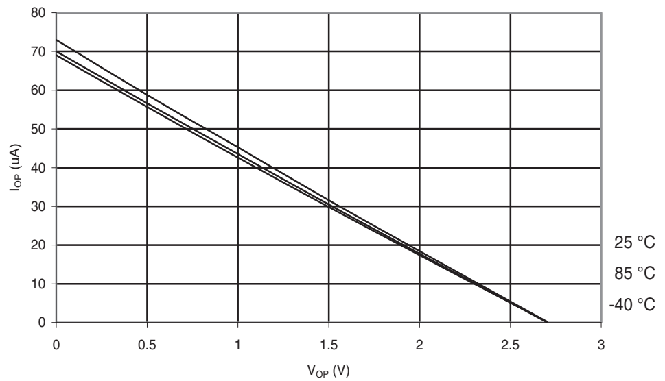
Figure 28-114. ATmega324A: I/O Pin Pull-up Resistor Current vs. Input Voltage ( V_{CC} = 2.7V ).
