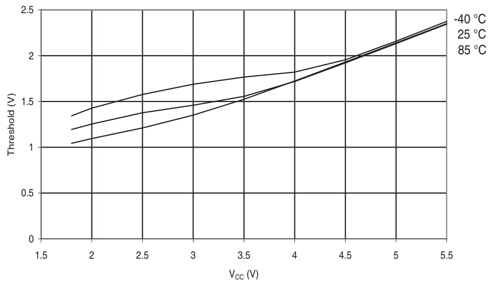
Figure 28-224. ATmega644A: Reset Pin Input Threshold vs. V_{CC} ( V_{IH} , I/O Pin Read as '1').
