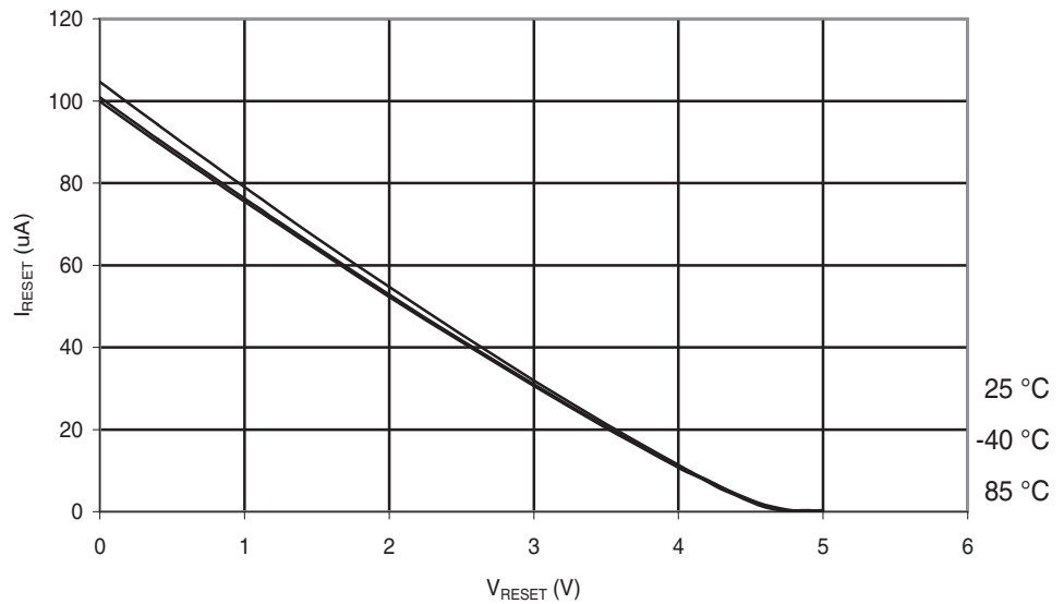
Figure 28-118. ATmega324A: Reset Pull-up Resistor Current vs. Reset Pin Voltage ( V_{CC} = 5V ).
