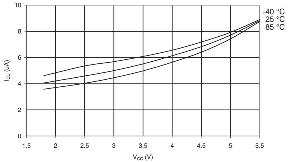
Figure 28-61. ATmega164PA: Power-down Supply Current vs. V_{CC} (Watchdog Timer Enabled).
