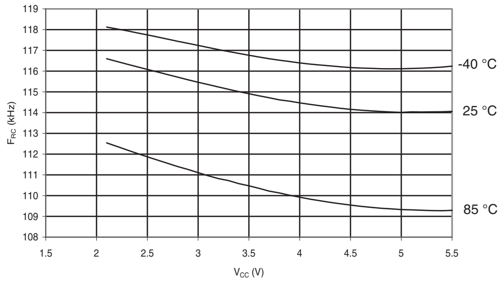
Figure 28-282. ATmega644PA: Watchdog Oscillator Frequency vs. V_{CC}
