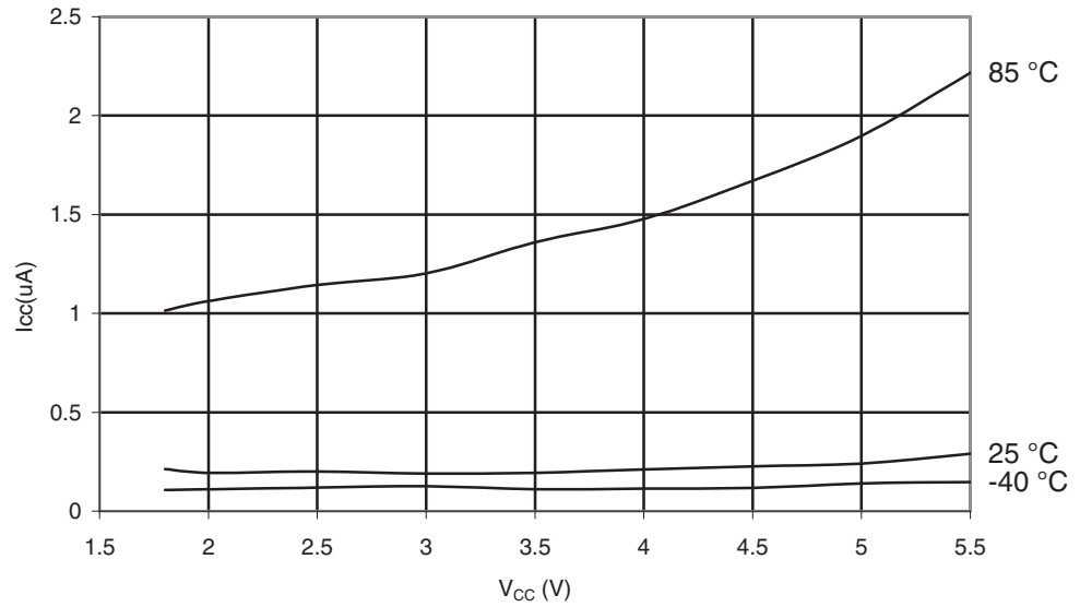
Figure 28-258. ATmega644PA: Power-save Supply Current vs. V_{CC} (Watchdog Timer Disabled and 32 kHz Crystal Oscillator Running).
