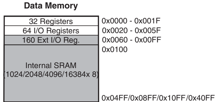
Figure 7-2. Data Memory Map for ATmega164A/164PA/324A/324PA/644A/644PA/1284/1284P
