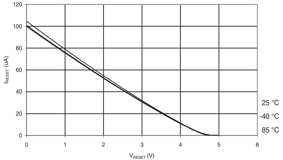
Figure 28-167. ATmega324PA: Reset Pull-up Resistor Current vs. Reset Pin Voltage ( V_{CC} = 5V ).
