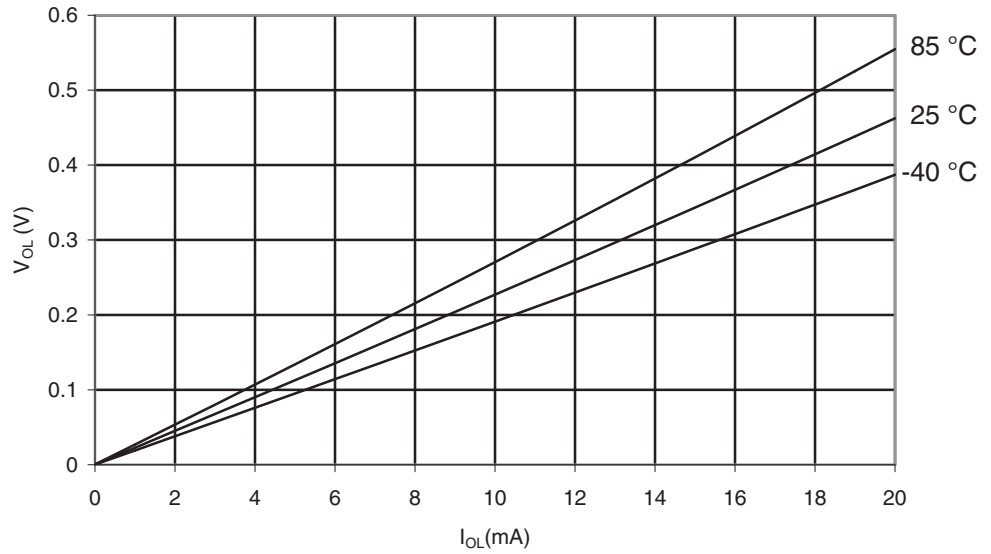
Figure 28-367. ATmega1284P: I/O Pin Output Voltage vs. Sink Current ( V_{CC} = 5V )
