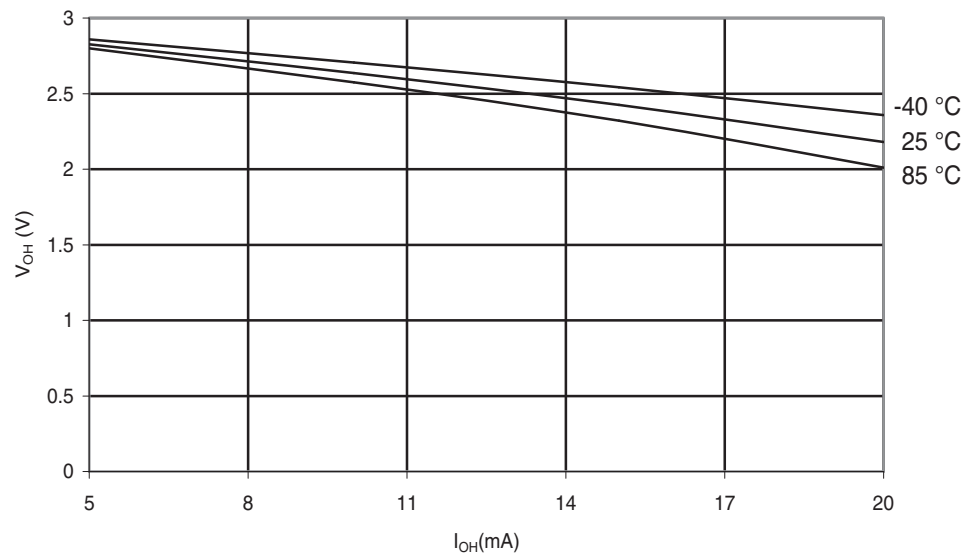
Figure 28-121. ATmega324A: I/O Pin Output Voltage vs. Source Current ( V_{CC} = 3V ).
