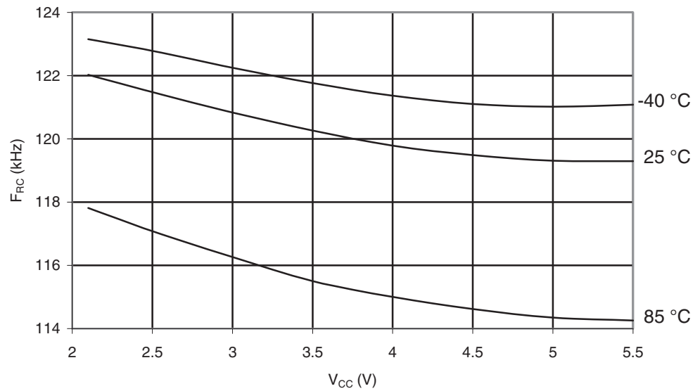
Figure 28-332. ATmega1284: Watchdog Oscillator Frequency vs. V_{CC}
