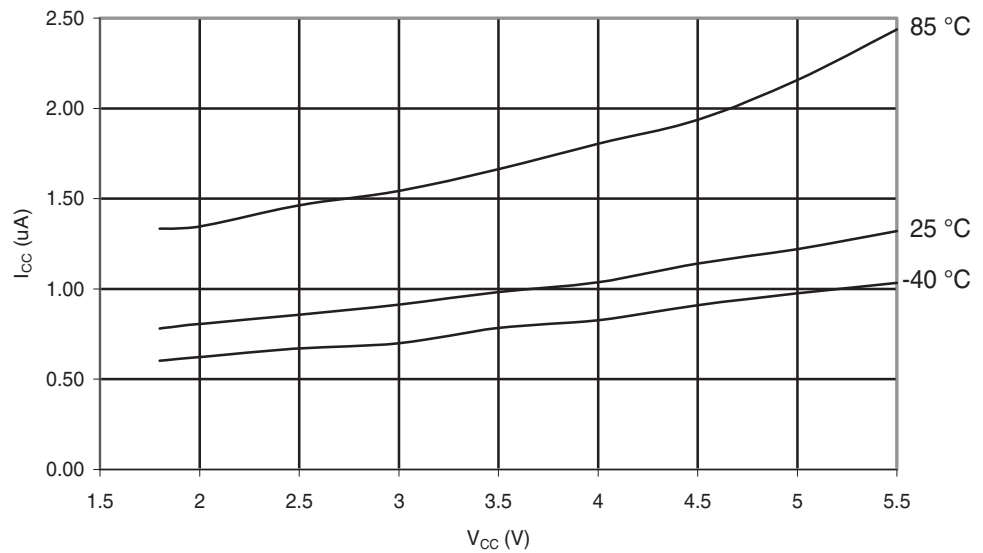
Figure 28-160. ATmega324PA: Power-save Supply Current vs. V_{CC} (Watchdog Timer Disabled and 32 kHz Crystal Oscillator Running).
