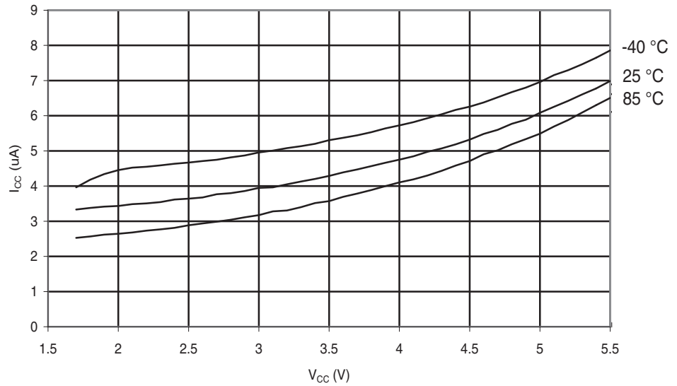
Figure 28-242. ATmega644A: Watchdog Timer Current vs. V_{CC}
