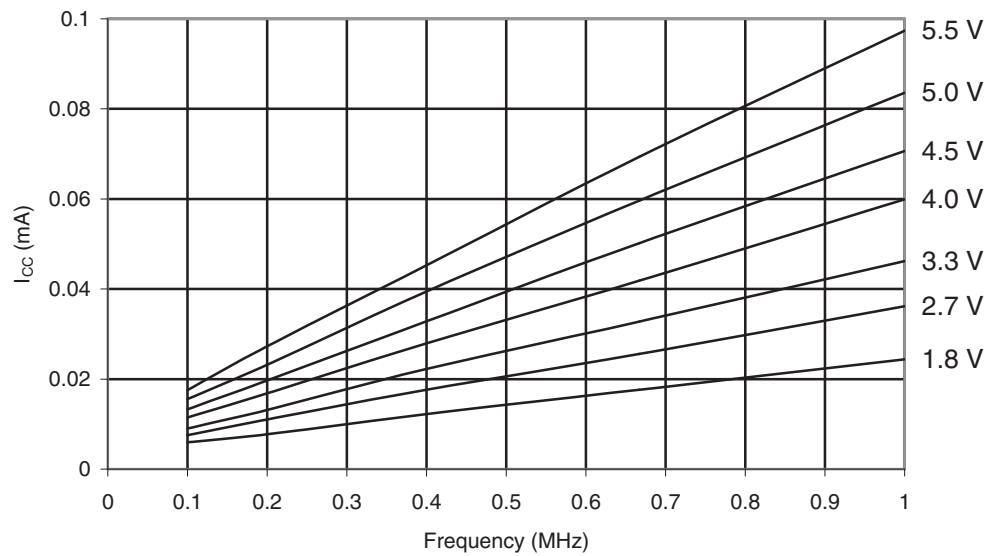
Figure 28-342. ATmega1284: Reset Supply Current vs. Low Frequency (0.1 - 1.0 MHz)
