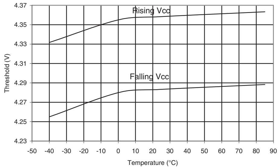
Figure 28-326. ATmega1284: BOD Threshold vs. Temperature ( V_{BOT} = 4.3V )
