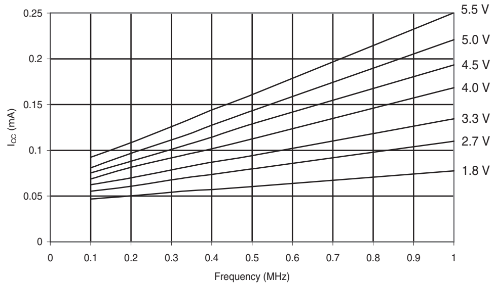
Figure 28-104. ATmega324A: Idle Supply Current vs. V_{CC} (0.1 - 1.0 MHz).
