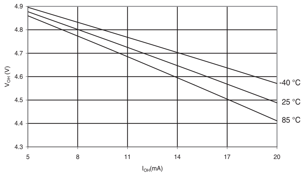
Figure 28-122. ATmega324A: I/O Pin Output Voltage vs. Source Current ( V_{CC} = 5V ).
