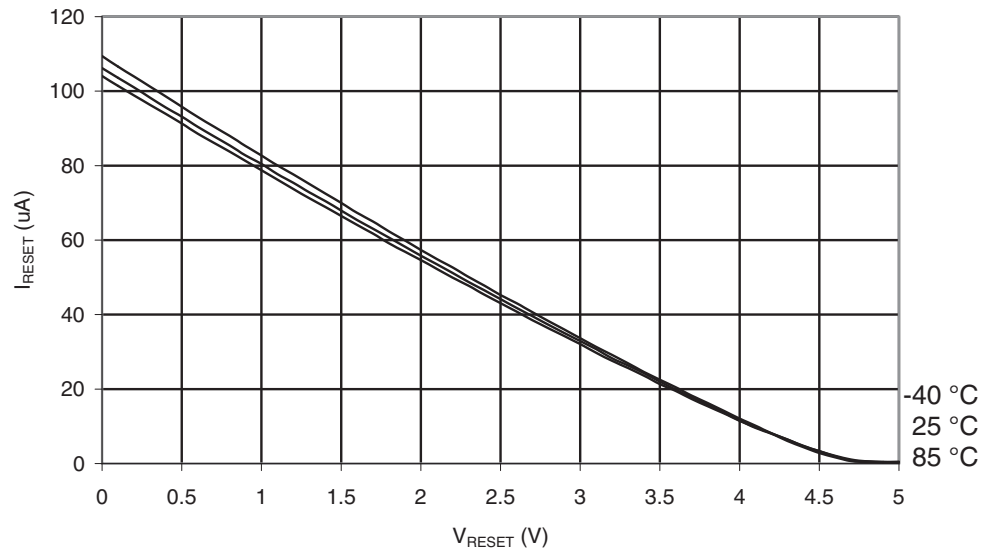
Figure 28-364. ATmega1284P: Reset Pull-up Resistor Current vs. Reset Pin Voltage ( V_{CC} = 5V )
