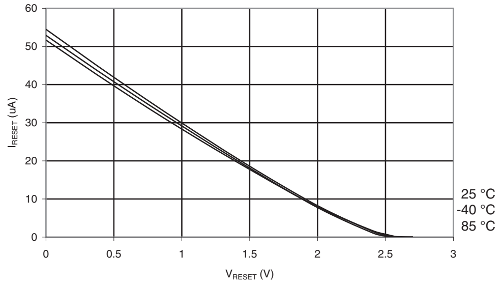
Figure 28-364. ATmega1284P: Reset Pull-up Resistor Current vs. Reset Pin Voltage ( V_{CC} = 5V )
