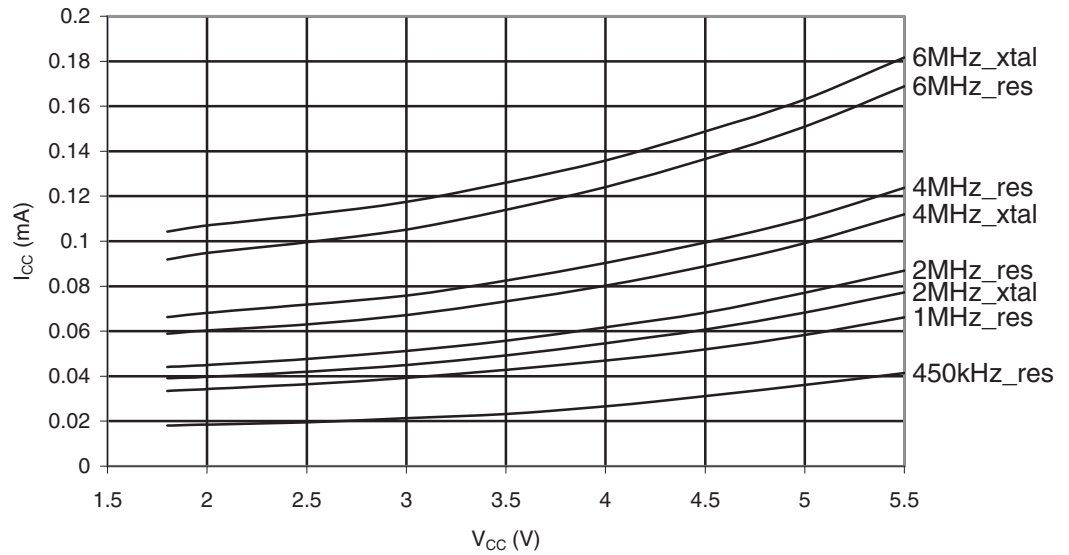
Figure 28-14. ATmega164A: Standby Supply Current vs. V_{CC} (Watchdog Timer Disabled).
