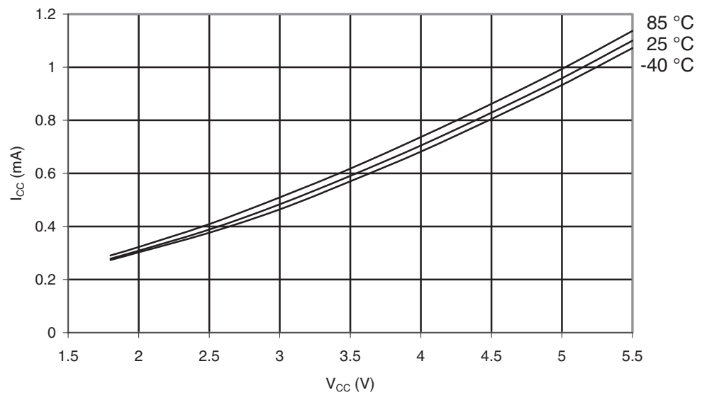
Figure 28-57. ATmega164PA: Idle Supply Current vs. V_{CC} (Internal RC Oscillator, 8 MHz).
