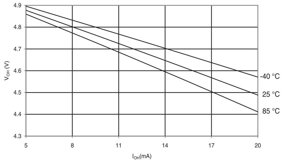
Figure 28-171. ATmega324PA: I/O Pin Output Voltage vs. Source Current ( V_{CC} = 5V ).
