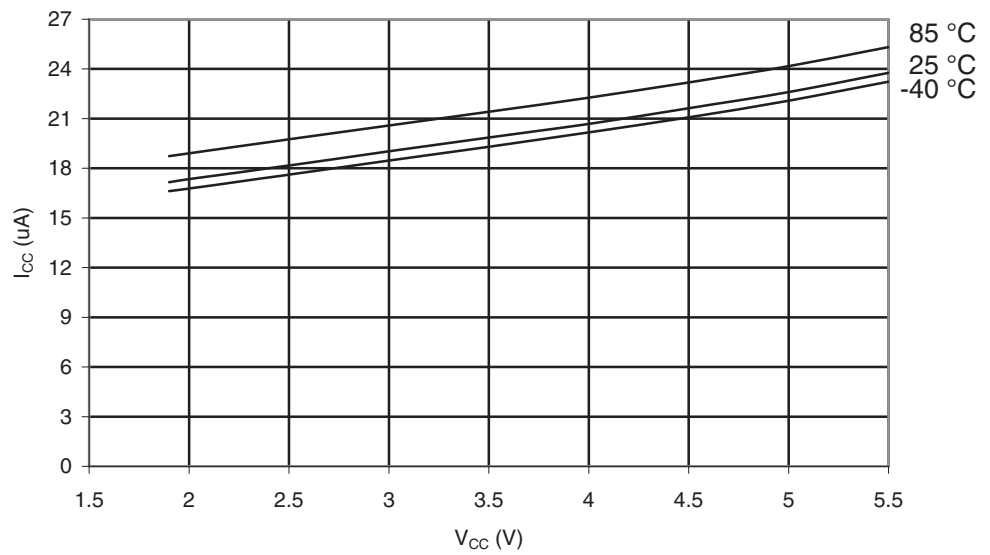
Figure 28-93. ATmega164PA: Brownout Detector Current vs. V_{CC}
