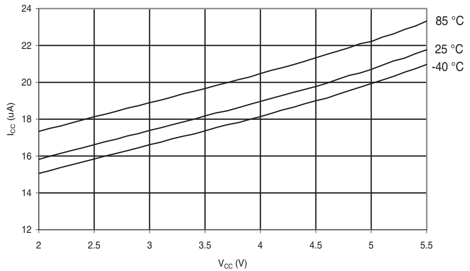
Figure 28-240. ATmega644A: Brownout Detector Current vs. V_{CC}
