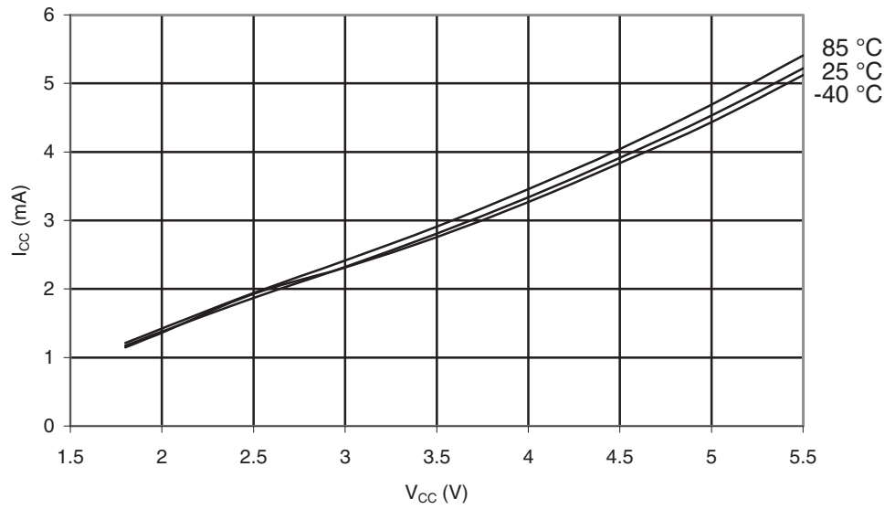
Figure 28-3. ATmega164A: Active Supply Current vs. V_{CC} (Internal RC Oscillator, 8 MHz).
