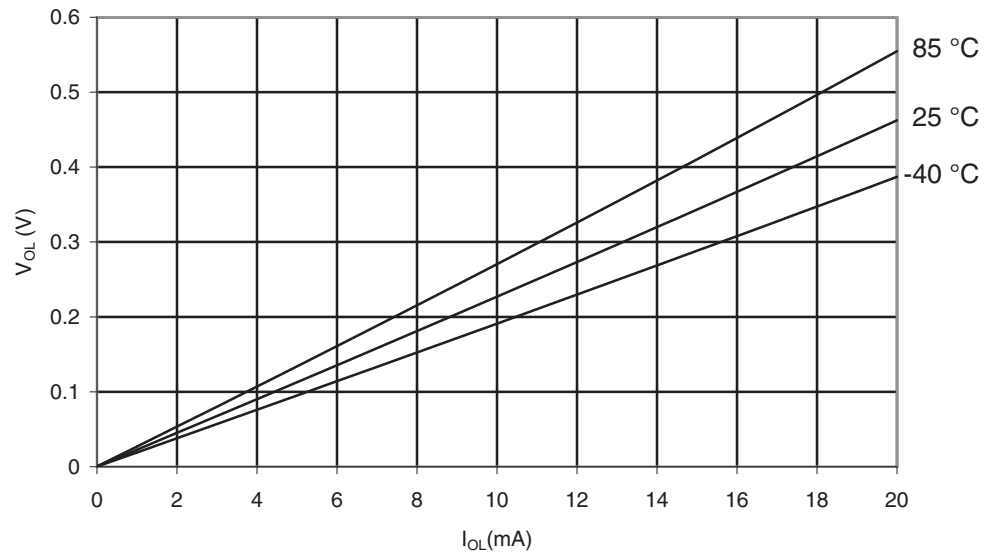
Figure 28-317. ATmega1284: I/O Pin Output Voltage vs. Sink Current ( V_{CC} = 5V )
