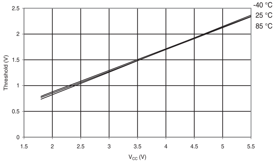
Figure 28-176. ATmega324PA: Reset Pin Input Threshold vs. V_{CC} ( V_{IL} , I/O Pin Read as '0').
