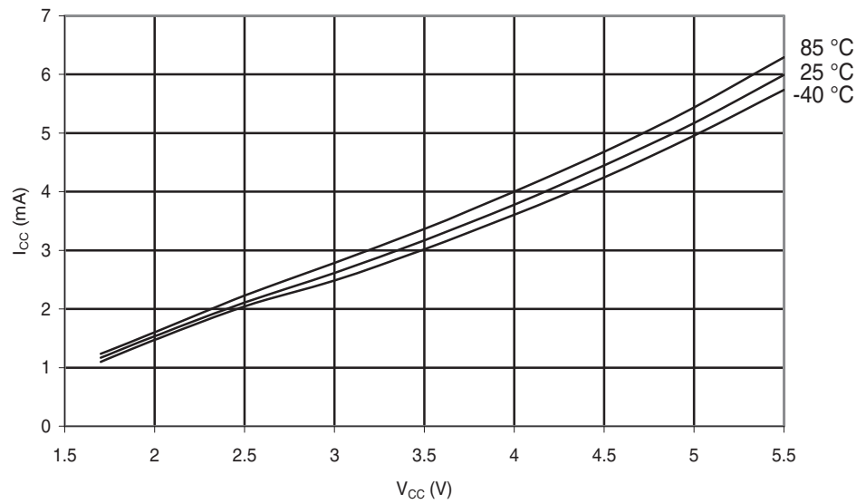
Figure 28-101. ATmega324A: Active Supply Current vs. V_{CC} (Internal RC Oscillator, 8 MHz).
