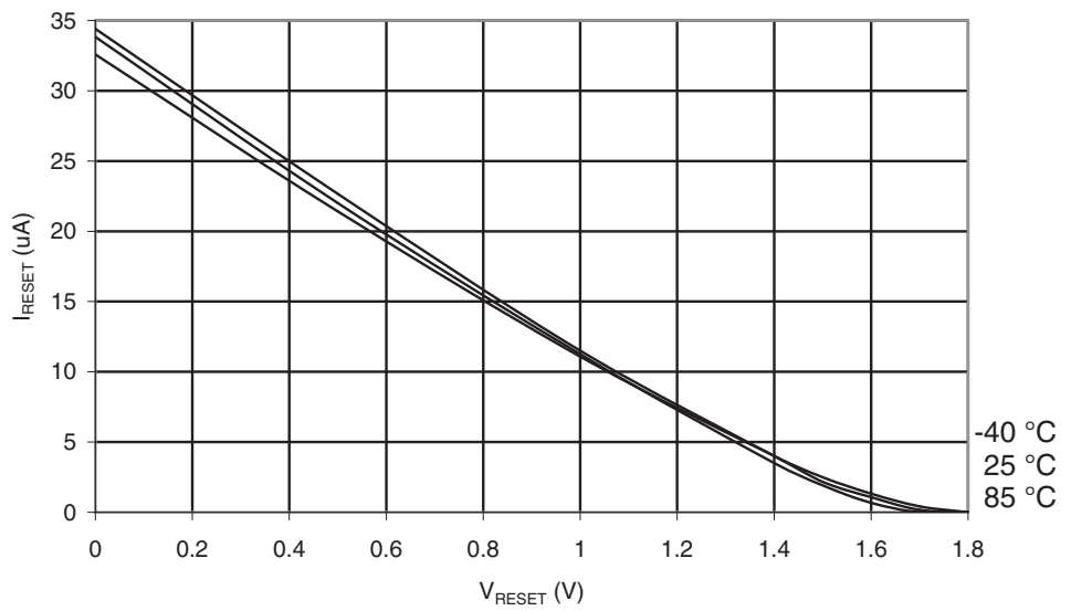
Figure 28-362. ATmega1284P: Reset Pull-up Resistor Current vs. Reset Pin Voltage ( V_{CC} = 1.8V )
