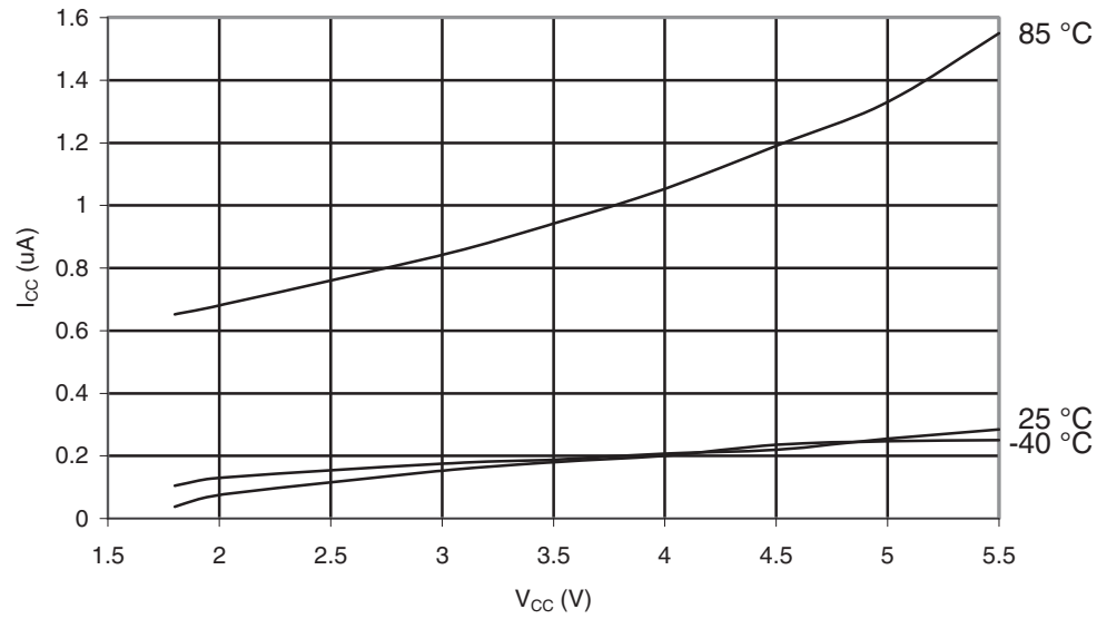
Figure 28-60. ATmega164PA: Power-down Supply Current vs. V_{CC} (Watchdog Timer Disabled).
