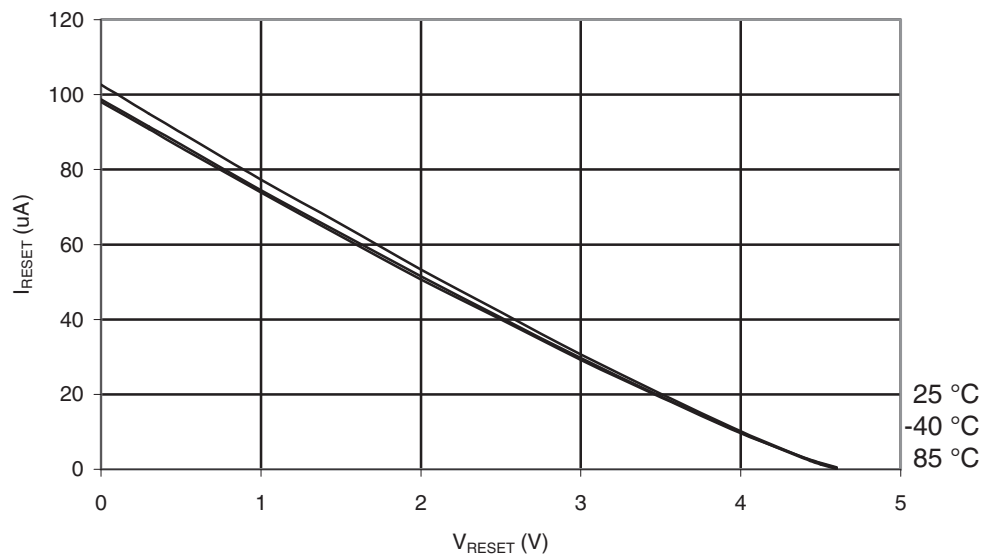
Figure 28-216. ATmega644A: Reset Pull-up Resistor Current vs. Reset Pin Voltage ( V_{CC} = 5V ).
