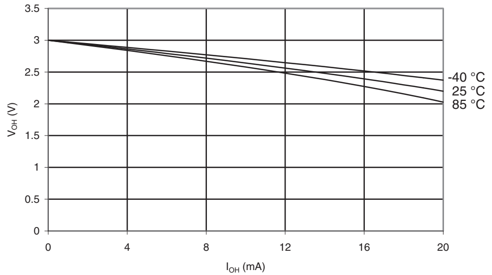
Figure 28-72. ATmega164PA: I/O Pin Output Voltage vs. Source Current ( V_{CC} = 3V ).
