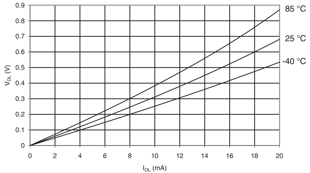
Figure 28-366. ATmega1284P: I/O Pin Output Voltage vs. Sink Current ( V_{CC} = 3V )
