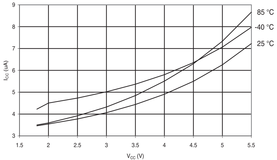
Figure 28-257. ATmega644PA: Power-down Supply Current vs. V_{CC} (Watchdog Timer Enabled).
