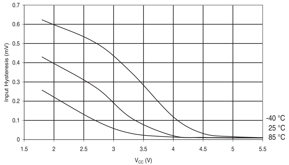
Figure 28-275. ATmega644PA: Reset Pin Input Hysteresis vs. V_{CC}
