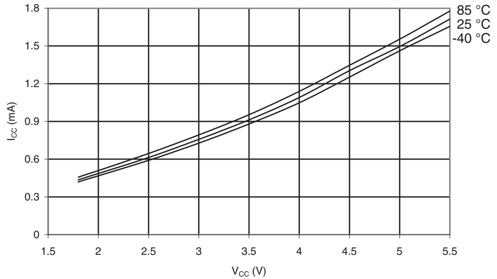
Figure 28-348. ATmega1284P: Active Supply Current vs. V_{CC} (Internal RC Oscillator, 1 MHz)
