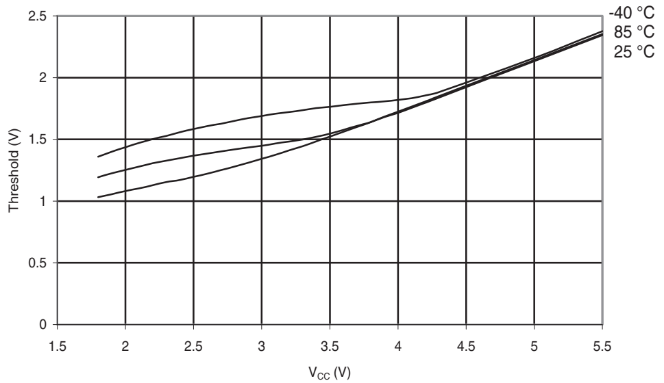
Figure 28-175. ATmega324PA: Reset Pin Input Threshold vs. V_{CC} ( V_{IH} , I/O Pin Read as '1').
