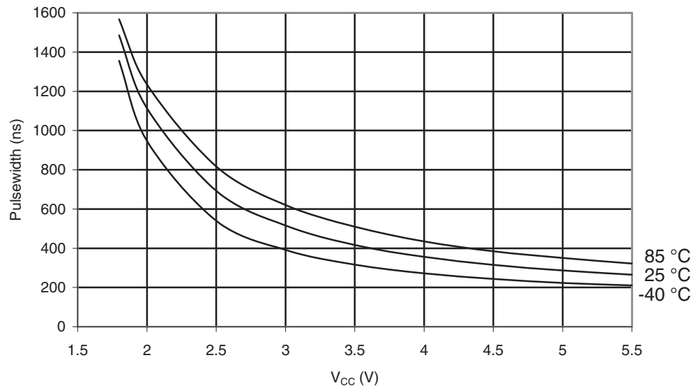
Figure 28-98. ATmega164PA: Minimum Reset Pulsewidth vs. V_{CC}
