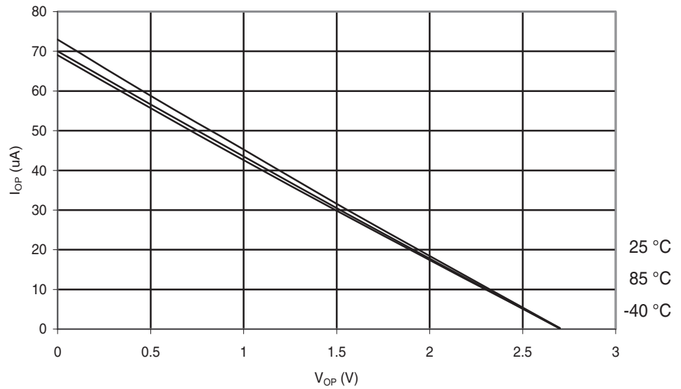
Figure 28-163. ATmega324PA: I/O Pin Pull-up Resistor Current vs. Input Voltage ( V_{CC} = 2.7V ).
