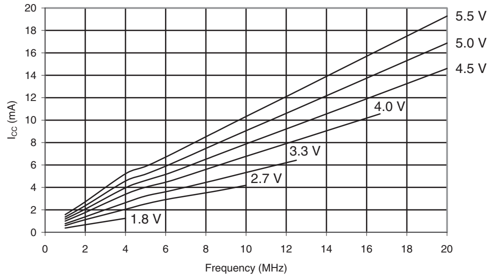
Figure 28-296. ATmega1284: Active Supply Current vs. Frequency (1 - 20 MHz)
