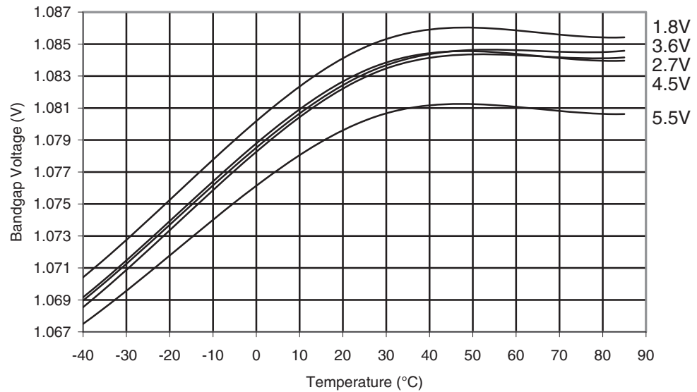
Figure 28-280. ATmega324PA: Bandgap Voltage vs. Temperature
