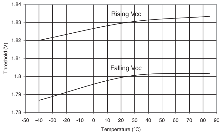
Figure 28-378. ATmega1284P: BOD Threshold vs. Temperature ( V_{BOT} = 1.8V )
