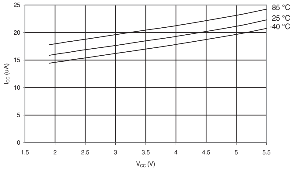
Figure 28-191. ATmega324PA: Brownout Detector Current vs. V_{CC}
