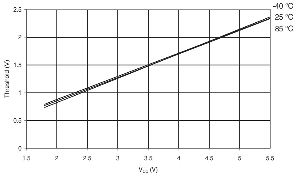
Figure 28-127. ATmega324A: Reset Pin Input Threshold vs. V_{CC} ( V_{IL} , I/O Pin Read as '0').
