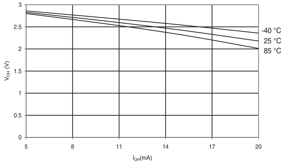
Figure 28-170. ATmega324PA: I/O Pin Output Voltage vs. Source Current ( V_{CC} = 3V ).
