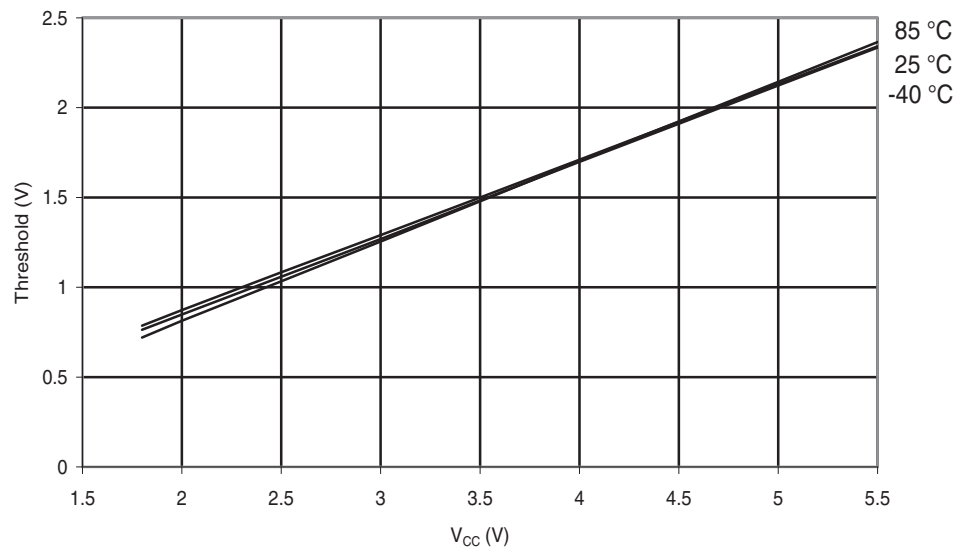
Figure 28-222. ATmega644A: I/O Pin Input Threshold vs. V_{CC} ( V_{IL} , I/O Pin Read as '0').
