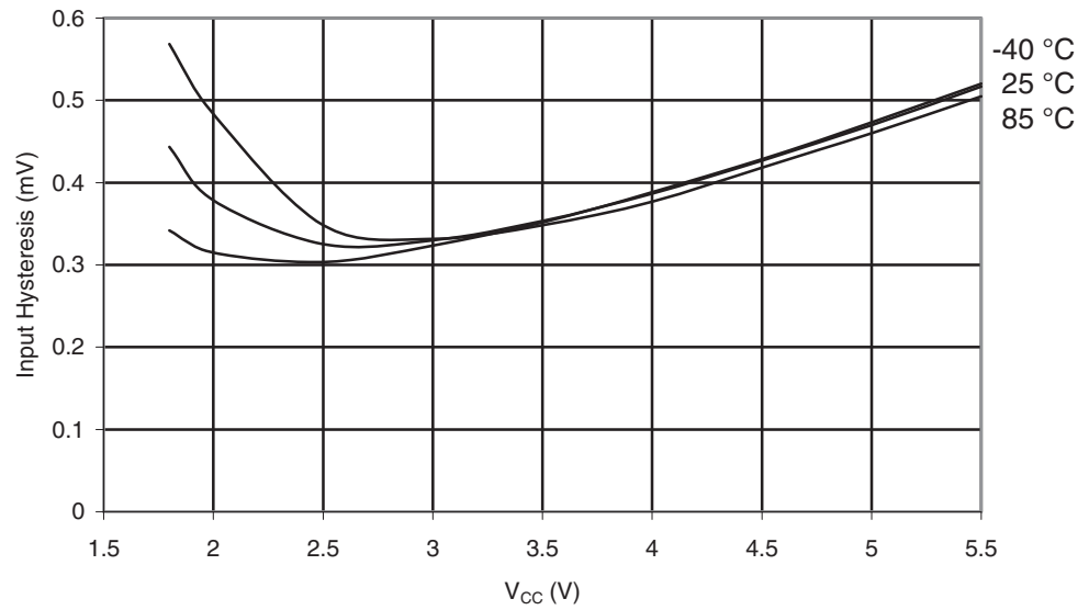
Figure 28-76. ATmega164PA: I/O Pin Input Hysteresis vs. V_{CC}
