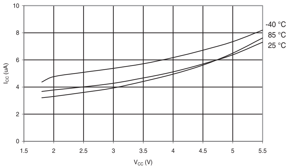
Figure 28-110. ATmega324A: Power-down Supply Current vs. V_{CC} (Watchdog Timer Enabled).
