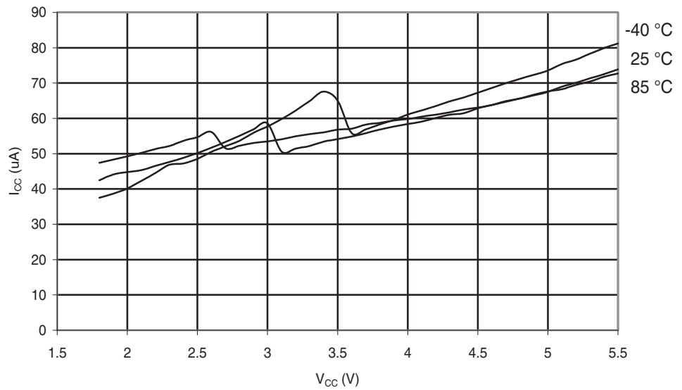
Figure 28-140. ATmega324A: Analog Comparator Current vs. V_{CC}
