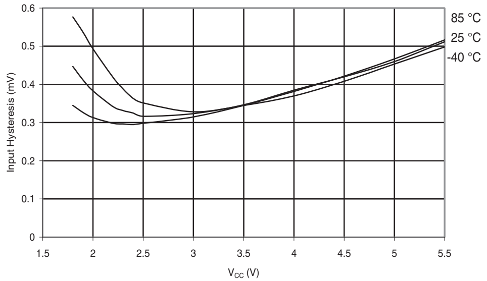
Figure 28-174. ATmega324PA: I/O Pin Input Hysteresis vs. V_{CC}
