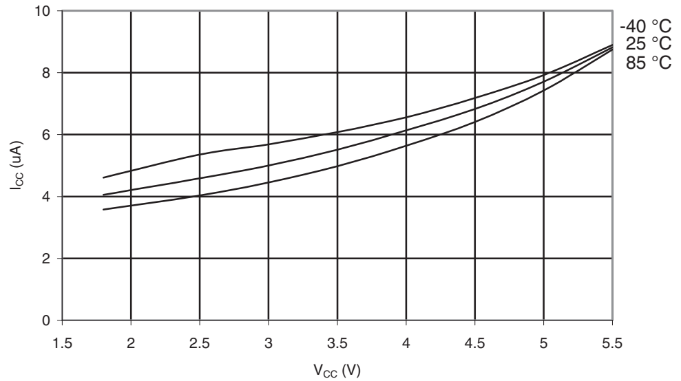
Figure 28-12. ATmega164A: Power-down Supply Current vs. V_{CC} (Watchdog Timer Enabled).
