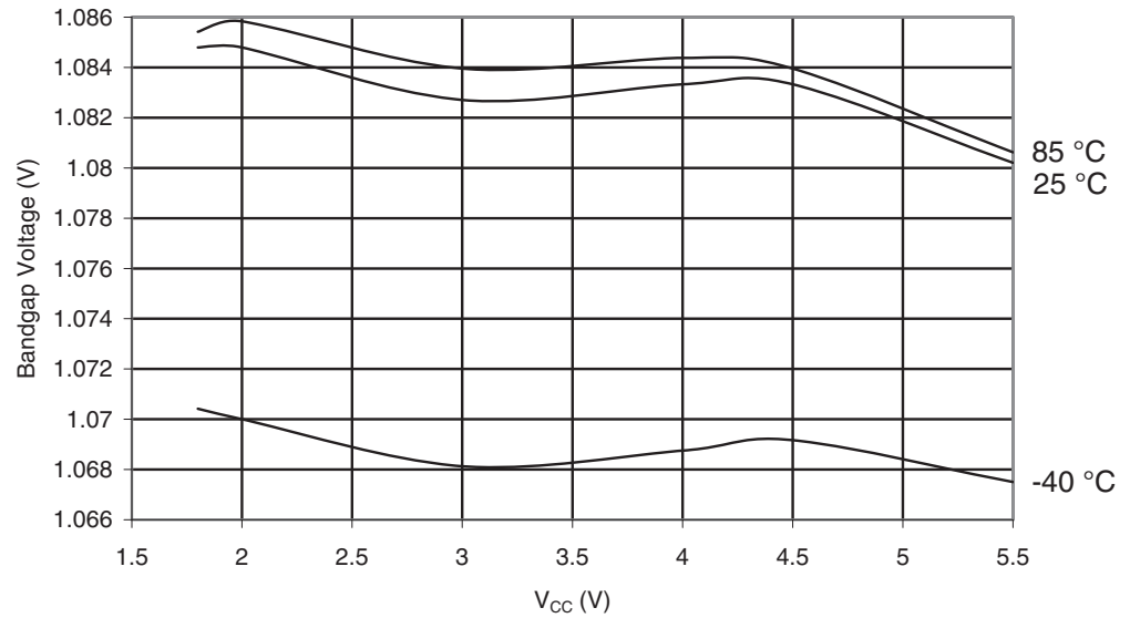
Figure 28-230. ATmega644A: Calibrated Bandgap Voltage vs. V_{CC}
