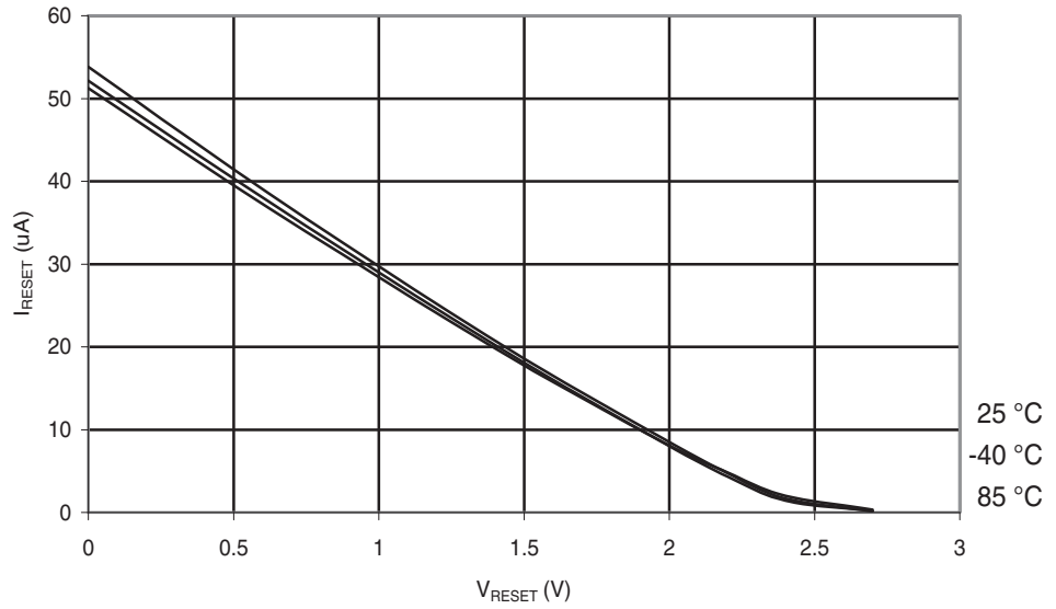
Figure 28-166. ATmega324PA: Reset Pull-up Resistor Current vs. Reset Pin Voltage ( V_{CC} = 2.7V ).
