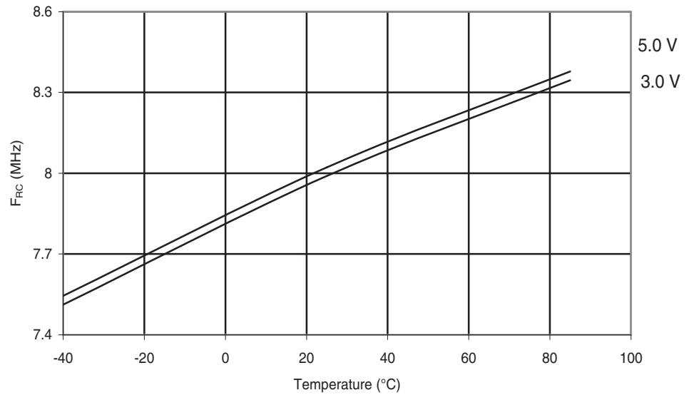
Figure 28-186. ATmega324PA: Calibrated 8 MHz RC Oscillator vs. Temperature
