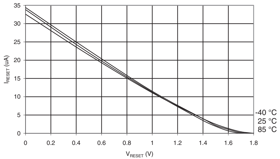
Figure 28-312. ATmega1284: Reset Pull-up Resistor Current vs. Reset Pin Voltage ( V_{CC} = 1.8V )
