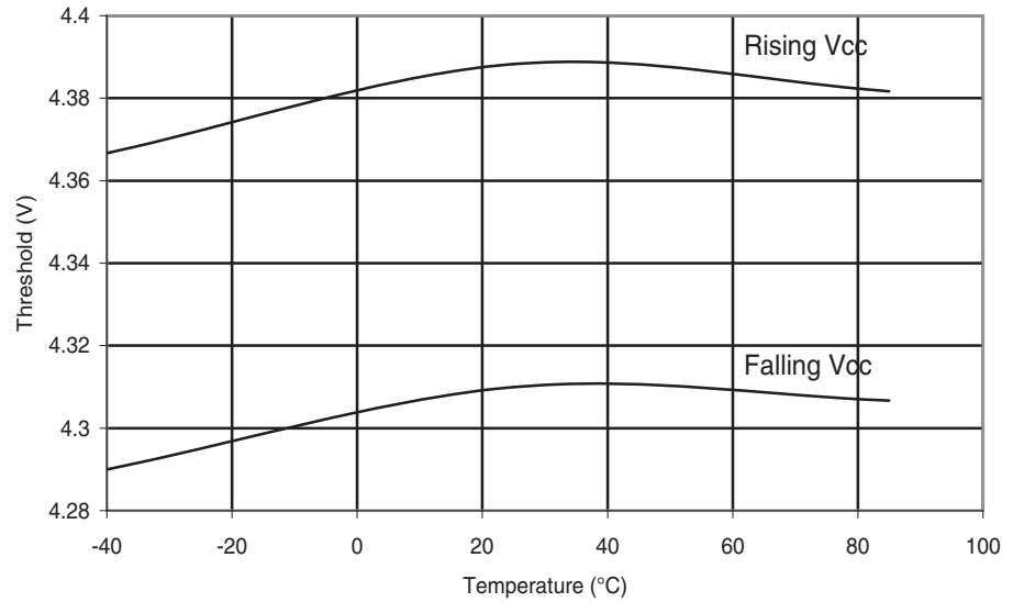
Figure 28-178. ATmega324PA: BOD Threshold vs. Temperature ( V_{BOT} = 4.3V )
