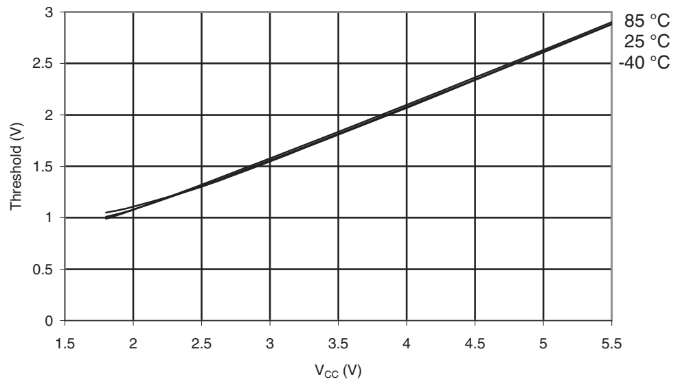
Figure 28-74. ATmega164PA: I/O Pin Input Threshold vs. V_{CC} ( V_{IH} , I/O Pin Read as '1').
