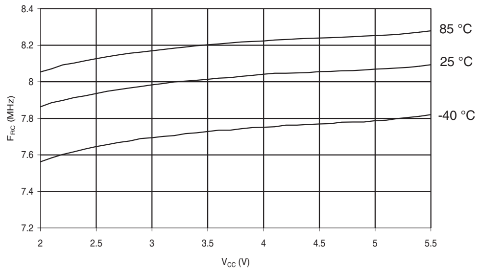
Figure 28-234. ATmega644A: Calibrated 8 MHz RC Oscillator vs. V_{CC}
