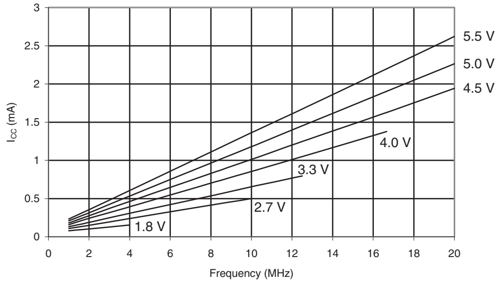
Figure 28-7. ATmega164A: Idle Supply Current vs. V_{CC} (1 - 20 MHz).
