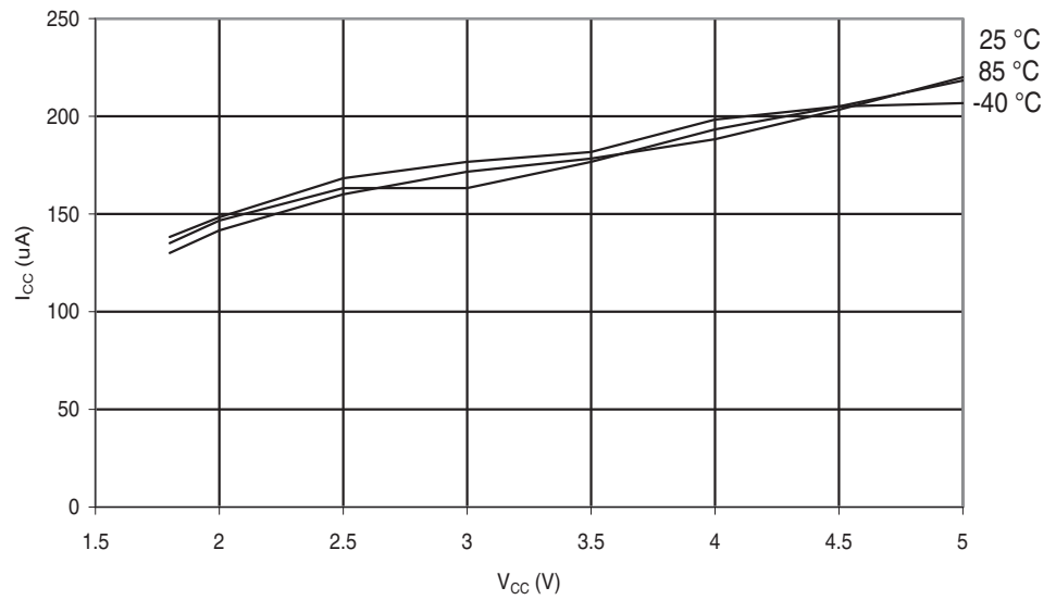
Figure 28-237. ATmega644A: ADC Current vs. V_{CC} (AREF = AV_{CC} )
