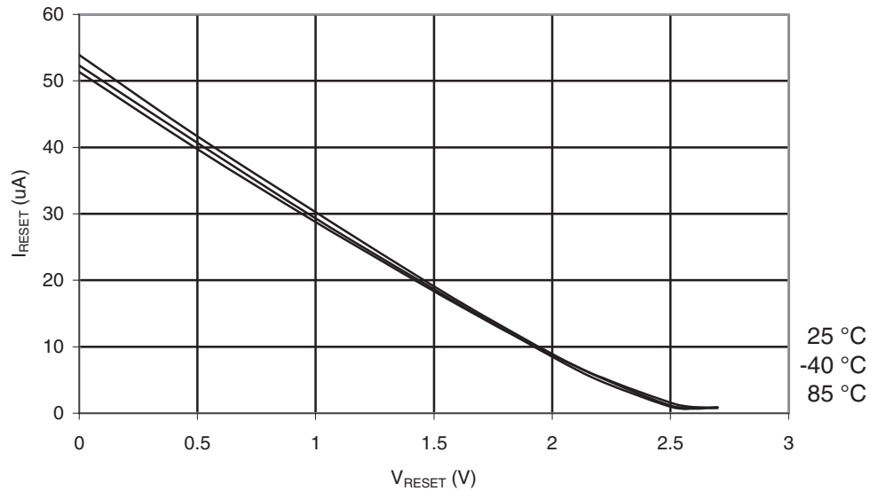
Figure 28-19. ATmega164A: Reset Pull-up Resistor Current vs. Reset Pin Voltage ( V_{CC} = 2.7V ).
