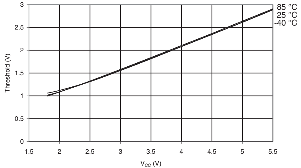
Figure 28-370. ATmega1284P: I/O Pin Input Threshold vs. V_{CC} ( V_{IH} , I/O Pin Read as '1')
