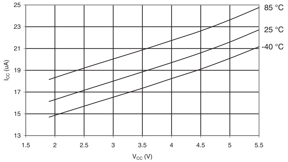
Figure 28-389. ATmega1284P: Brownout Detector Current vs. V_{CC}
