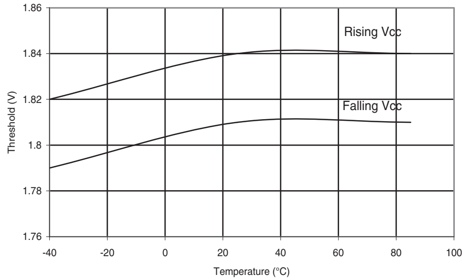
Figure 28-131. ATmega324A: BOD Threshold vs. Temperature ( V_{BOT} = 1.8V )
