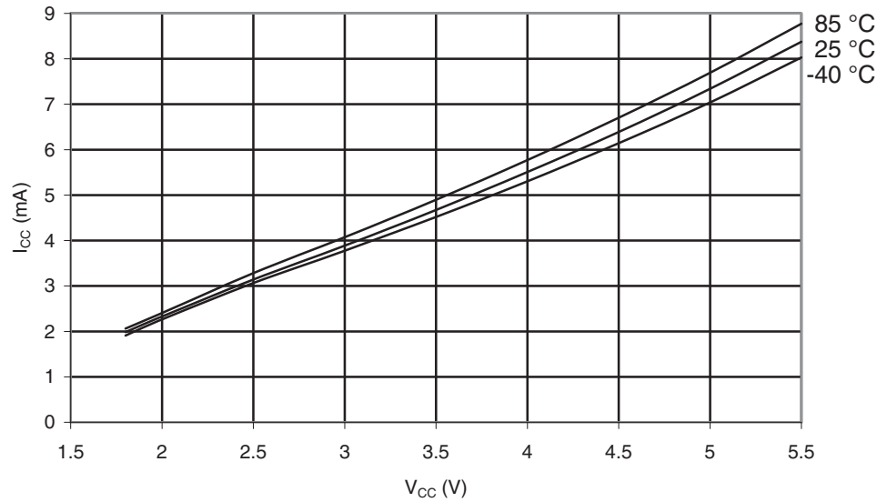
Figure 28-348. ATmega1284P: Active Supply Current vs. V_{CC} (Internal RC Oscillator, 1 MHz)
