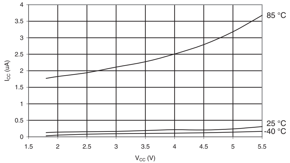
Figure 28-356. ATmega1284P: Power-down Supply Current vs. V_{CC} (Watchdog Timer Enabled)
