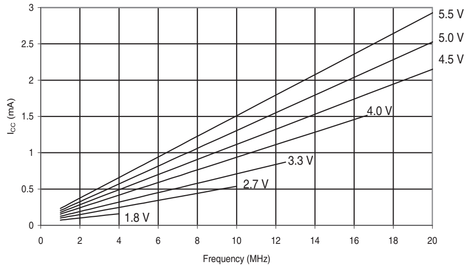
Figure 28-252. ATmega644PA: Idle Supply Current vs. V_{CC} (1 - 20 MHz).
