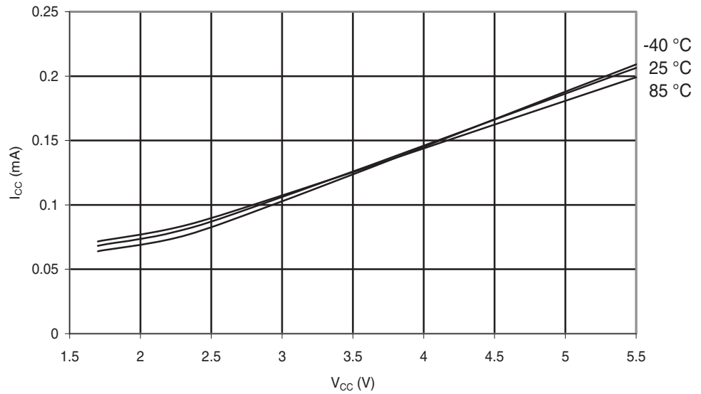
Figure 28-103. ATmega324A: Active Supply Current vs. V_{CC} (Internal RC Oscillator, 128 kHz).
