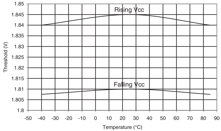
Figure 28-33. ATmega164A: BOD Threshold vs. Temperature ( V_{BOT} = 1.8V )
