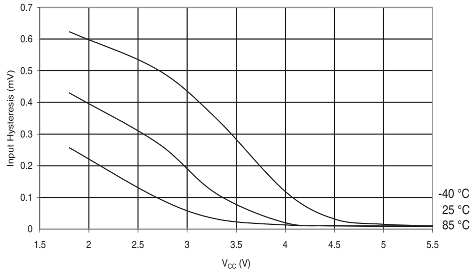
Figure 28-226. ATmega644A: Reset Pin Input Hysteresis vs. V_{CC}
