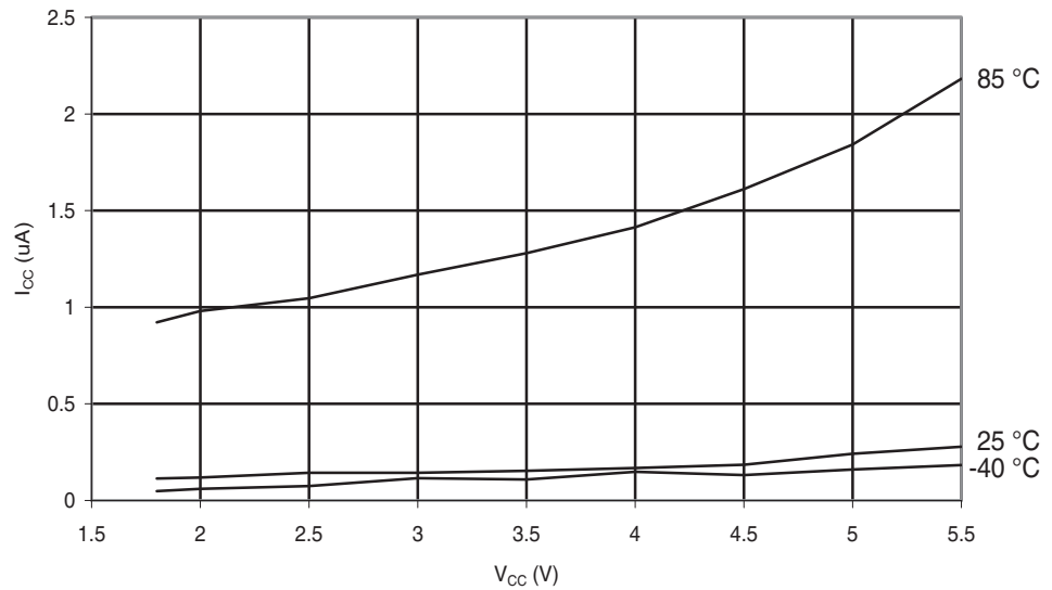
Figure 28-256. ATmega644PA: Power-down Supply Current vs. V_{CC} (Watchdog Timer Disabled).
