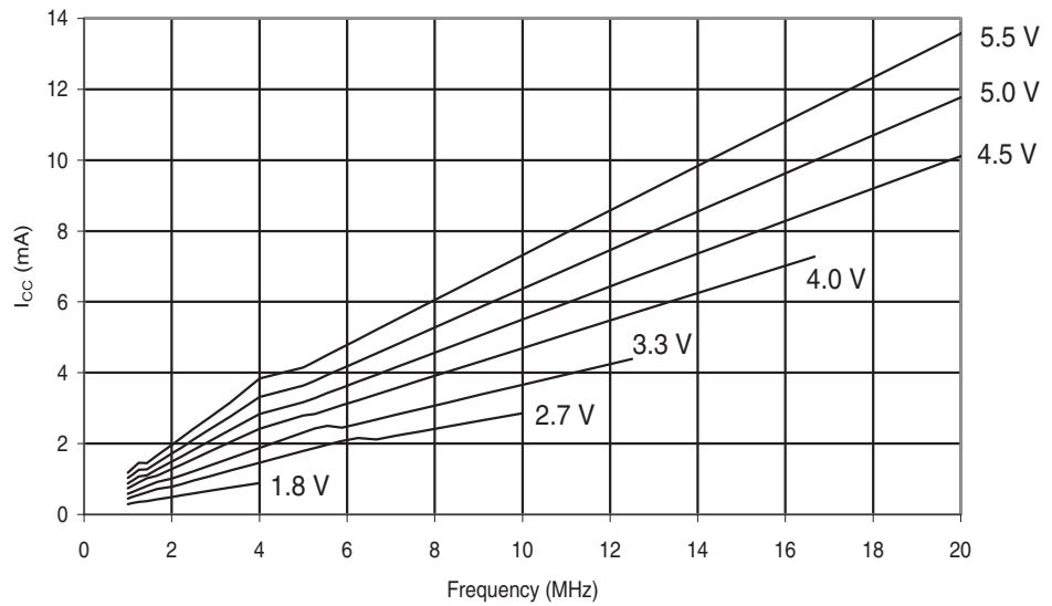
Figure 28-247. ATmega644PA: Active Supply Current vs. Frequency (1 - 20 MHz).
