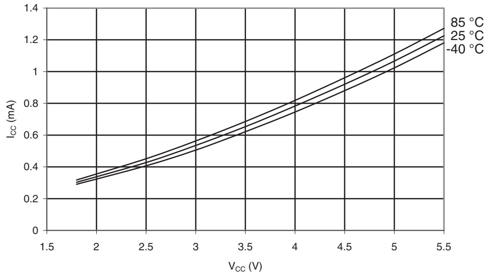
Figure 28-253. ATmega644PA: Idle Supply Current vs. V_{CC} (Internal RC Oscillator, 8 MHz).
