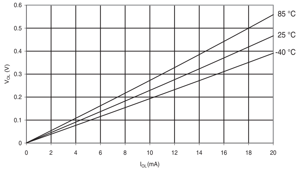
Figure 28-267. ATmega644PA: I/O Pin Output Voltage vs. Sink Current ( V_{CC} = 5V ).
