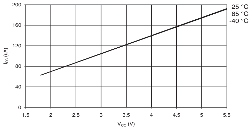
Figure 28-92. ATmega164PA: AREF External Reference Current vs. V_{CC}
