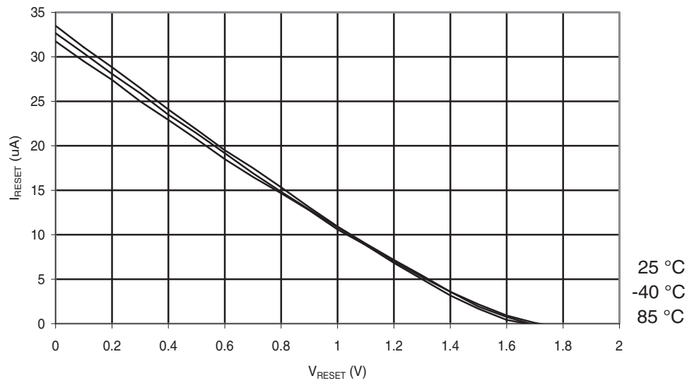
Figure 28-263. ATmega644PA: Reset Pull-up Resistor Current vs. Reset Pin Voltage ( V_{CC} = 1.8V ).
