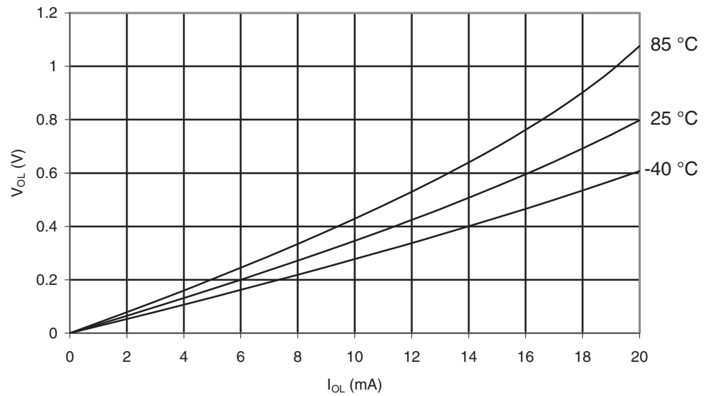
Figure 28-365. ATmega1284P: I/O Pin Output Voltage vs. Sink Current ( V_{CC} = 2.7V )
