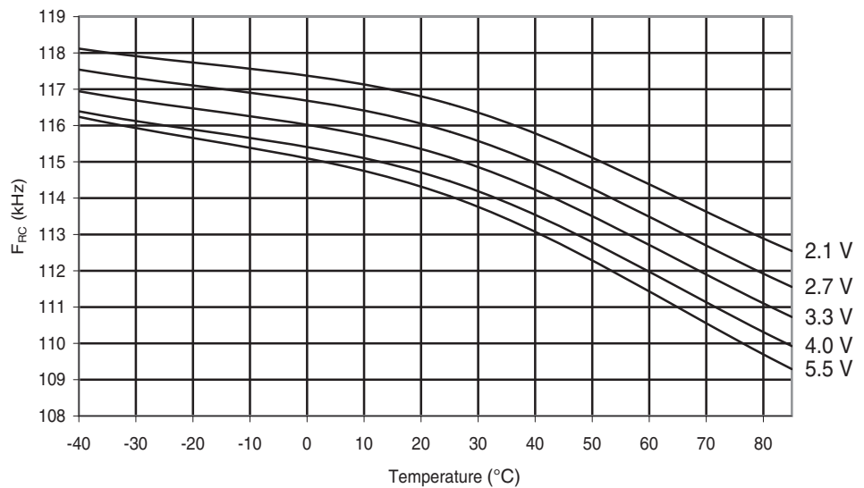
Figure 28-232. ATmega644A: Watchdog Oscillator Frequency vs. Temperature
