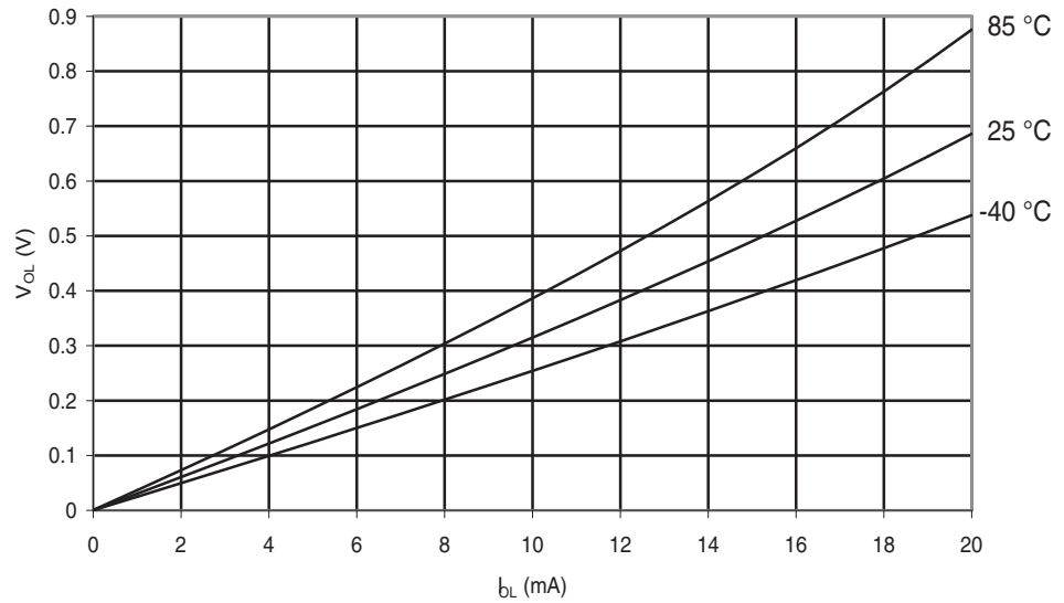
Figure 28-266. ATmega644PA: I/O Pin Output Voltage vs. Sink Current ( V_{CC} = 3V ).
