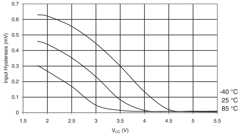
Figure 28-79. ATmega164PA: Reset Pin Input Hysteresis vs. V_{CC}
