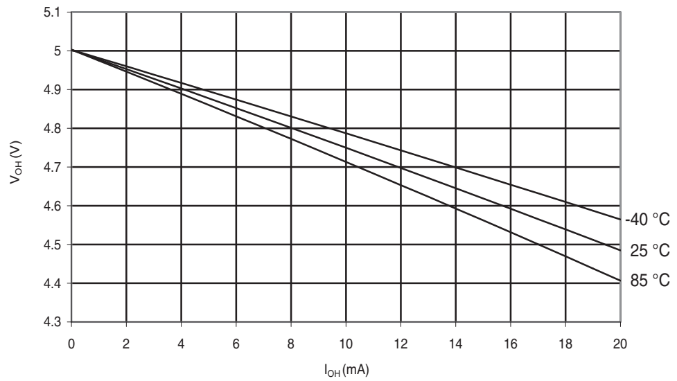
Figure 28-220. ATmega644A: I/O Pin Output Voltage vs. Source Current ( V_{CC} = 5V )
