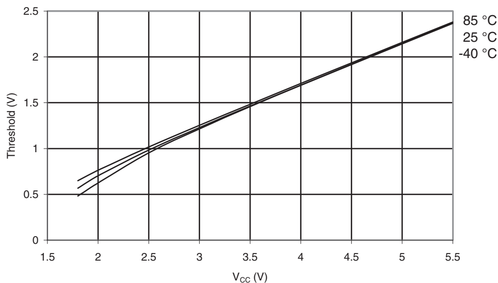
Figure 28-26. ATmega164A: I/O Pin Input Threshold vs. V_{CC} ( V_{IL} , I/O Pin Read as '0').
