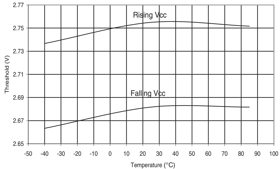
Figure 28-277. ATmega644PA: BOD Threshold vs. Temperature ( V_{BOT} = 2.7V )
