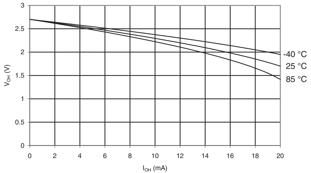
Figure 28-318. ATmega1284: I/O Pin Output Voltage vs. Source Current ( V_{CC} = 2.7V )
