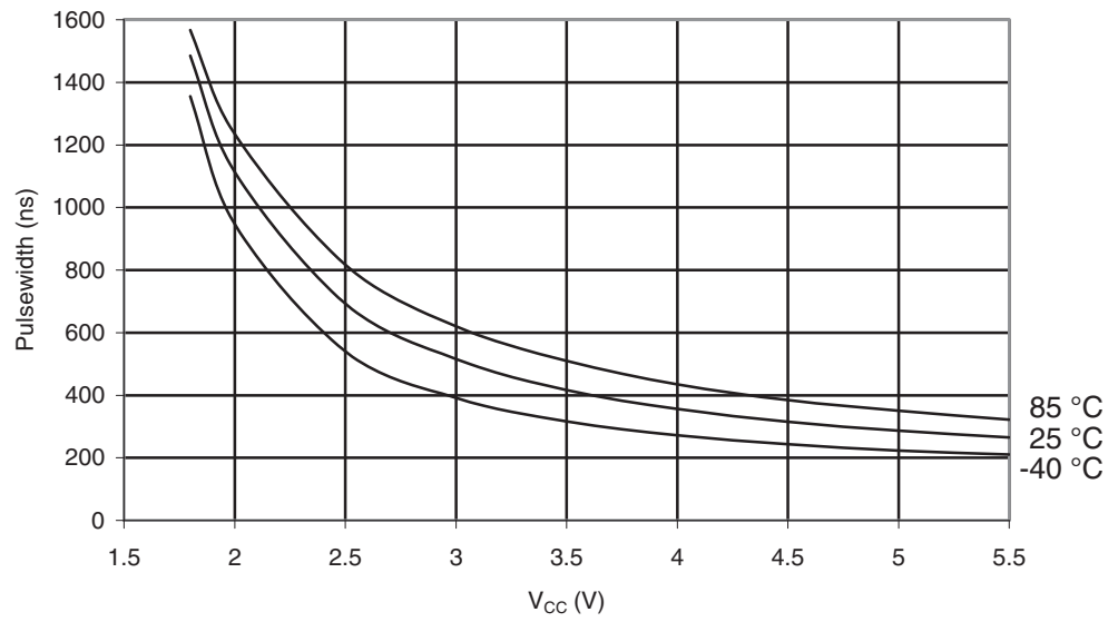
Figure 28-49. ATmega164A: Minimum Reset Pulsewidth vs. V_{CC}
