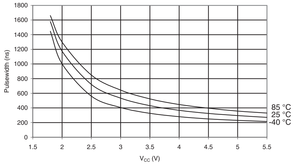
Figure 28-294. ATmega644PA: Minimum Reset Pulsewidth vs. V_{CC}
