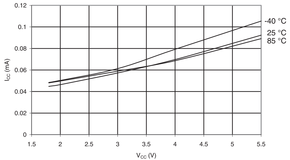
Figure 28-10. ATmega164A: Idle Supply Current vs. V_{CC} (Internal RC Oscillator, 128 kHz).
