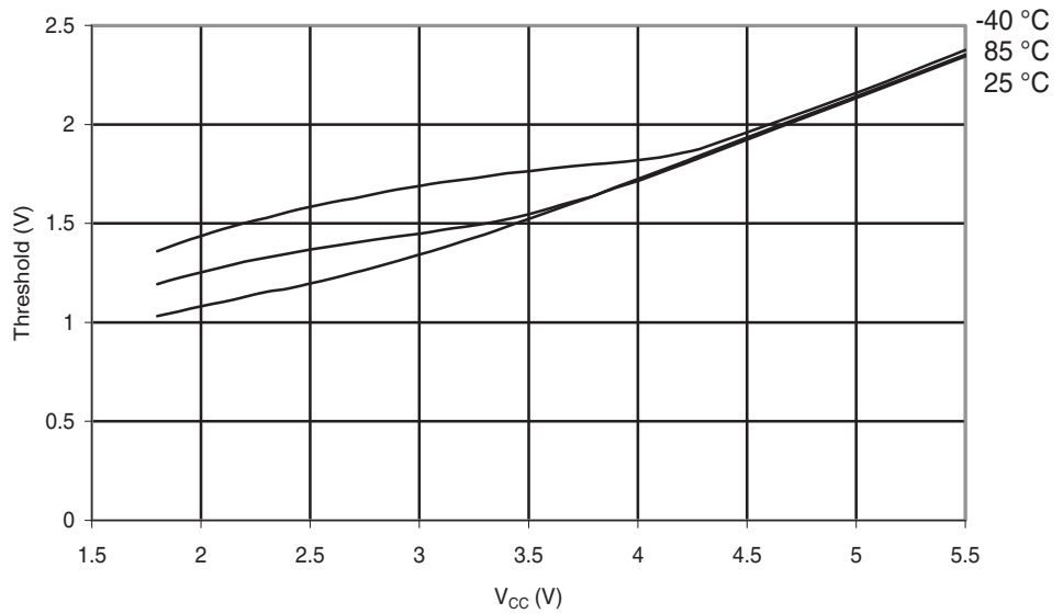
Figure 28-126. ATmega324A: Reset Pin Input Threshold vs. V_{CC} ( V_{IH} , I/O Pin Read as '1').
