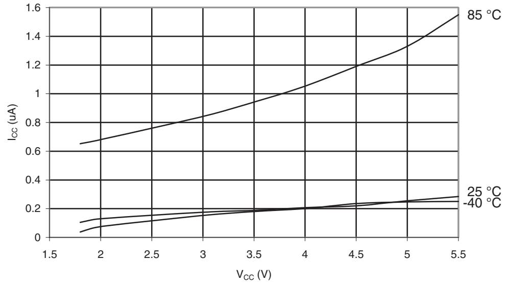
Figure 28-11. ATmega164A: Power-down Supply Current vs. V_{CC} (Watchdog Timer Disabled).
