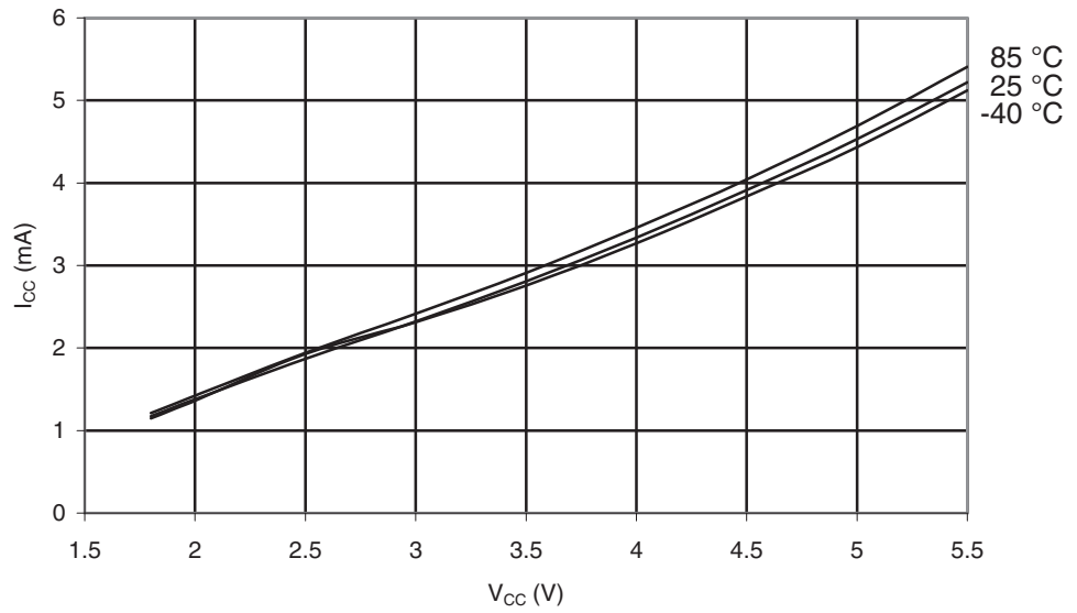
Figure 28-52. ATmega164PA: Active Supply Current vs. V_{CC} (Internal RC Oscillator, 8 MHz).
