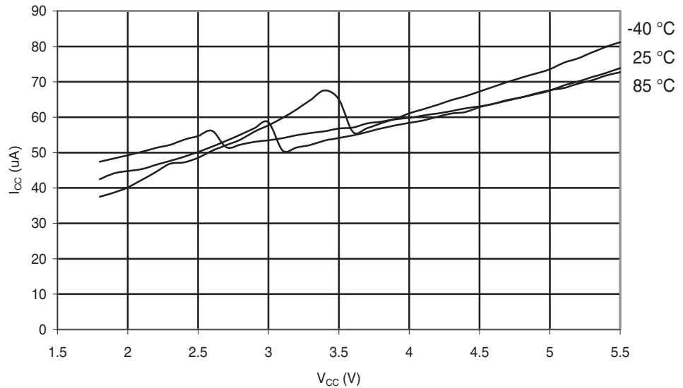
Figure 28-189. ATmega324PA: Analog Comparator Current vs. V_{CC}
