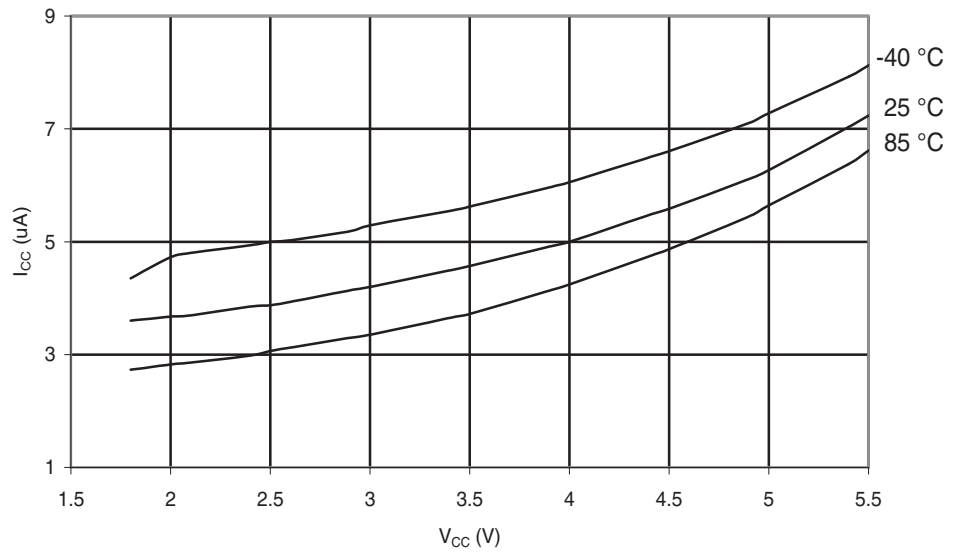
Figure 28-144. ATmega324A: Watchdog Timer Current vs. V_{CC}
