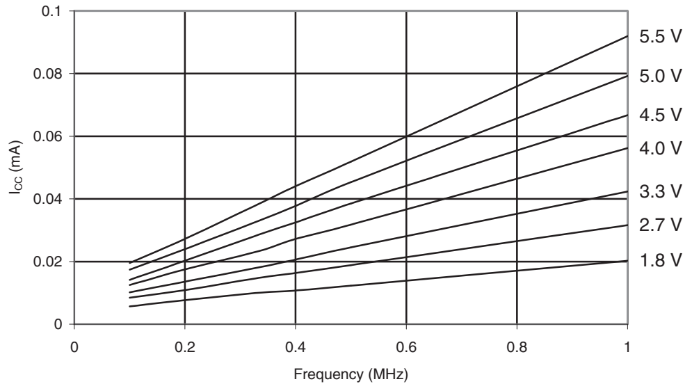
Figure 28-47. ATmega164A: Reset Supply Current vs. Low Frequency (0.1 - 1.0 MHz).
