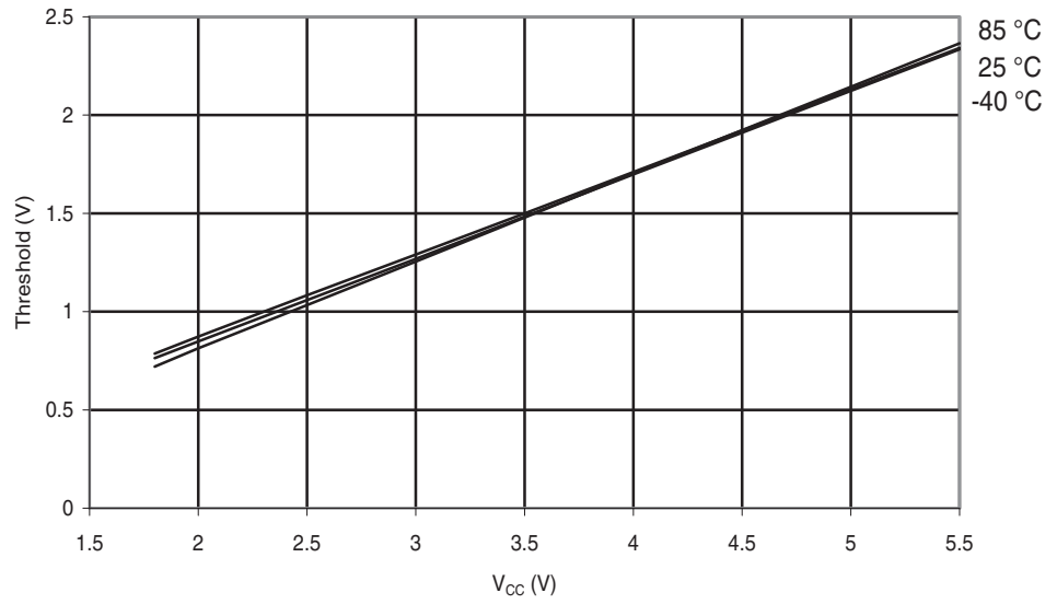
Figure 28-274. ATmega644PA: Reset Pin Input Threshold vs. V_{CC} ( V_{IL} , I/O Pin Read as '0').
