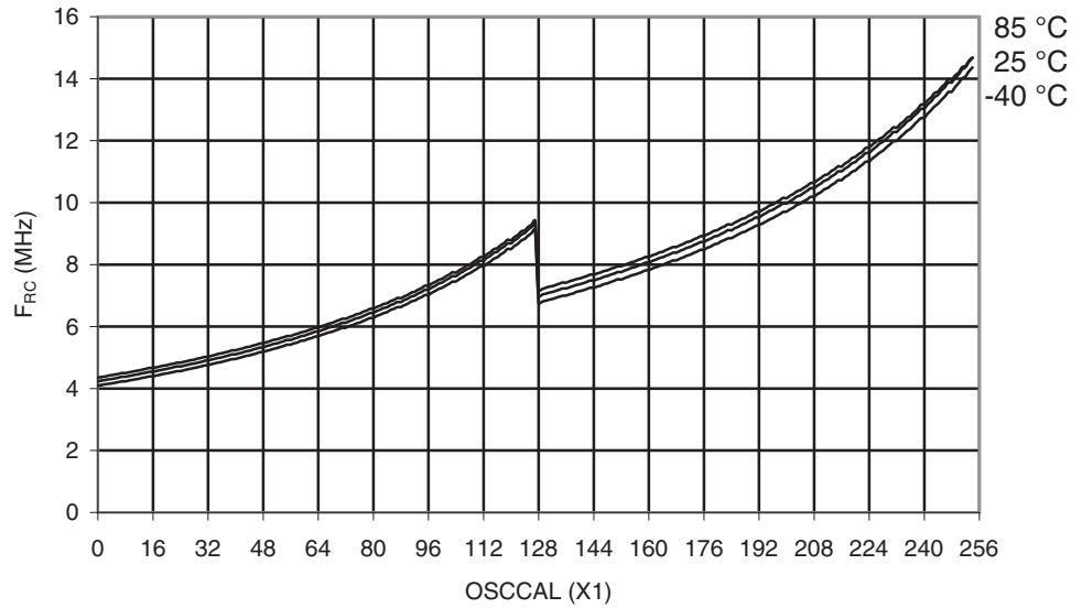
Figure 28-385. ATmega1284P: Calibrated 8 MHz RC Oscillator vs. OSCCAL Value
