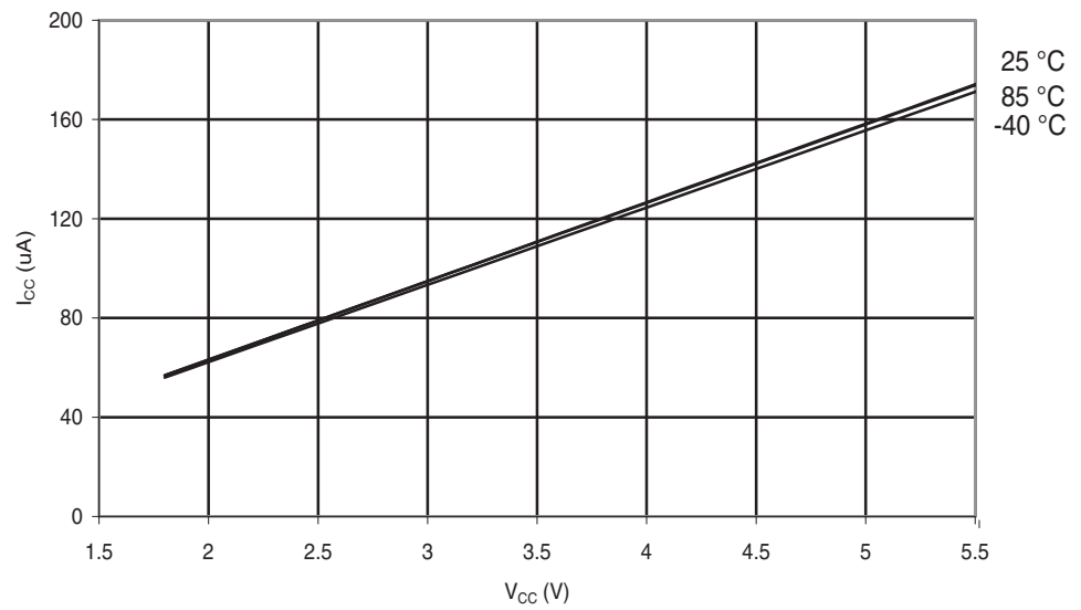
Figure 28-288. ATmega644PA: AREF External Reference Current vs. V_{CC}
