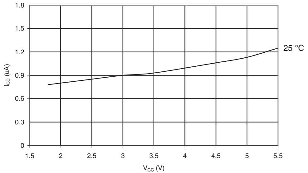
Figure 28-13. ATmega164A: Power-save Supply Current vs. V_{CC} (Watchdog Timer Disabled and 32 kHz Crystal Oscillator Running).
