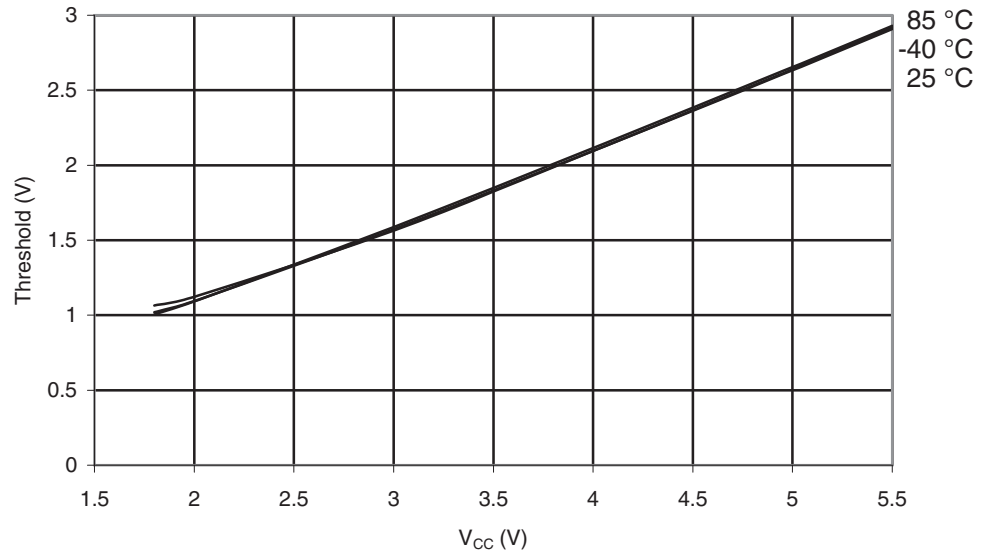
Figure 28-271. ATmega644PA: I/O Pin Input Threshold vs. V_{CC} ( V_{IL} , I/O Pin Read as '0').
