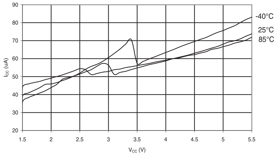
Figure 28-238. ATmega644A: Analog Comparator Current vs. V_{CC}
