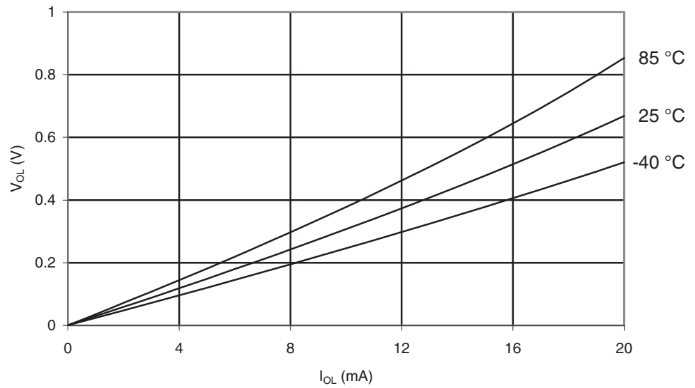
Figure 28-70. ATmega164PA: I/O Pin Output Voltage vs. Sink Current ( V_{CC} = 3V ).
