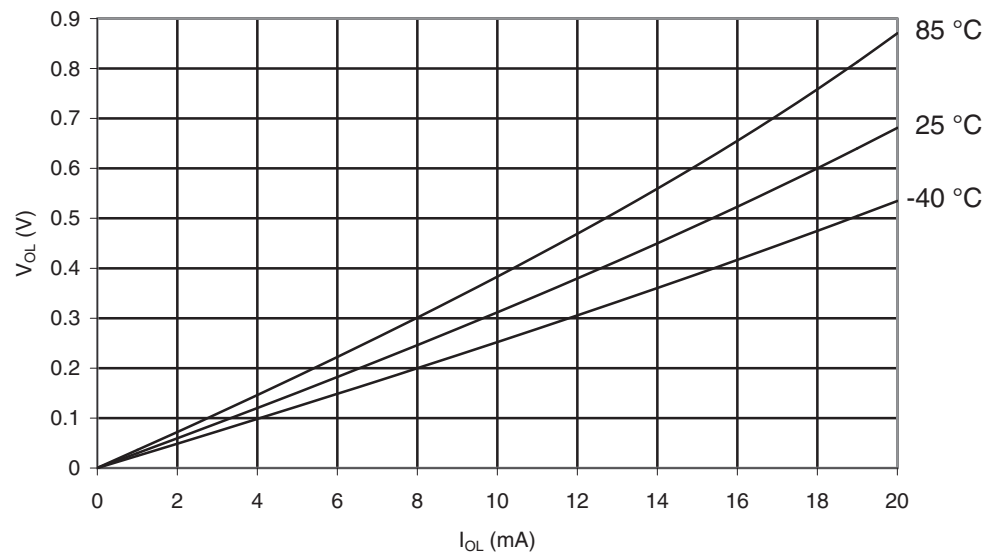
Figure 28-316. ATmega1284: I/O Pin Output Voltage vs. Sink Current ( V_{CC} = 3V )
