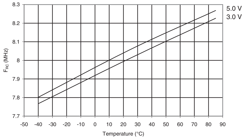
Figure 28-88. ATmega164PA: Calibrated 8 MHz RC Oscillator vs. Temperature
