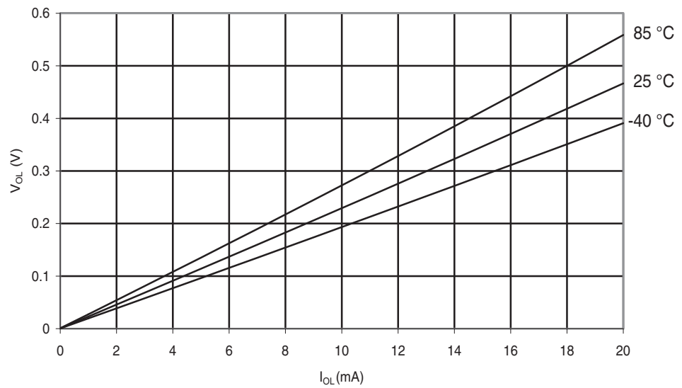
Figure 28-218. ATmega644A: I/O Pin Output Voltage vs. Sink Current ( V_{CC} = 5V ).
