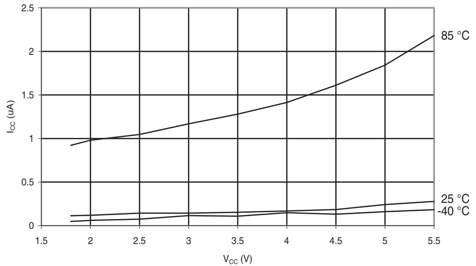
Figure 28-207. ATmega644A: Power-down Supply Current vs. V_{CC} (Watchdog Timer Disabled)
