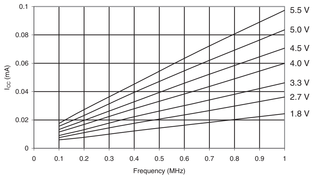
Figure 28-392. ATmega1284P: Reset Supply Current vs. Low Frequency (0.1 - 1.0 MHz)
