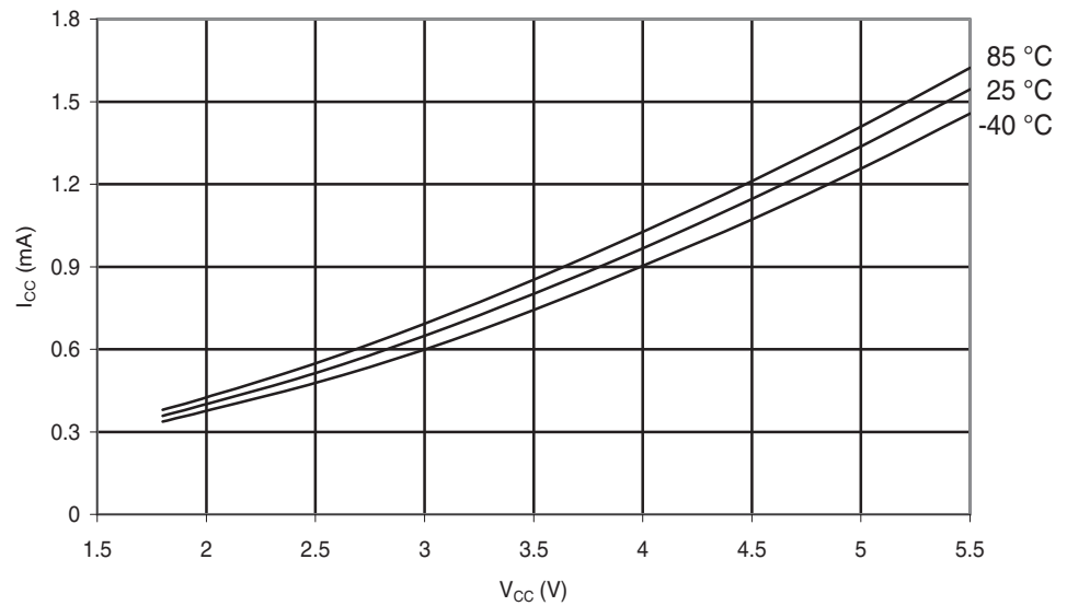
Figure 28-155. ATmega324PA: Idle Supply Current vs. V_{CC} (Internal RC Oscillator, 8 MHz).
