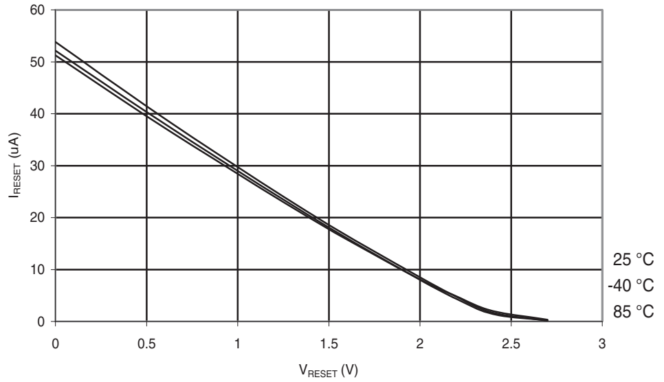
Figure 28-117. ATmega324A: Reset Pull-up Resistor Current vs. Reset Pin Voltage ( V_{CC} = 2.7V ).
