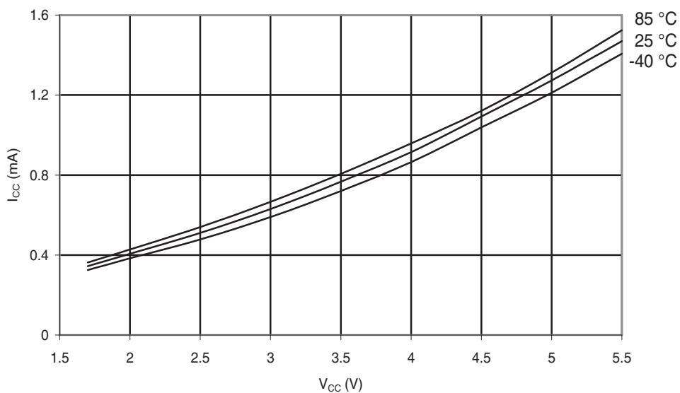
Figure 28-151. ATmega324PA: Active Supply Current vs. V_{CC} (Internal RC Oscillator, 1 MHz).
