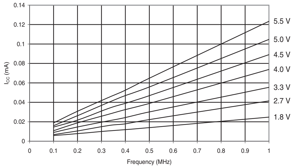
Figure 28-194. ATmega324PA: Reset Supply Current vs. Low Frequency (0.1 - 1.0 MHz)
