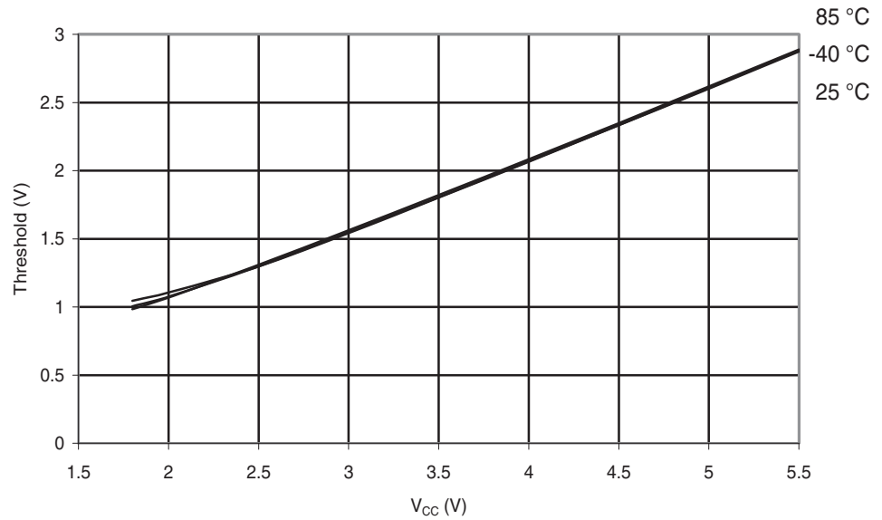
Figure 28-172. ATmega324PA: I/O Pin Input Threshold vs. V_{CC} ( V_{IH} , I/O Pin Read as '1').
