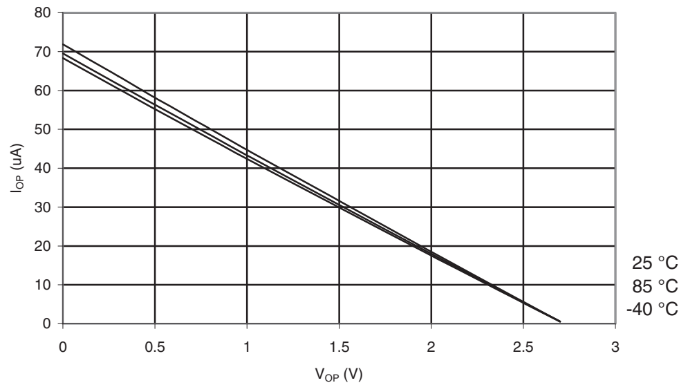
Figure 28-16. ATmega164A: I/O Pin Pull-up Resistor Current vs. Input Voltage ( V_{CC} = 2.7V ).
