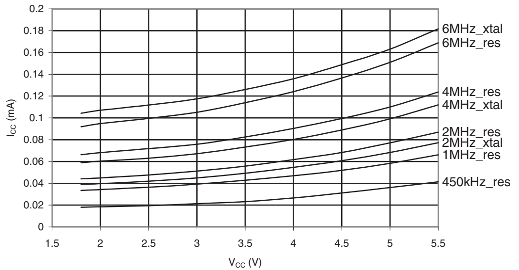
Figure 28-63. ATmega164PA: Standby Supply Current vs. V_{CC} (Watchdog Timer Disabled).
