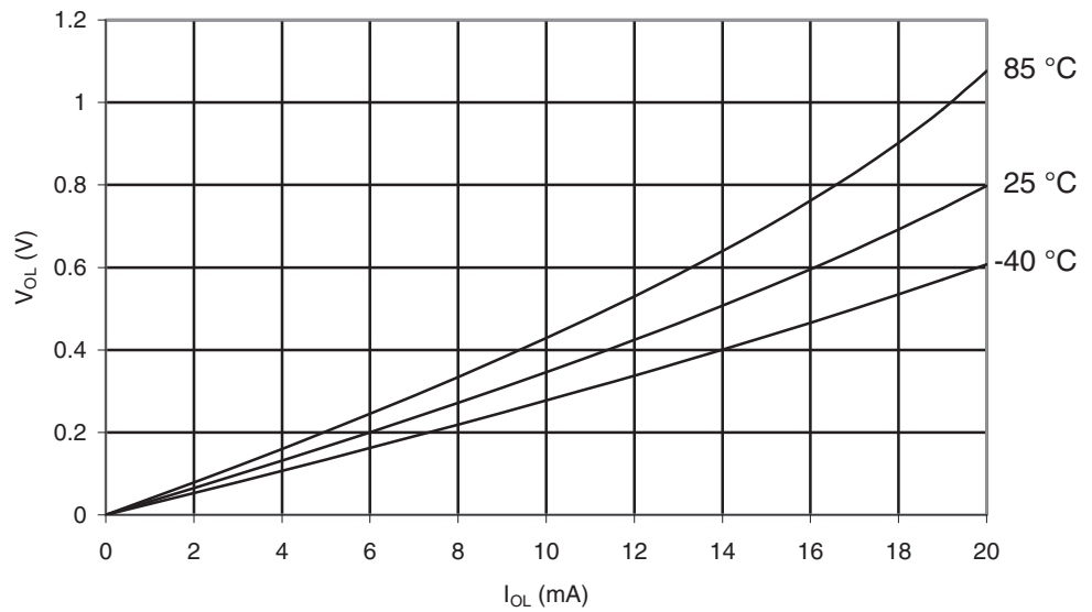
Figure 28-315. ATmega1284: I/O Pin Output Voltage vs. Sink Current ( V_{CC} = 2.7V )
