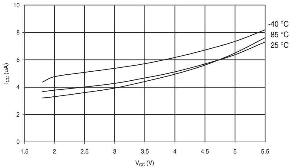
Figure 28-159. ATmega324PA: Power-down Supply Current vs. V_{CC} (Watchdog Timer Enabled).
