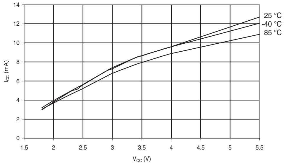
Figure 28-192. ATmega324PA: Programming Current vs. V_{CC}
