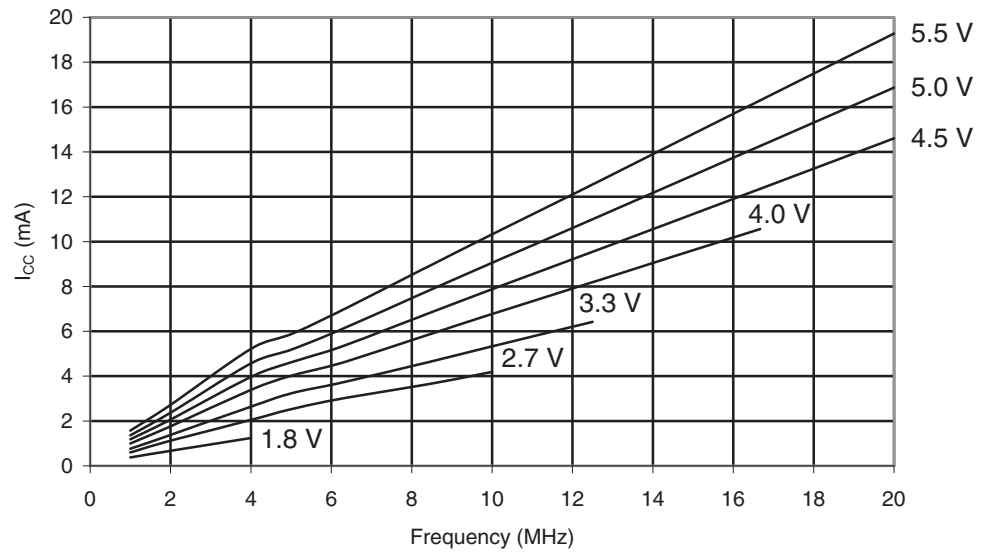
Figure 28-346. ATmega1284P: Active Supply Current vs. Frequency (1 - 20 MHz)
