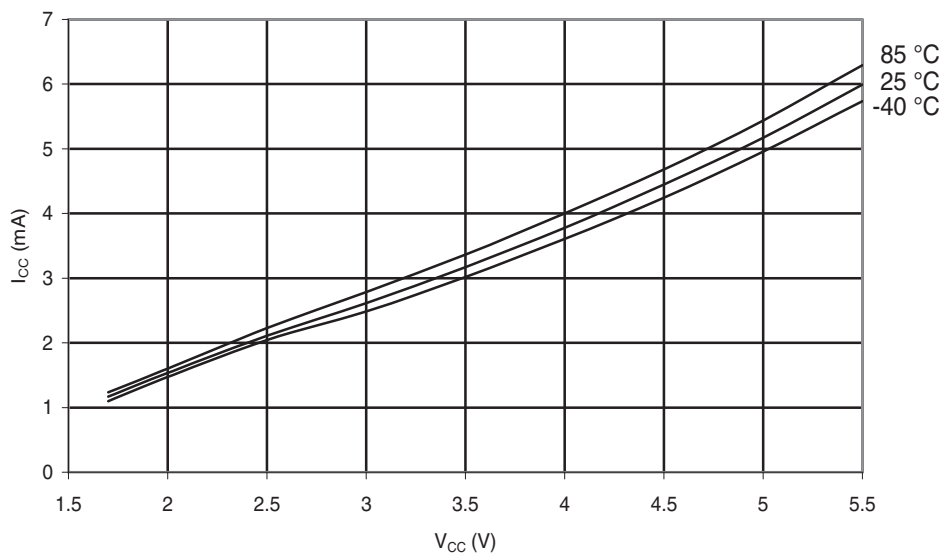
Figure 28-150. ATmega324PA: Active Supply Current vs. V_{CC} (Internal RC Oscillator, 8 MHz).
