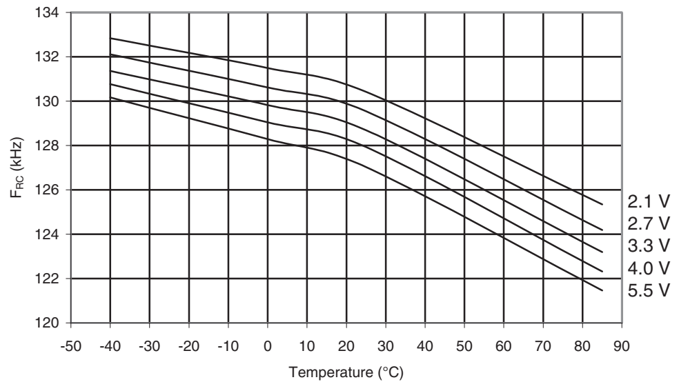
Figure 28-85. ATmega164PA: Watchdog Oscillator Frequency vs. Temperature
