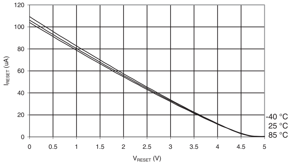
Figure 28-314. ATmega1284: Reset Pull-up Resistor Current vs. Reset Pin Voltage ( V_{CC} = 5V )
