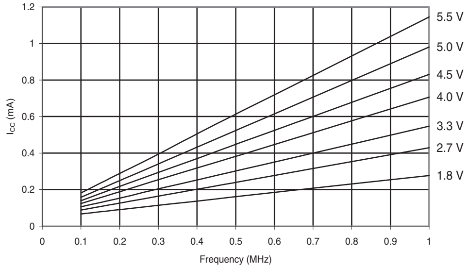
Figure 28-148. ATmega324PA: Active Supply Current vs. Low Frequency (0.1 - 1.0 MHz).
