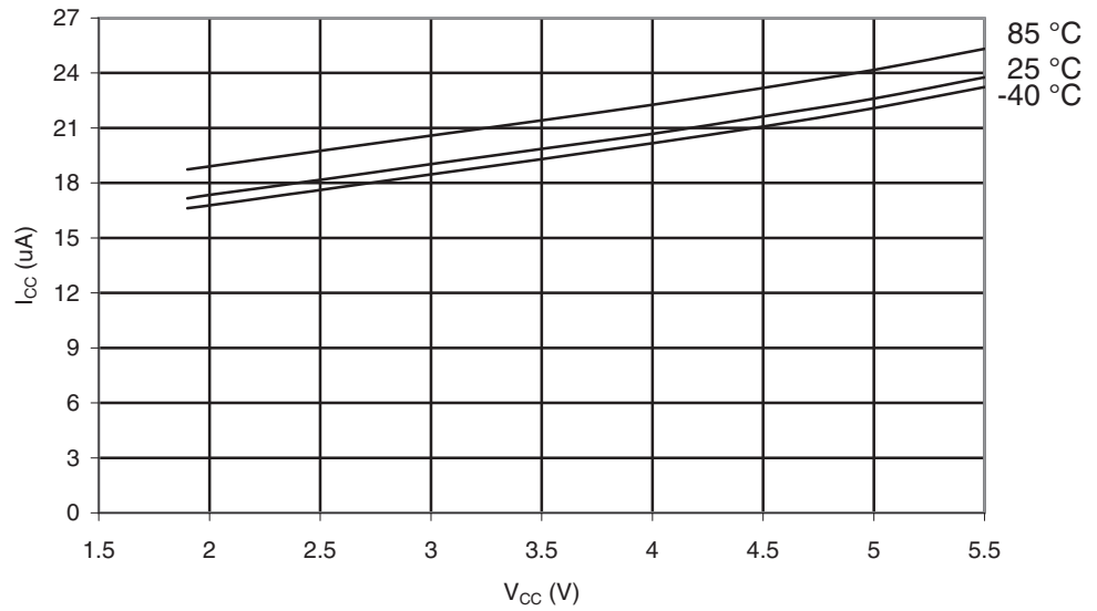
Figure 28-44. ATmega164A: Brownout Detector Current vs. V_{CC}
