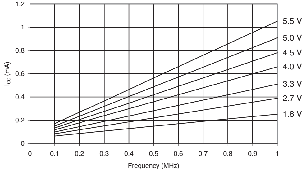
Figure 28-50. ATmega164PA: Active Supply Current vs. Low Frequency (0.1 - 1.0 MHz).
