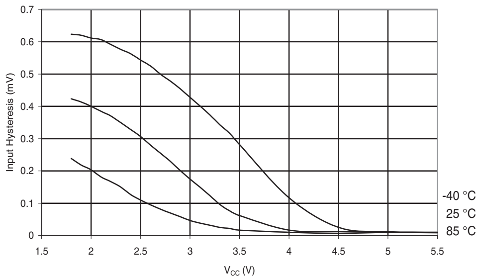
Figure 28-177. ATmega324PA: Reset Pin Input Hysteresis vs. V_{CC}
