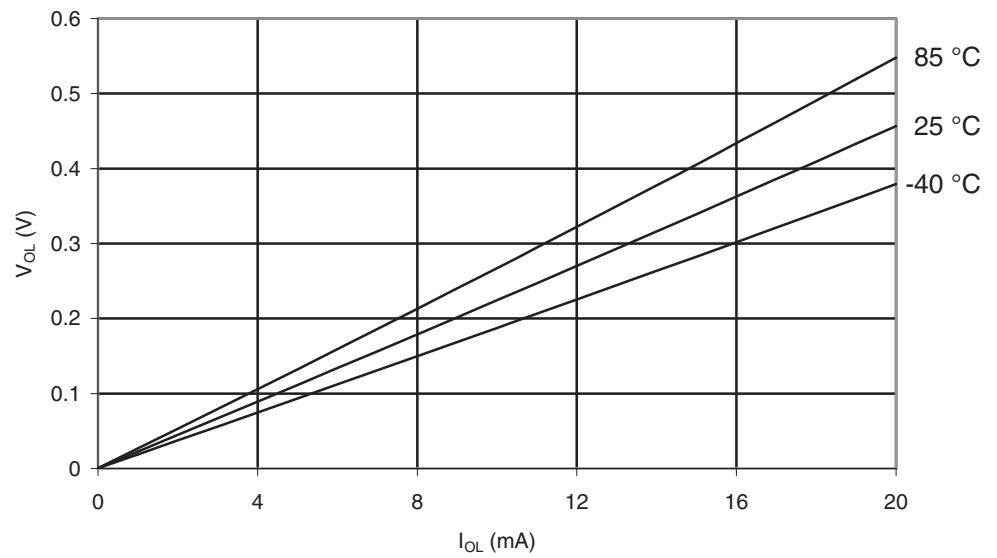
Figure 28-22. ATmega164A: I/O Pin Output Voltage vs. Sink Current ( V_{CC} = 5V ).
