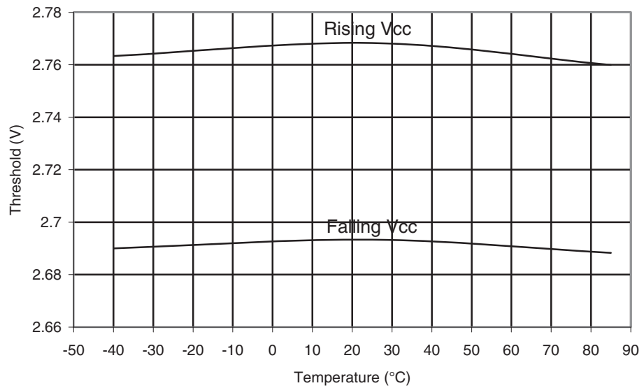
Figure 28-81. ATmega164PA: BOD Threshold vs. Temperature ( V_{BOT} = 2.7V )
