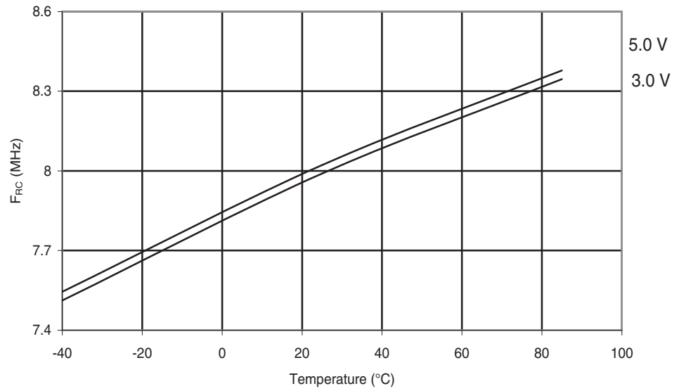
Figure 28-137. ATmega324A: Calibrated 8 MHz RC Oscillator vs. Temperature
