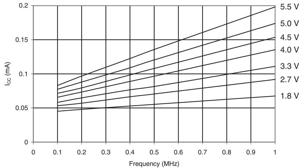
Figure 28-6. ATmega164A: Idle Supply Current vs. V_{CC} (0.1 - 1.0 MHz).
