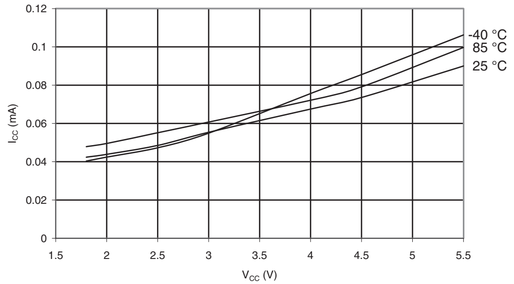
Figure 28-304. ATmega1284: Idle Supply Current vs. V_{CC} (Internal RC Oscillator, 128 kHz)
