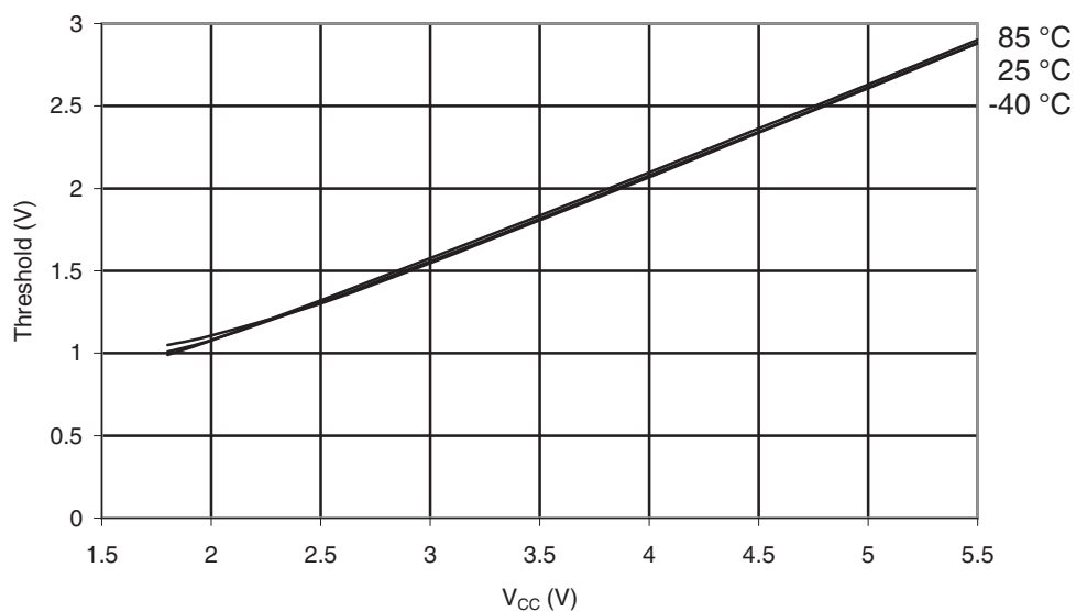
Figure 28-25. ATmega164A: I/O Pin Input Threshold vs. V_{CC} ( V_{IH} , I/O Pin Read as '1').
