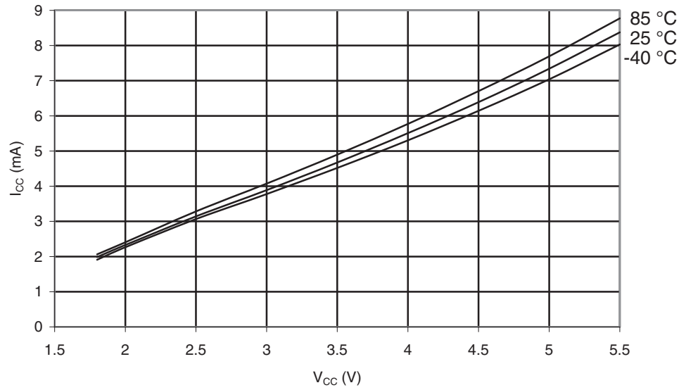
Figure 28-298. ATmega1284: Active Supply Current vs. V_{CC} (Internal RC Oscillator, 1 MHz)
