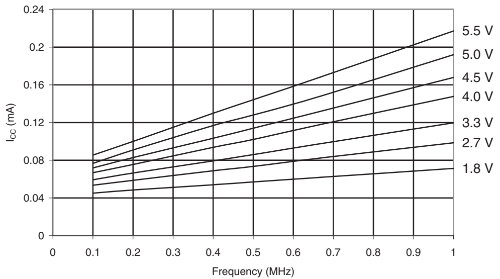
Figure 28-202. ATmega644A: Idle Supply Current vs. V_{CC} (0.1 - 1.0 MHz).
