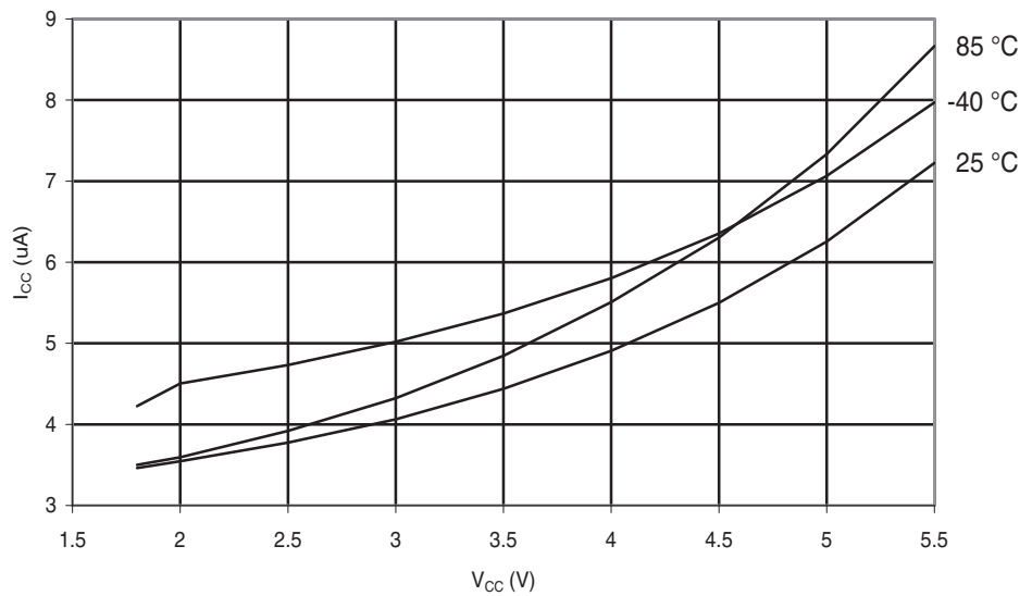
Figure 28-208. ATmega644A: Power-down Supply Current vs. V_{CC} (Watchdog Timer Enabled)
