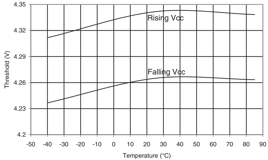
Figure 28-276. ATmega644PA: BOD Threshold vs. Temperature ( V_{BOT} = 4.3V )
