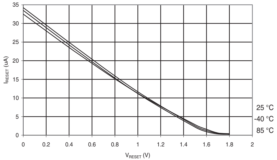
Figure 28-165. ATmega324PA: Reset Pull-up Resistor Current vs. Reset Pin Voltage ( V_{CC} = 1.8V ).
