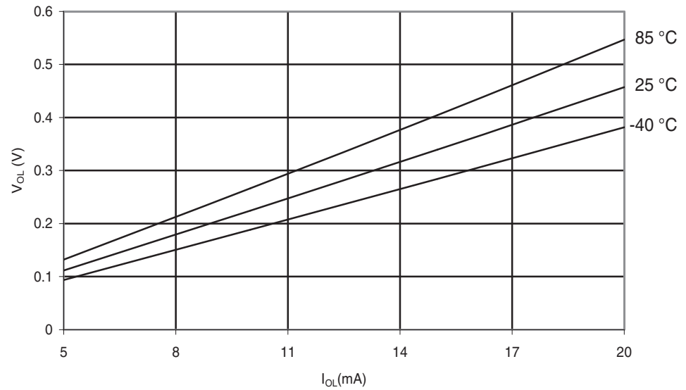
Figure 28-169. ATmega324PA: I/O Pin Output Voltage vs. Sink Current ( V_{CC} = 5V ).
