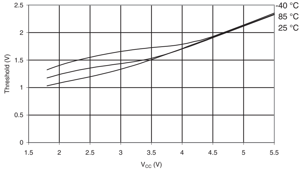
Figure 28-324. ATmega1284: Reset Pin Input Threshold vs. V_{CC} ( V_{IL} , I/O Pin Read as '0')
