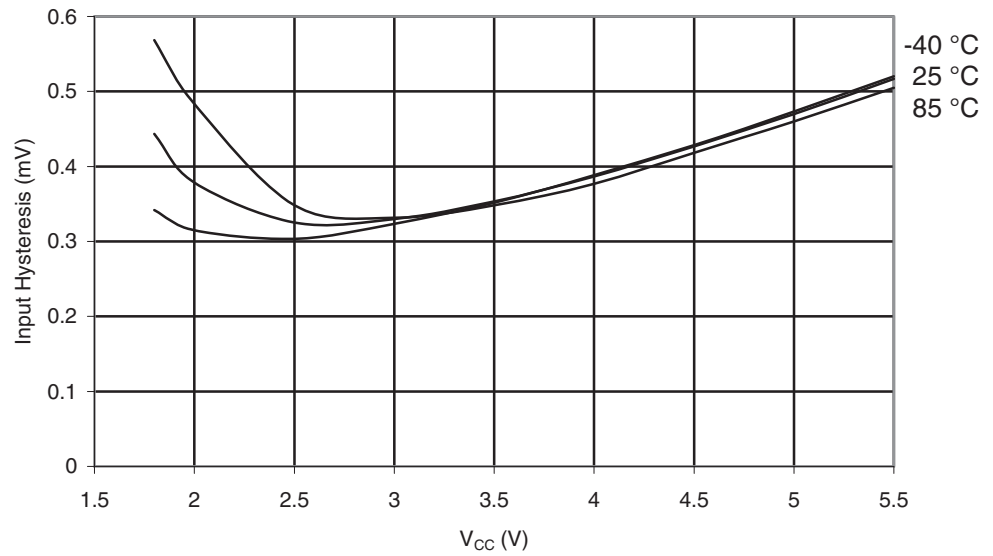
Figure 28-27. ATmega164A: I/O Pin Input Hysteresis vs. V_{CC}
