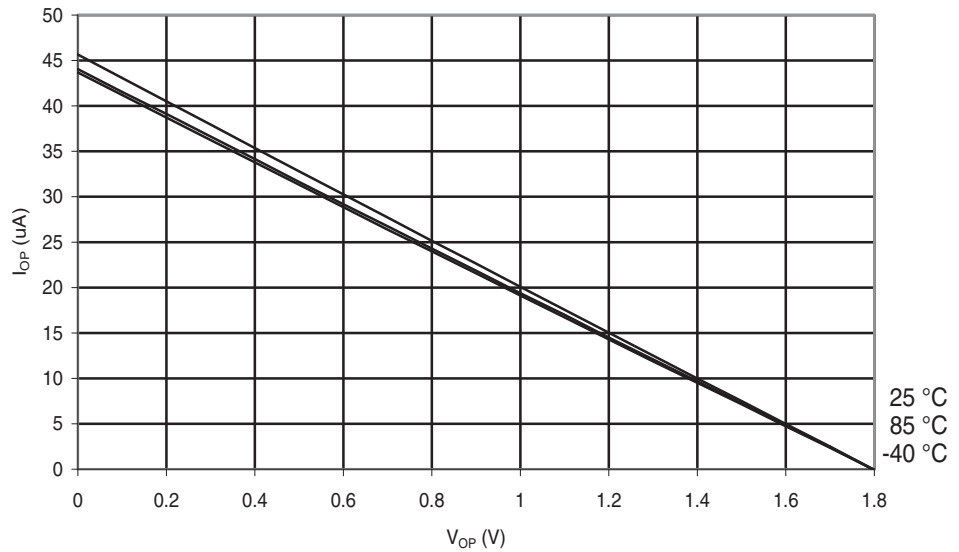
Figure 28-260. ATmega644PA: I/O Pin Pull-up Resistor Current vs. Input Voltage ( V_{CC} = 1.8V ).
