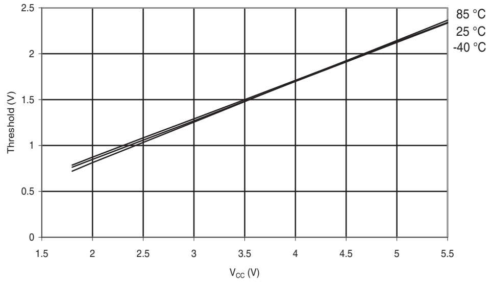
Figure 28-225. ATmega644A: Reset Pin Input Threshold vs. V_{CC} ( V_{IL} , I/O Pin Read as '0').
