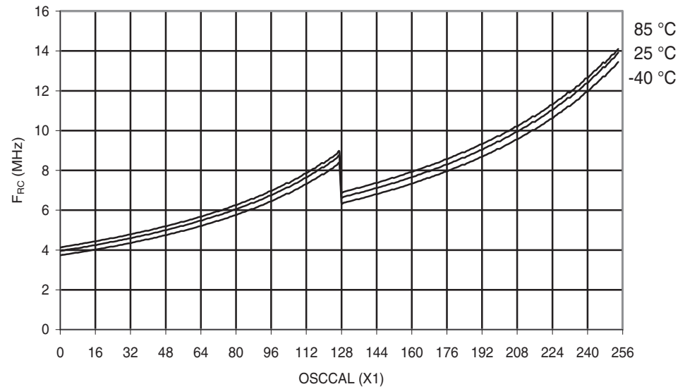
Figure 28-138. ATmega324A: Calibrated 8 MHz RC Oscillator vs. OSCCAL Value
