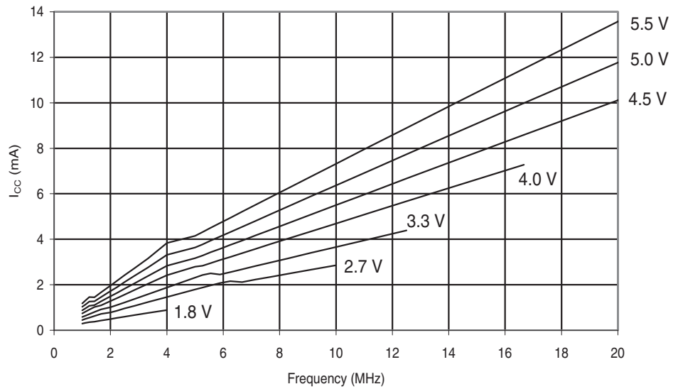
Figure 28-198. ATmega644A: Active Supply Current vs. Frequency (1 - 20 MHz).
