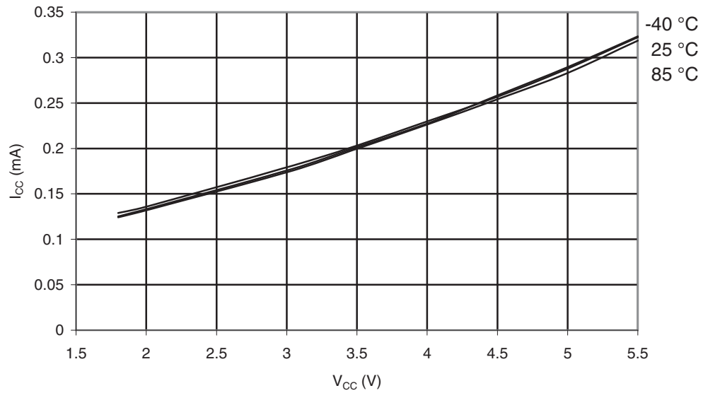
Figure 28-58. ATmega164PA: Idle Supply Current vs. V_{CC} (Internal RC Oscillator, 1 MHz).
