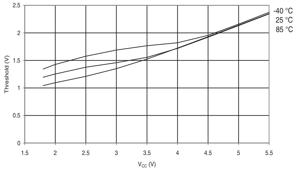
Figure 28-273. ATmega644PA: Reset Pin Input Threshold vs. V_{CC} ( V_{IH} , I/O Pin Read as '1').
