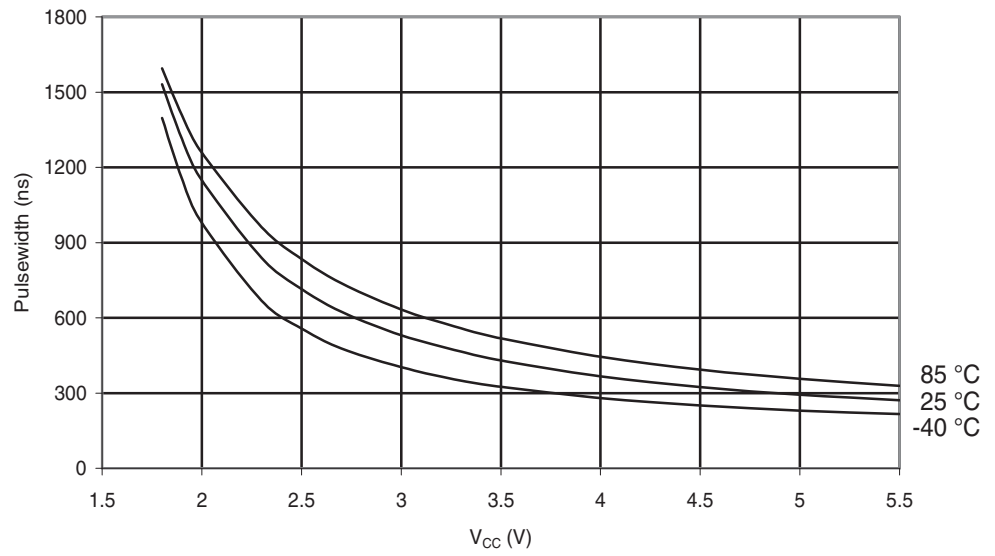
Figure 28-196. ATmega324PA: Minimum Reset Pulsewidth vs. V_{CC}
