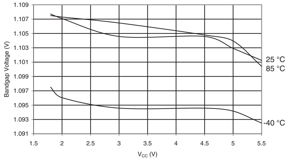
Figure 28-83. ATmega164PA: Calibrated Bandgap Voltage vs. V_{CC}
