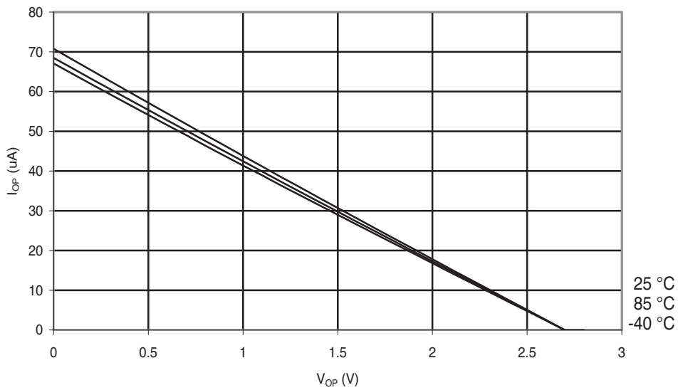
Figure 28-261. ATmega644PA: I/O Pin Pull-up Resistor Current vs. Input Voltage ( V_{CC} = 2.7V ).
