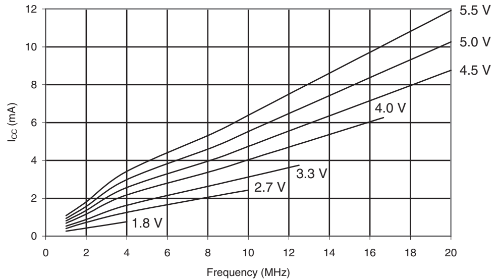
Figure 28-51. ATmega164PA: Active Supply Current vs. Frequency (1 - 20 MHz).
