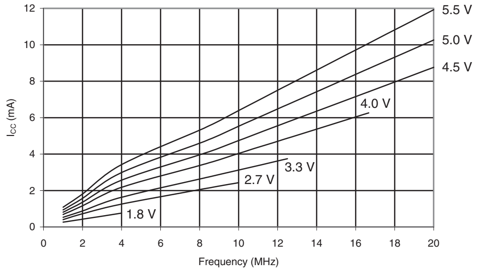
Figure 28-2. ATmega164A: Active Supply Current vs. Frequency (1 - 20 MHz).
