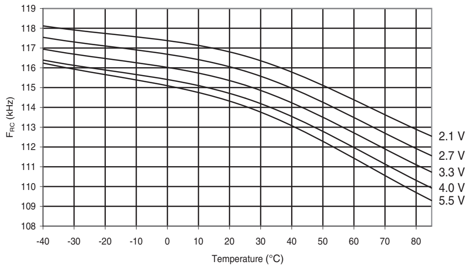
Figure 28-281. ATmega644PA: Watchdog Oscillator Frequency vs. Temperature
