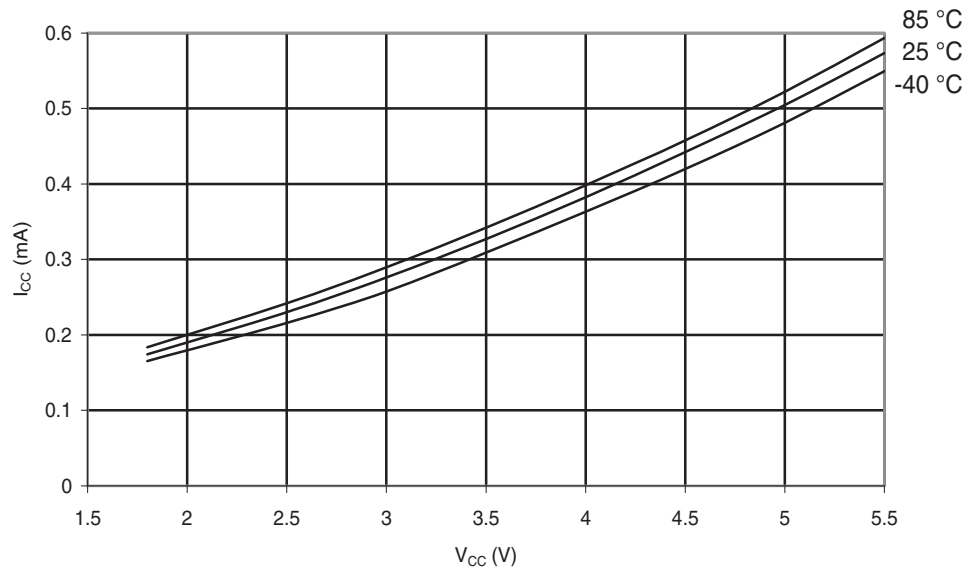
Figure 28-156. ATmega324PA: Idle Supply Current vs. V_{CC} (Internal RC Oscillator, 1 MHz).
