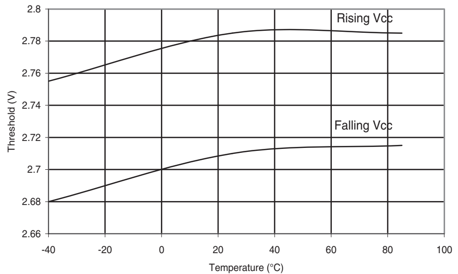
Figure 28-179. ATmega324PA: BOD Threshold vs. Temperature ( V_{BOT} = 2.7V )
