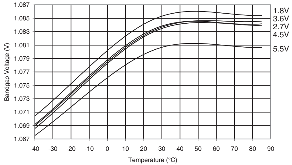
Figure 28-84. ATmega164PA: Bandgap Voltage vs. Temperature
