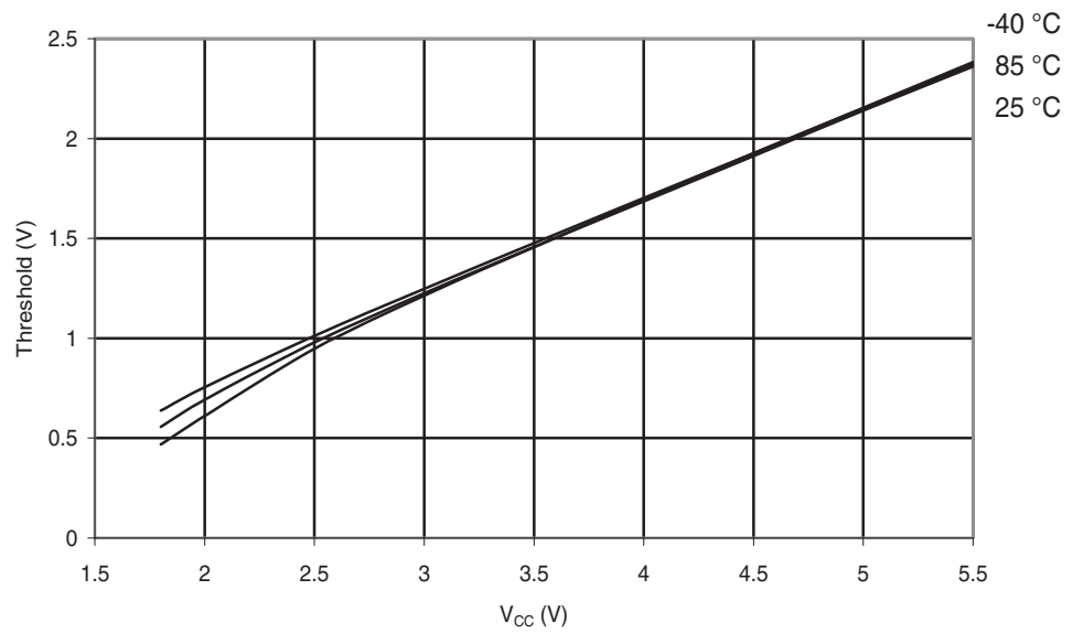
Figure 28-124. ATmega324A: I/O Pin Input Threshold vs. V_{CC} ( V_{IL} , I/O Pin Read as '0').
