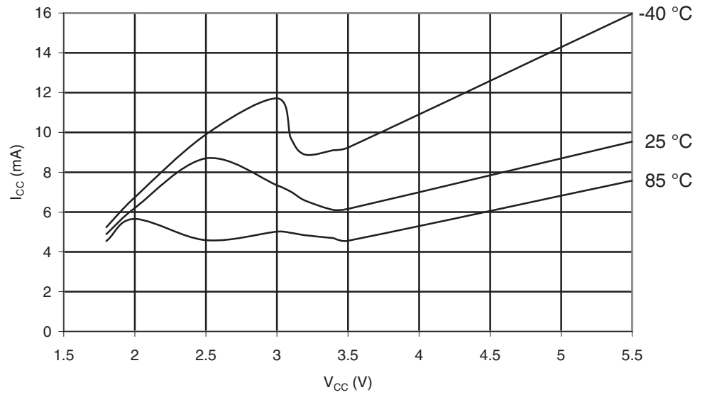
Figure 28-241. ATmega644A: Programming Current vs. V_{CC}
