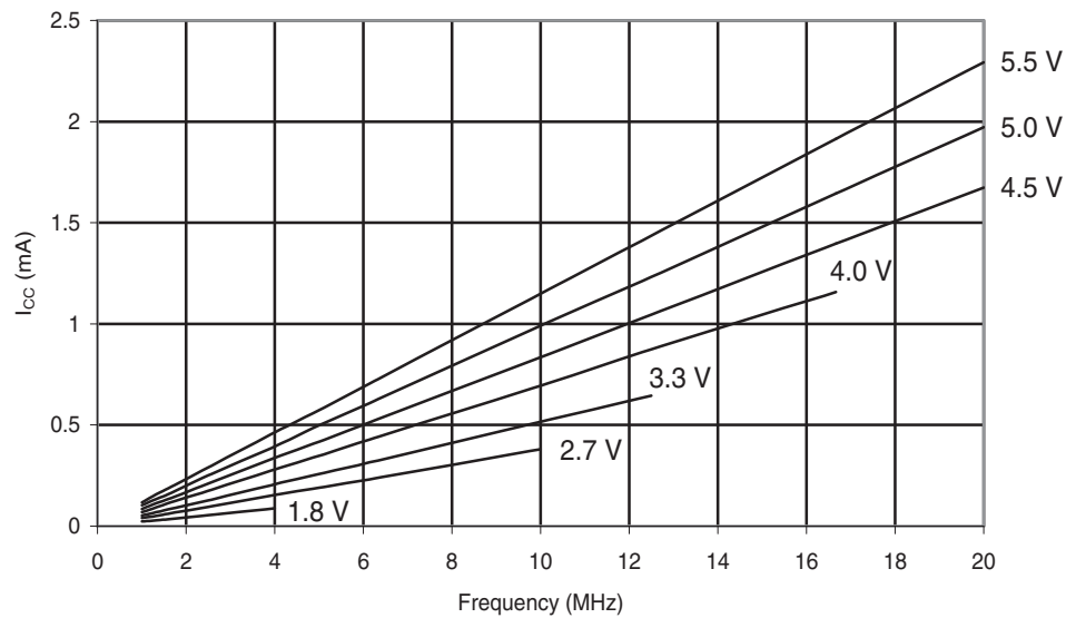
Figure 28-195. ATmega324PA: Reset Supply Current vs. Frequency (1 - 20 MHz)
