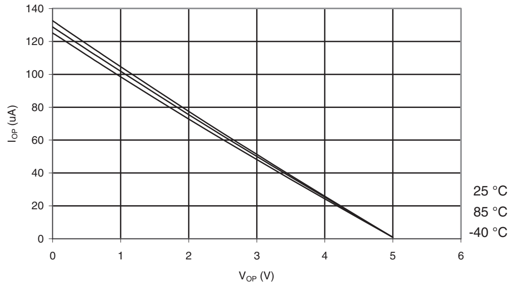
Figure 28-66. ATmega164PA: I/O Pin Pull-up Resistor Current vs. Input Voltage ( V_{CC} = 5V ).
