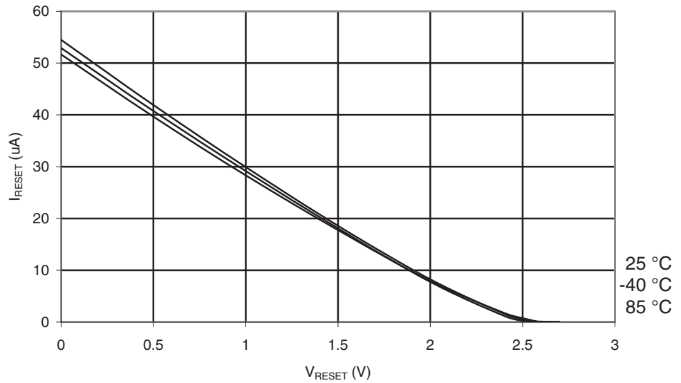
Figure 28-313. ATmega1284: Reset Pull-up Resistor Current vs. Reset Pin Voltage ( V_{CC} = 2.7V )
