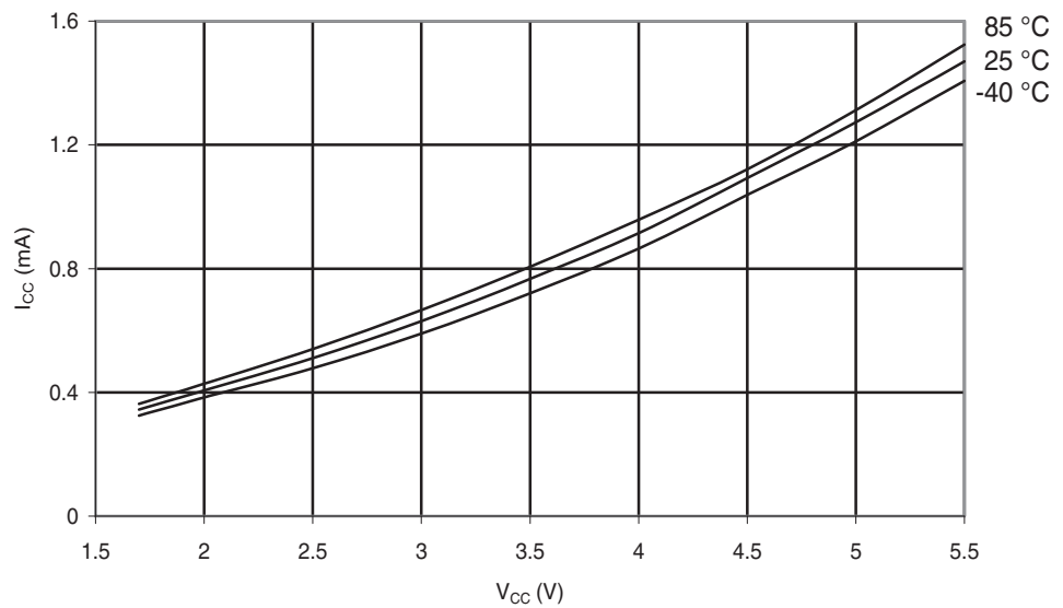
Figure 28-102. ATmega324A: Active Supply Current vs. V_{CC} (Internal RC Oscillator, 1 MHz).
