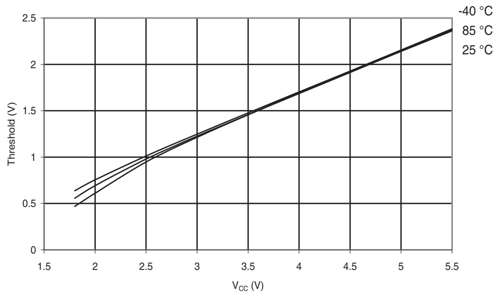
Figure 28-173. ATmega324PA: I/O Pin Input Threshold vs. V_{CC} ( V_{IL} , I/O Pin Read as '0').
