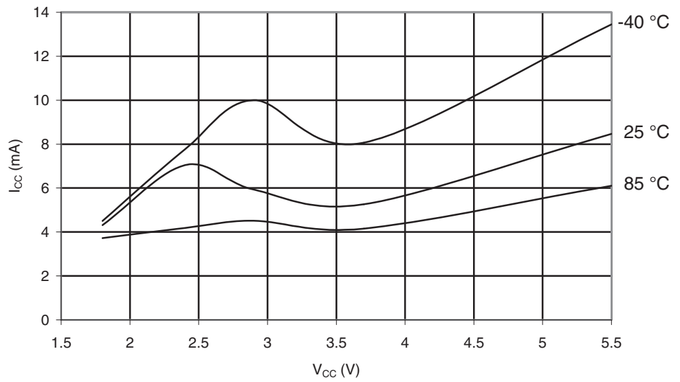
Figure 28-390. ATmega1284P: Programming Current vs. V_{CC}
