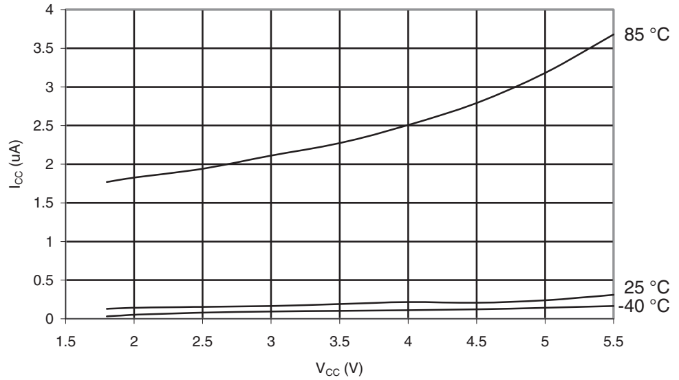
Figure 28-306. ATmega1284: Power-down Supply Current vs. V_{CC} (Watchdog Timer Enabled)
