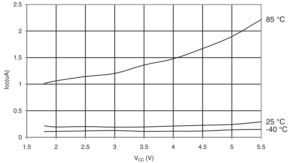
Figure 28-209. ATmega644A: Power-save Supply Current vs. V_{CC} (Watchdog Timer Disabled and 32 kHz Crystal Oscillator Running)
