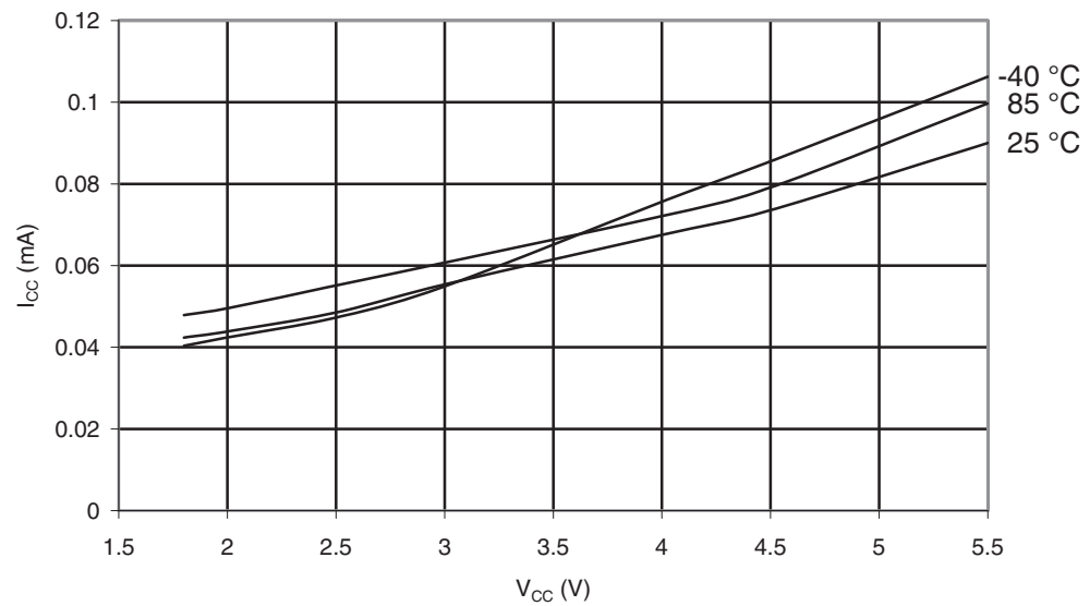
Figure 28-354. ATmega1284P: Idle Supply Current vs. V_{CC} (Internal RC Oscillator, 128 kHz)
