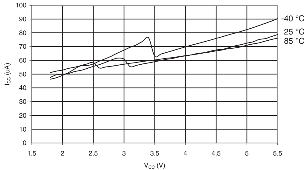
Figure 28-42. ATmega164A: Analog Comparator Current vs. V_{CC}
