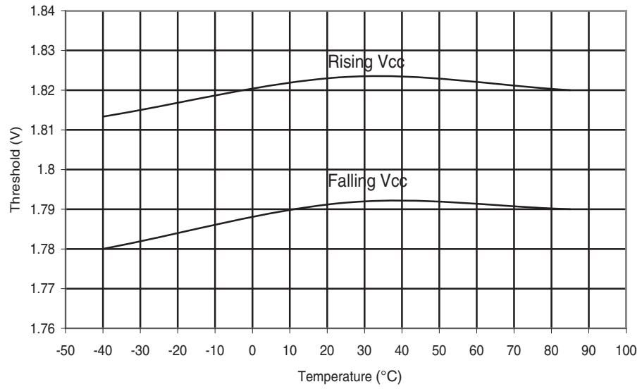
Figure 28-229. ATmega644A: BOD Threshold vs. Temperature ( V_{BOT} = 1.8V )
