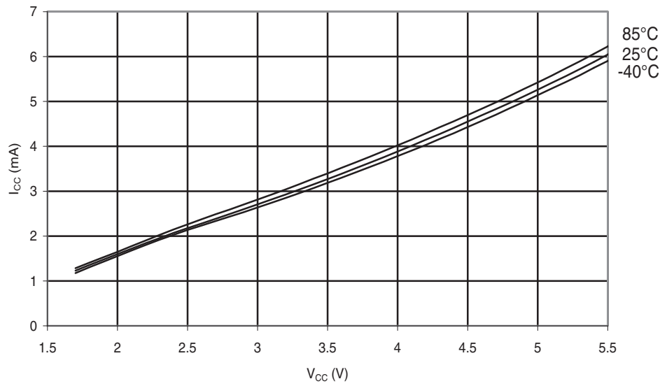
Figure 28-249. ATmega644PA: Active Supply Current vs. V_{CC} (Internal RC Oscillator, 1 MHz).
