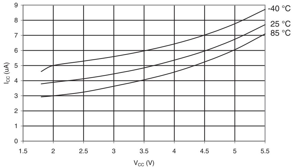
Figure 28-46. ATmega164A: Watchdog Timer Current vs. V_{CC}
