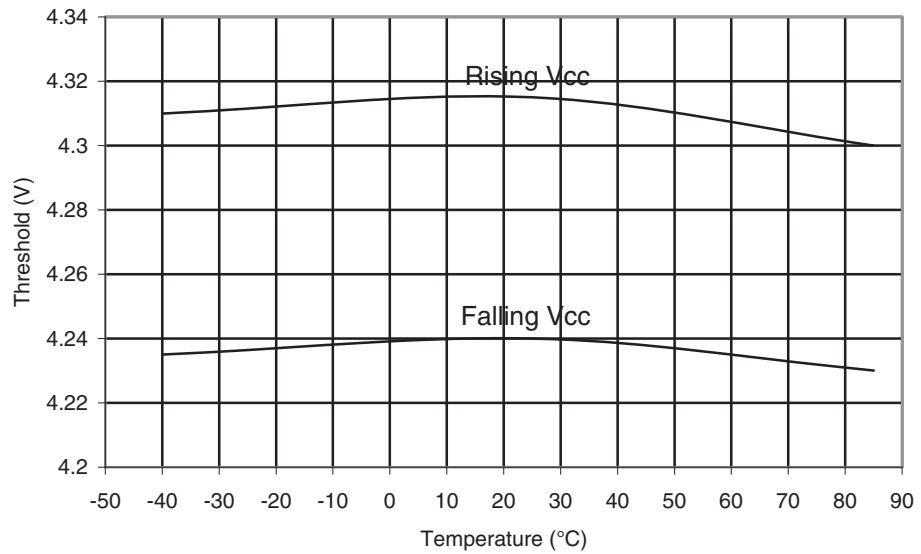
Figure 28-80. ATmega164PA: BOD Threshold vs. Temperature ( V_{BOT} = 4.3V )
