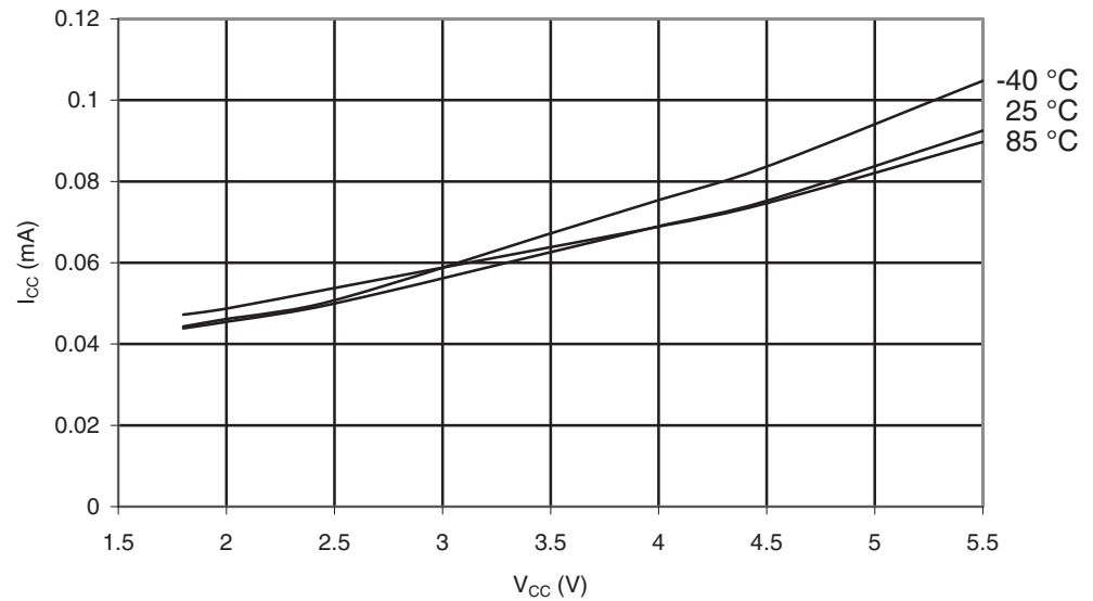
Figure 28-206. ATmega644A: Idle Supply Current vs. V_{CC} (Internal RC Oscillator, 128 kHz).
