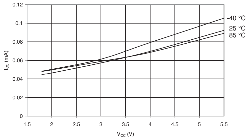
Figure 28-59. ATmega164PA: Idle Supply Current vs. V_{CC} (Internal RC Oscillator, 128 kHz).
