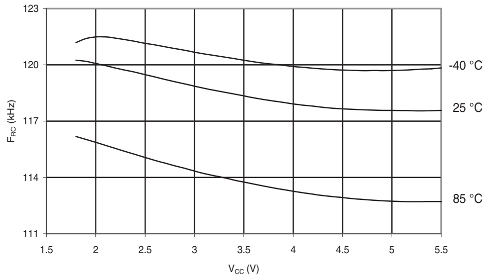
Figure 28-184. ATmega324PA: Watchdog Oscillator Frequency vs. V_{CC}
