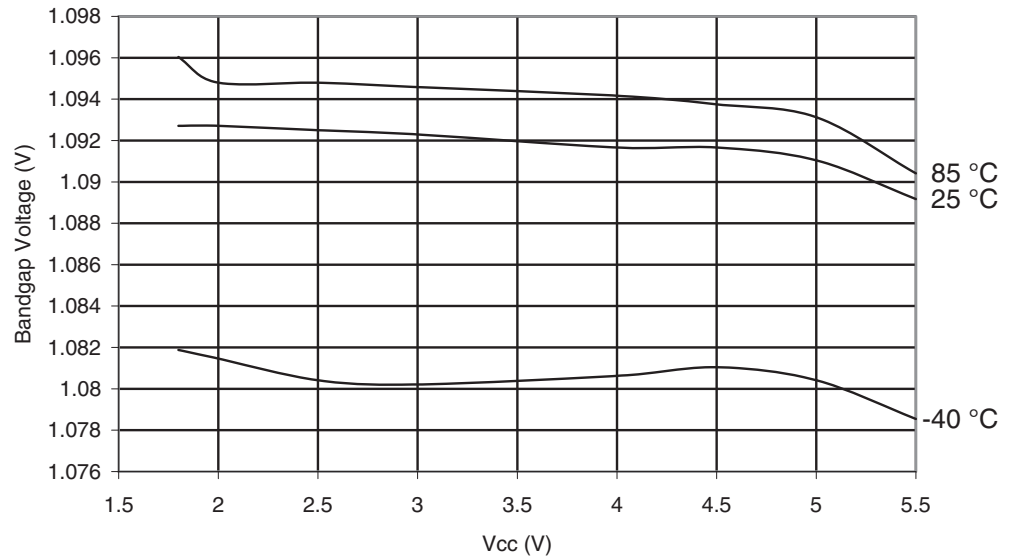
Figure 28-132. ATmega324A: Calibrated Bandgap Voltage vs. V_{CC}
