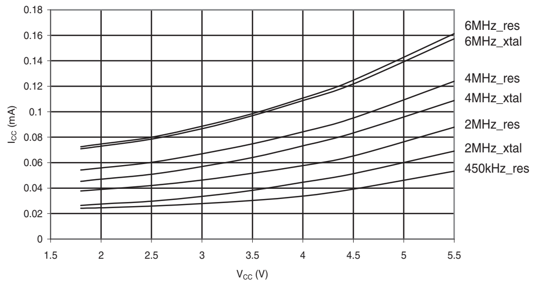
Figure 28-112. ATmega324A: Standby Supply Current vs. V_{CC} (Watchdog Timer Disabled).
