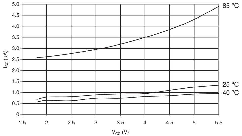
Figure 28-307. ATmega1284: Power-save Supply Current vs. V_{CC} (Watchdog Timer Disabled and 32 kHz Crystal Oscillator Running)
