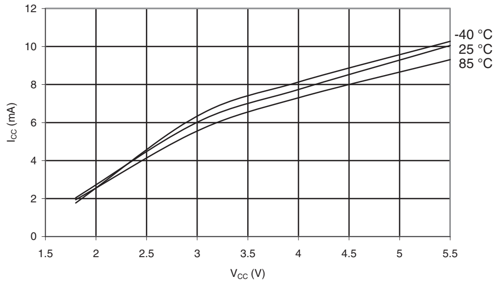
Figure 28-94. ATmega164PA: Programming Current vs. V_{CC}
