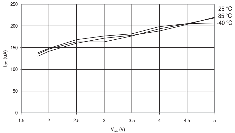
Figure 28-286. ATmega644PA: ADC Current vs. V_{CC} (AREF = AV_{CC} )
