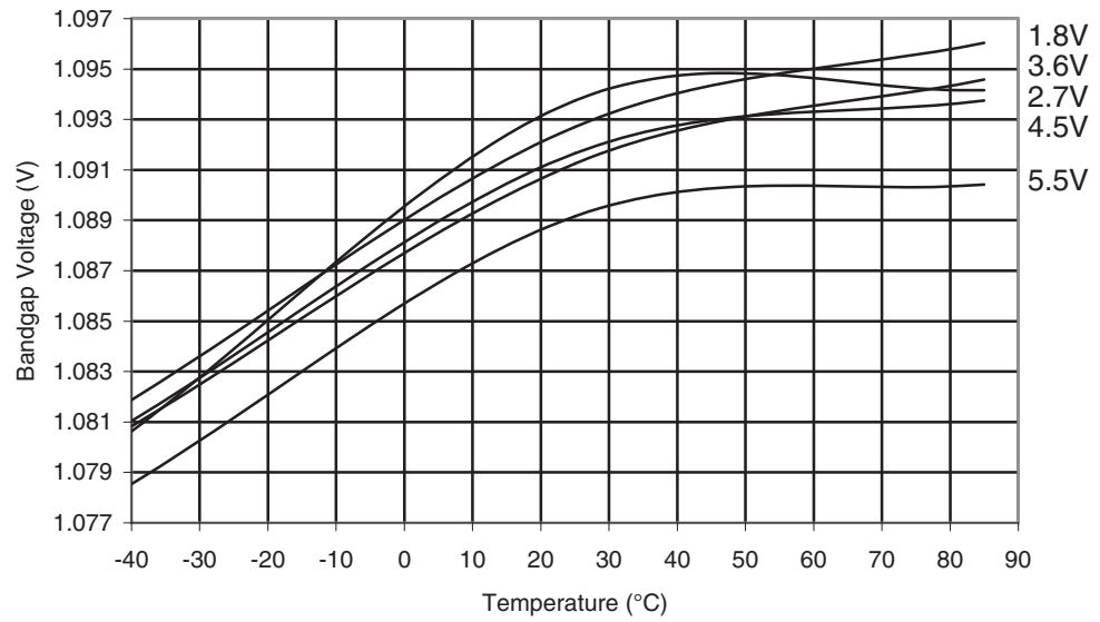
Figure 28-182. ATmega324PA: Bandgap Voltage vs. Temperature
