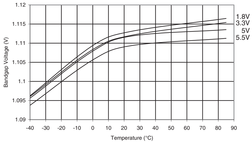
Figure 28-380. ATmega1284P: Bandgap Voltage vs. Temperature
