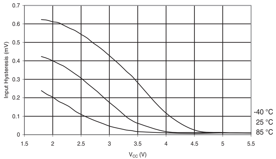
Figure 28-128. ATmega324A: Reset Pin Input Hysteresis vs. V_{CC}
