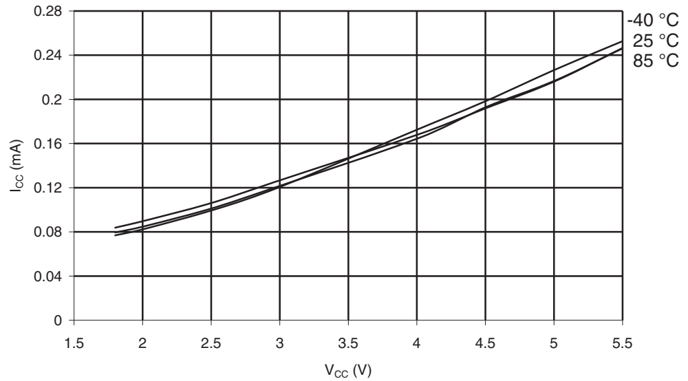
Figure 28-299. ATmega1284: Active Supply Current vs. V_{CC} (Internal RC Oscillator, 128 kHz)
